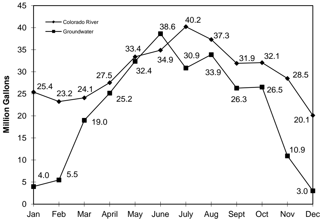
Figure 7. Nellis Air Force Base groundwater and imported Colorado River water usage for 2014.
