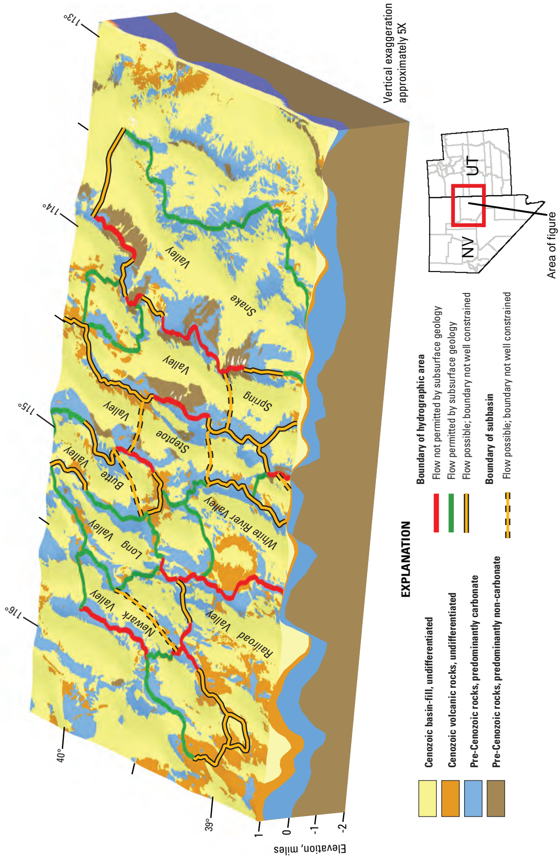
Figure 42. Perspective view of simplified three-dimensional geologic model of the study area.
