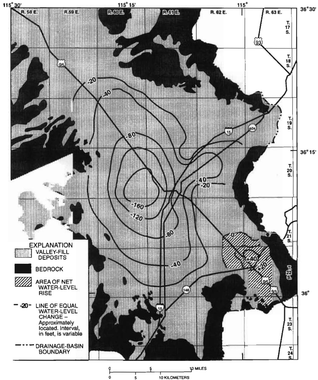
Figure 4.2.2.1-2. Simulated water-level change in developed-zone aquifers, 1912-72.
