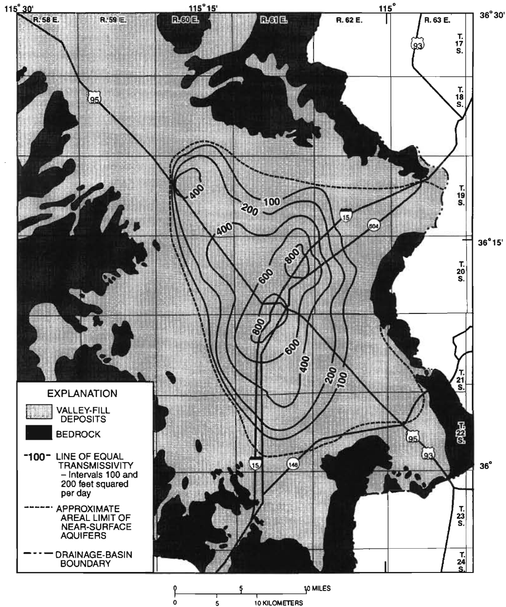
Figure 3.3.1-1. Estimated transmissivity in near-surface aquifers.
