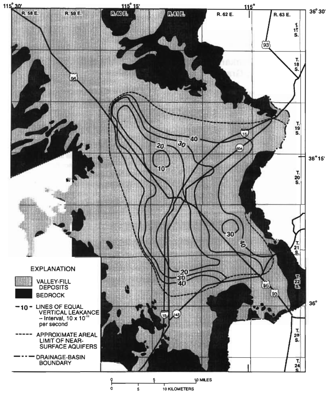
Figure 3.3.2-1. Vertical leakage between near-surface and developed-zone aquifers.
