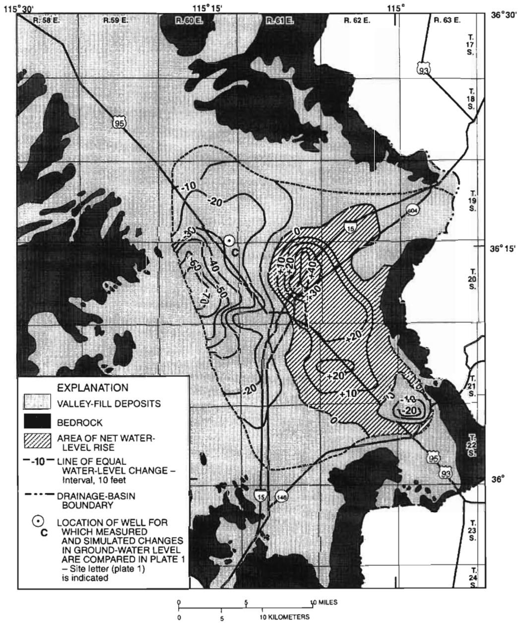
Figure 4.2.3.1-3. Simulated water-level changes in near-surface aquifers, 1972–81.
