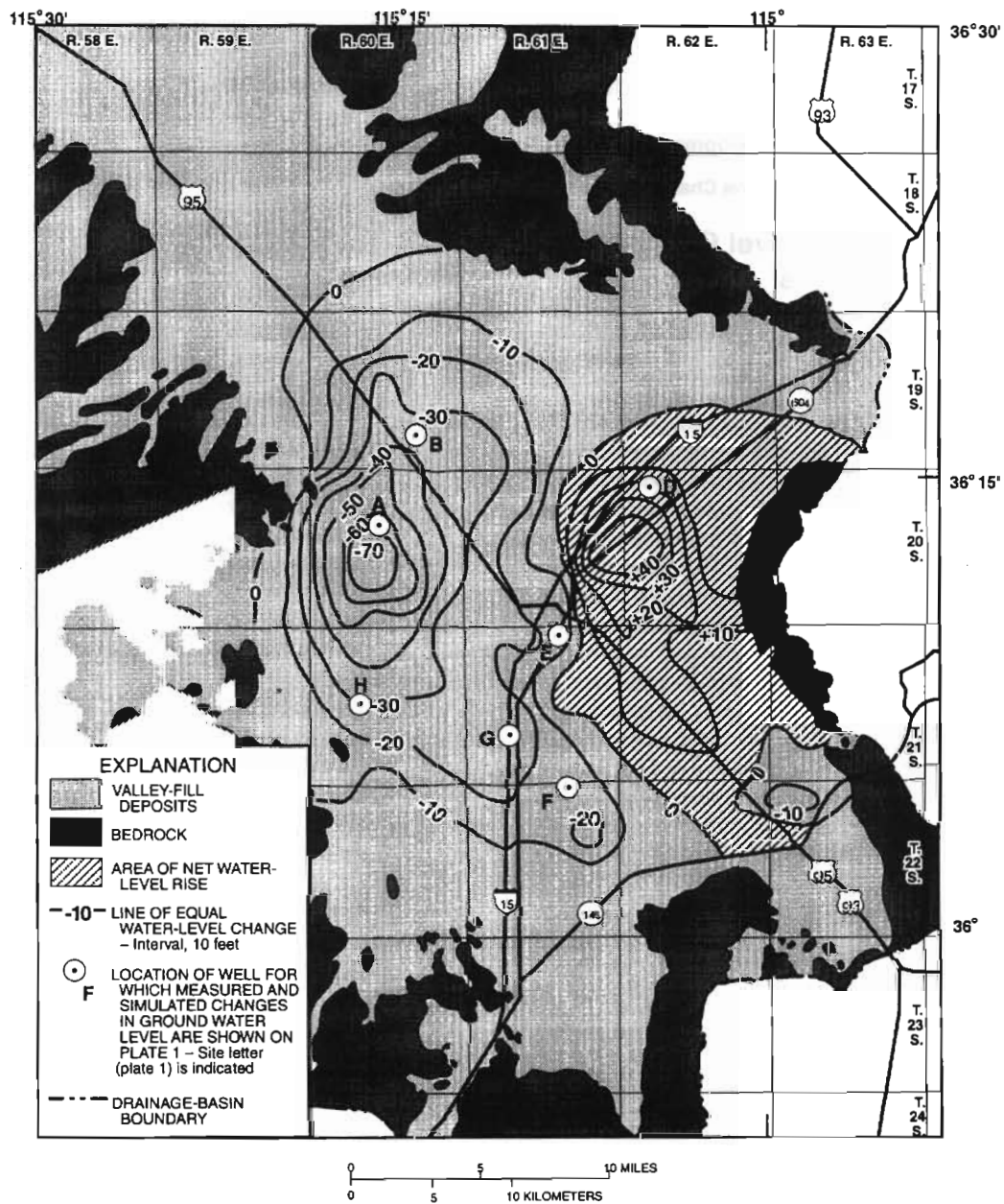
Figure 4.2.3.1-2. Simulated water-level changes in developed-zone aquifers, 1972-81.
