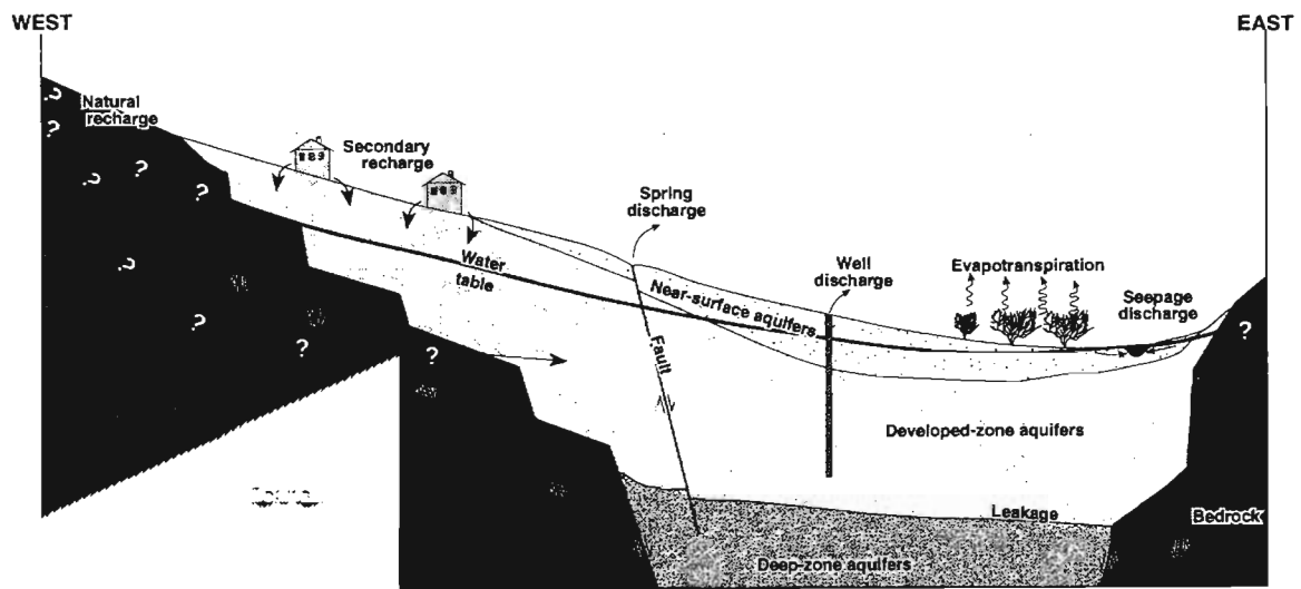
Figure 3.1.1-1. Schematic west-to-east hydrogeologic section.
