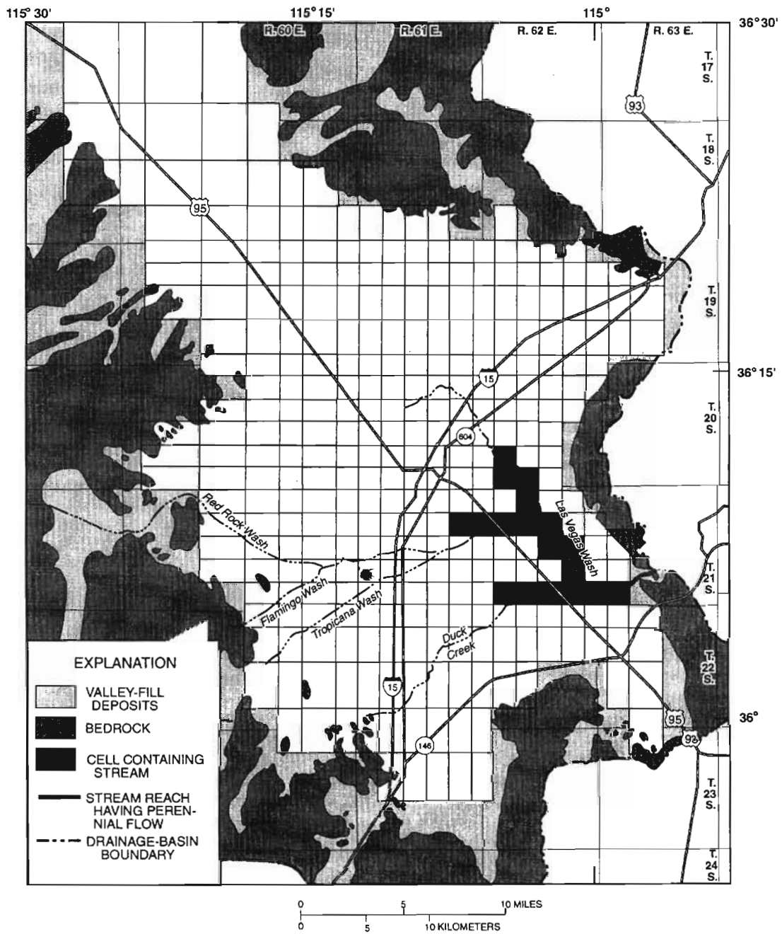
Figure 3.2.3-1. Model grid showing cells containing streams with potential to drain ground water from shallowest parts of near-surface aquifers.
