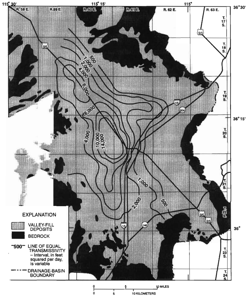
Figure 3.3.1-2. Estimated transmissivity in developed-zone aquifers.
