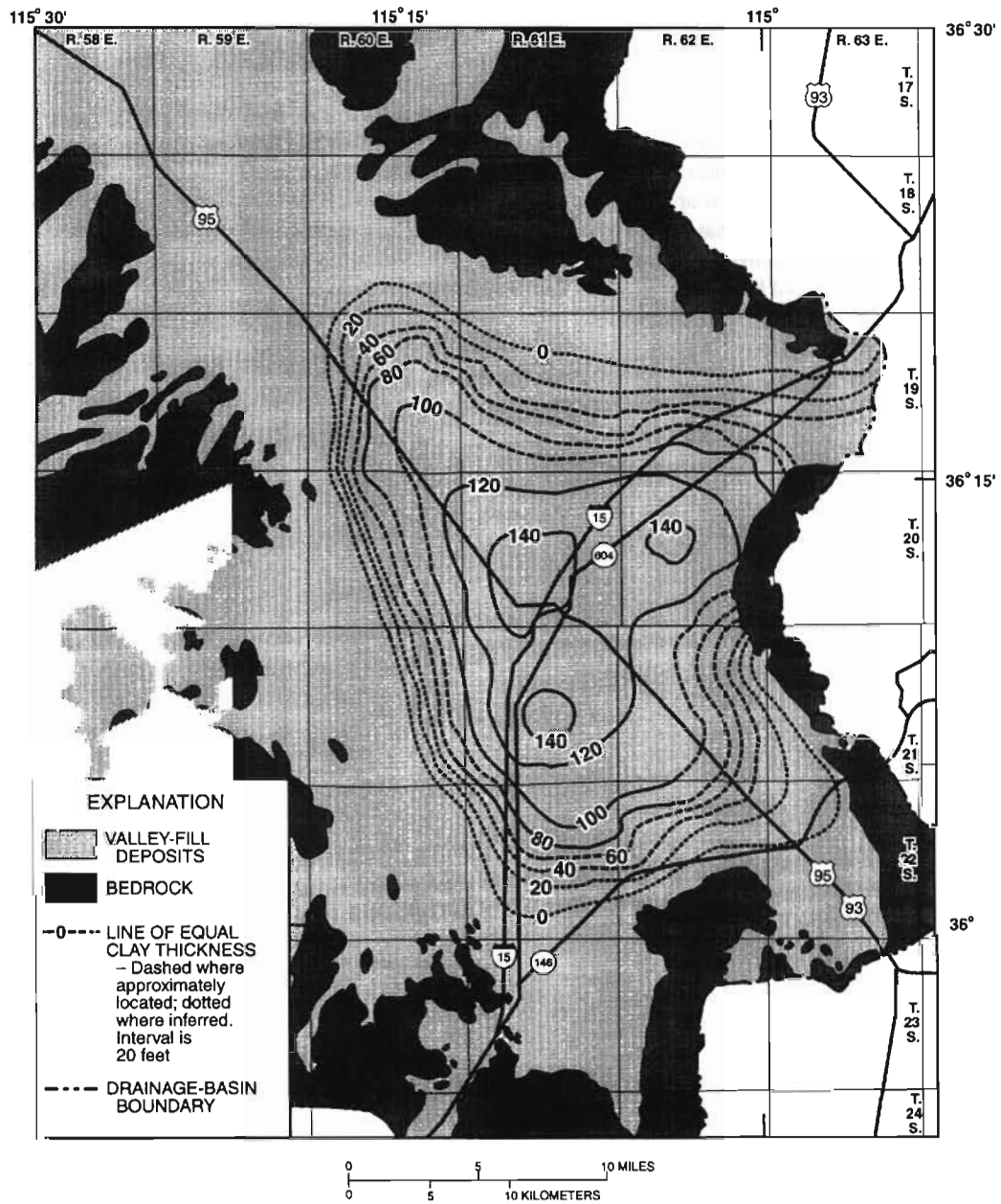
Figure 3.3.4-1. Approximate thickness of clay within near-surface aquifers.
