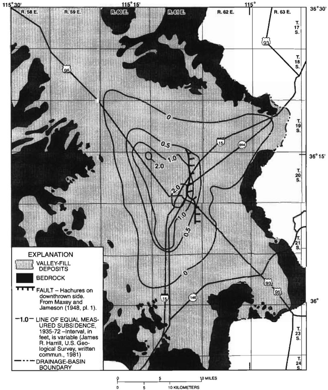
Figure 4.2.2.3-1. Measured land subsidence due to ground-water withdrawals, 1935–72.
