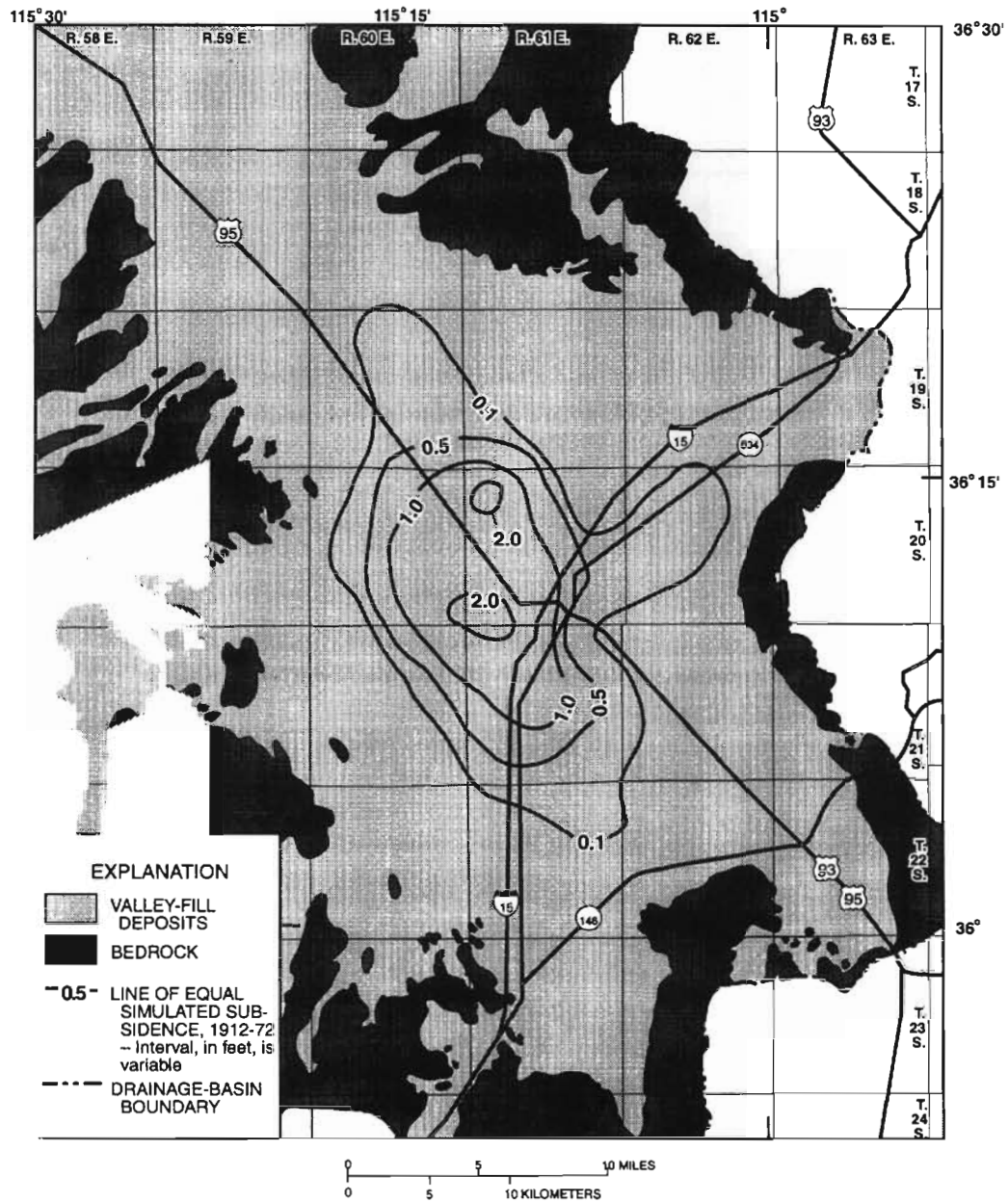
Figure 4.2.2.3-2. Simulated land subsidence due to ground-water withdrawals, 1912–72.
