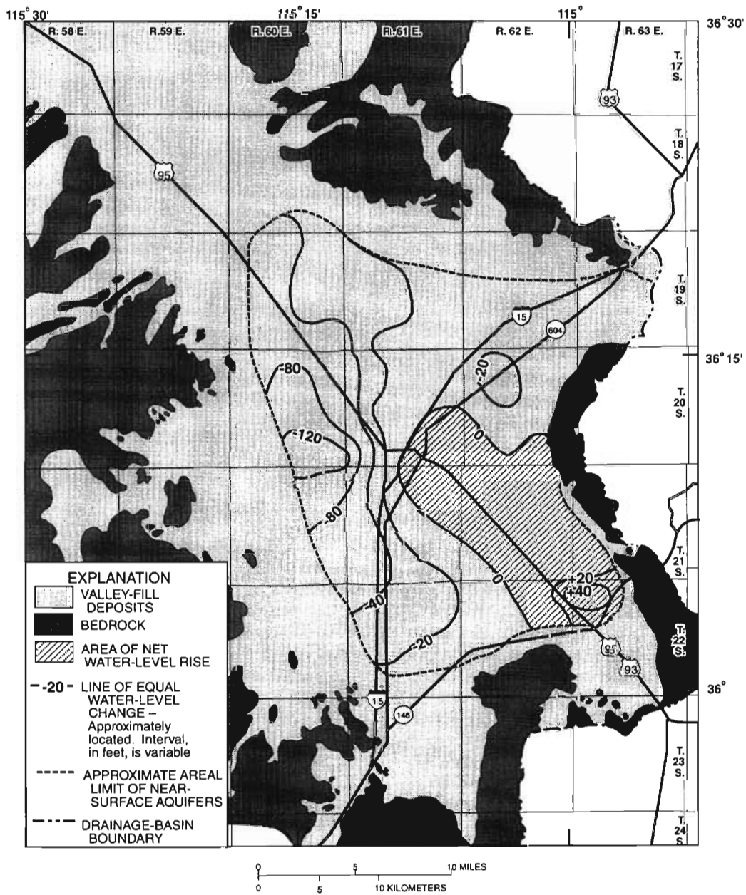
Figure 4.2.2.2-2. Simulated water-level change in near-surface aquifers, 1912–72.
