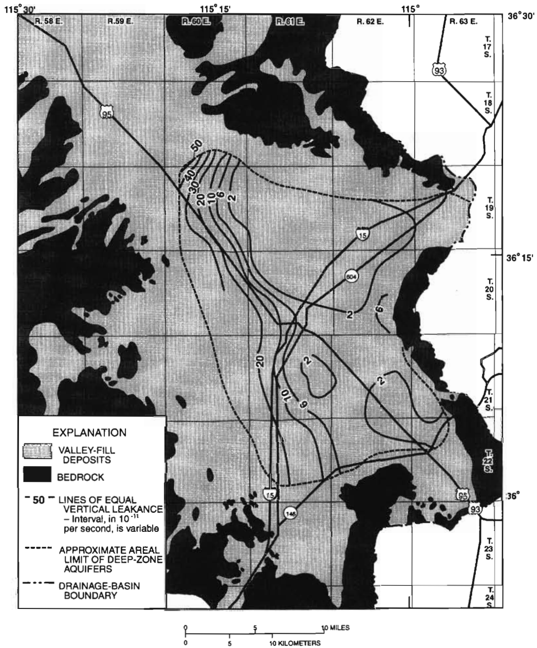
Figure 3.3.2-2. Vertical leakance between developed-zone and deep-zone aquifers.
