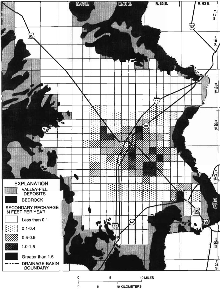
Figure 3.2.5-3. Estimated secondary recharge in 1979.
