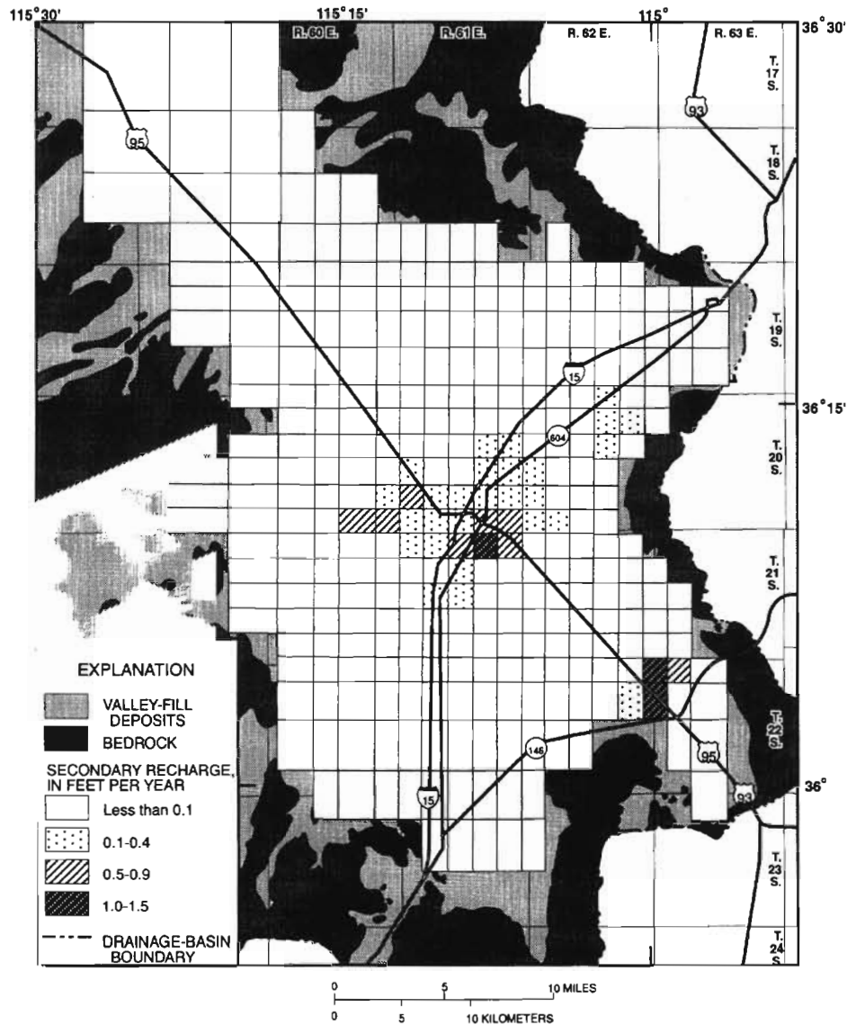
Figure 3.2.5-1. Estimated secondary recharge in 1955.
