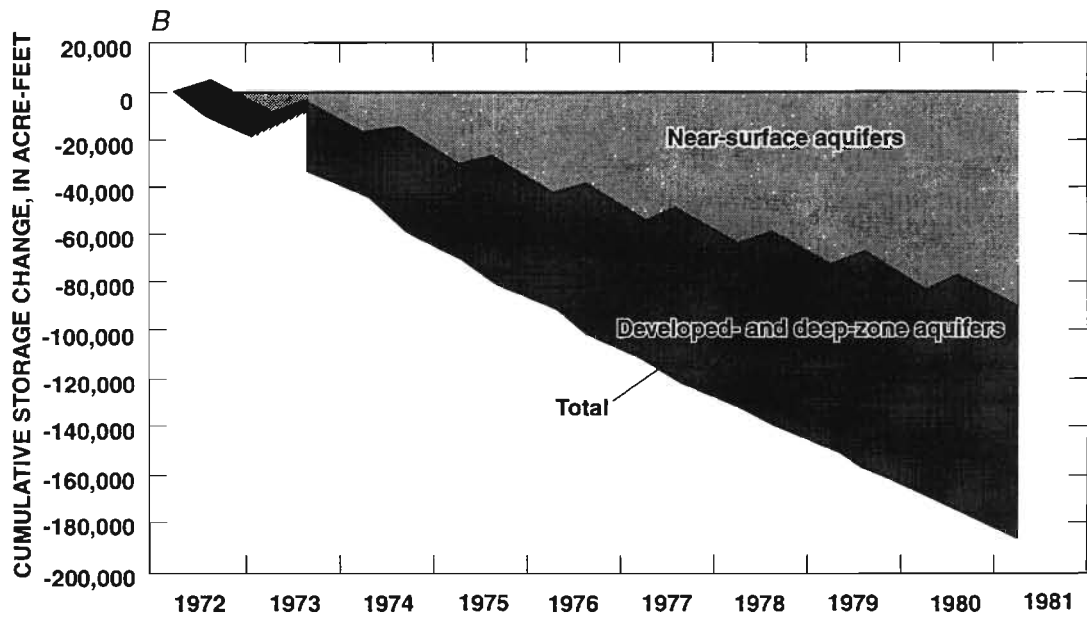
Figure 4.2.3.2-1. Simulated changes in storage, 1972–81. A , Monthly rates; B , cumulative declines. In A , symbols are calculated values; curves are interpolated values. Negative values indicate storage depletion.
