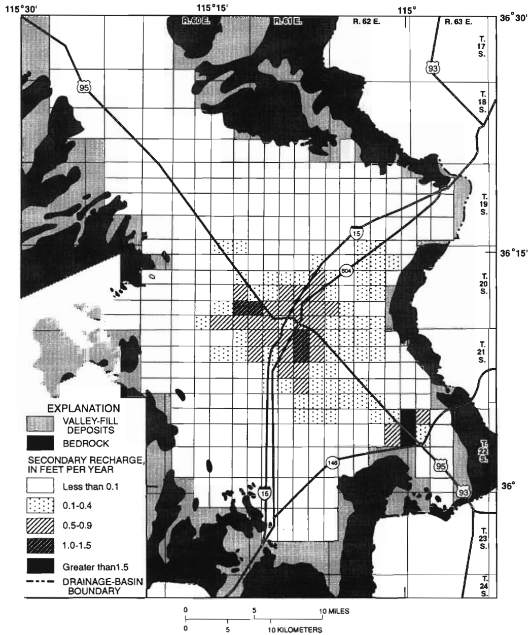
Figure 3.2.5-2. Estimated secondary recharge in 1972.
