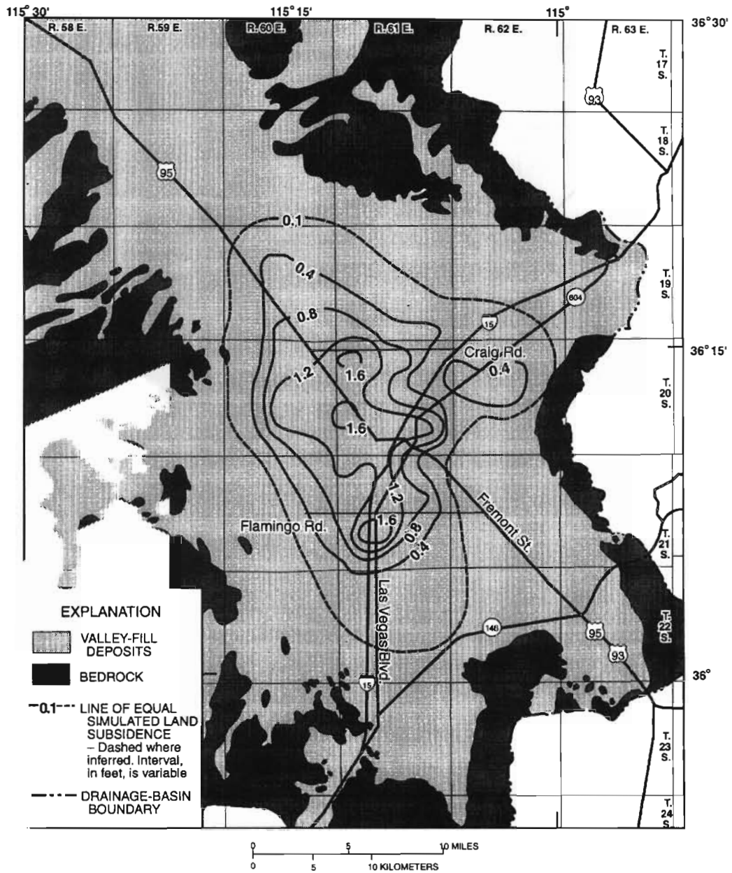
Figure 4.2.3.3-2. Simulated land subsidence, 1972-81.
