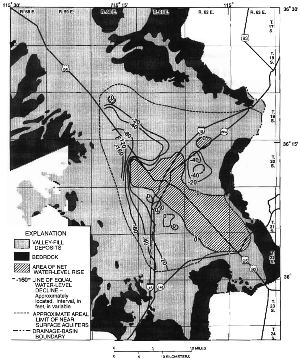
Figure 4.2.2-1. Approximate water-level change in near-surface aquifers, 1955-73 (from Harrill, 1976a, fig. 12).
