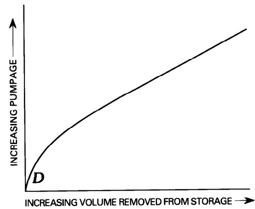
FIGURE 22.—Generalized geologic and hydrologic characteristics of the central basins. A , Physical system. B , Water budget before development. C , Flow-component response to pumping. D , Change in storage in response to pumping.
