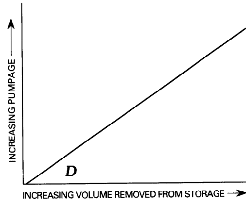
FIGURE 23.—Generalized geologic and hydrologic characteristics of the west basins. A, Physical system. B, Water budget before development. C, Flow-component response to pumping. D, Change in storage in response to pumping.
