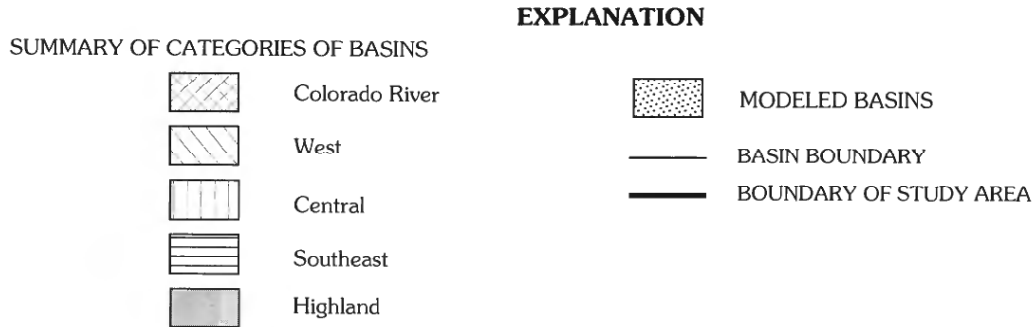
FIGURE 17.—Categories of alluvial basins based on geohydrologic factors.
