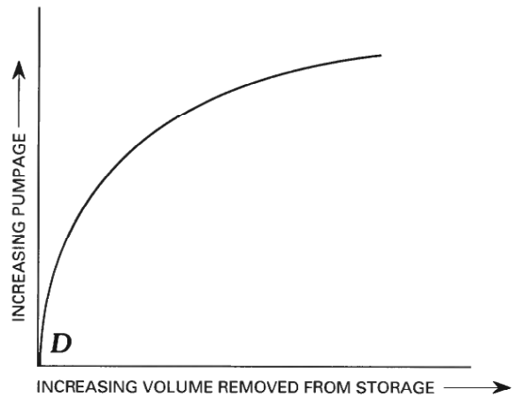
FIGURE 21.—Generalized geologic and hydrologic characteristics of the southeast basins. A, Physical system. B, Water budget before development. C, Flow-component response to pumping. D, Change in storage in response to pumping.
