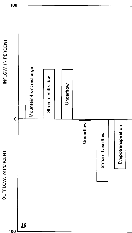
FIGURE 25.—Generalized geologic and hydrologic characteristics of the highland basins. A, Physical system. B, Water budget before development. C, Flow-component response to pumping. D, Change in storage in response to pumping.
