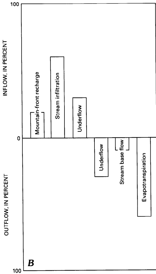
FIGURE 23.—Generalized geologic and hydrologic characteristics of the west basins. A, Physical system. B, Water budget before development. C, Flow-component response to pumping. D, Change in storage in response to pumping.
