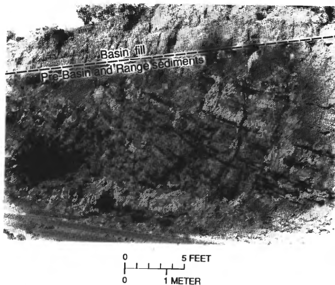
FIGURE 6.—Tilted pre-Basin and Range sediments overlain by basin fill near Tucson.
