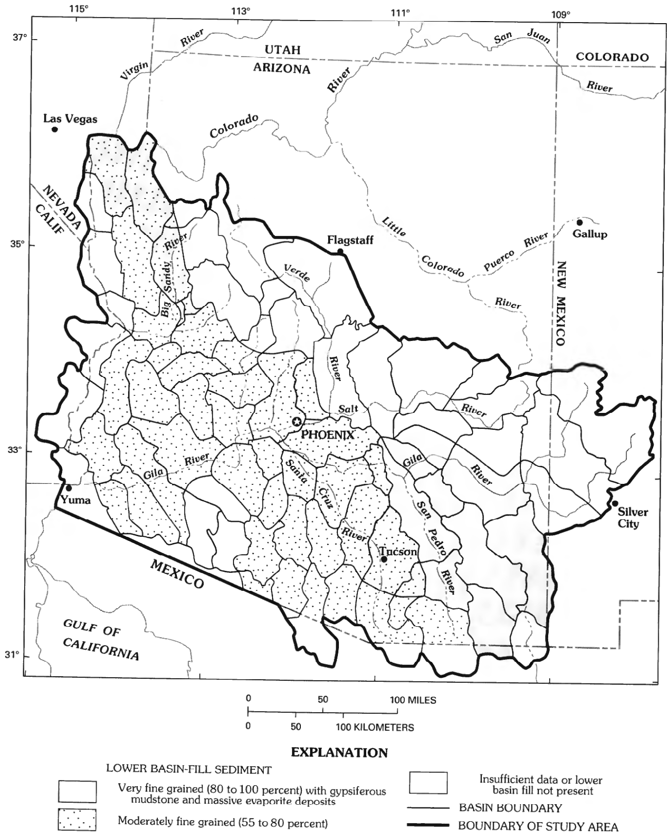
FIGURE 8.—Generalized areal extent of two groups of lower basin-fill sediments in the study area.
