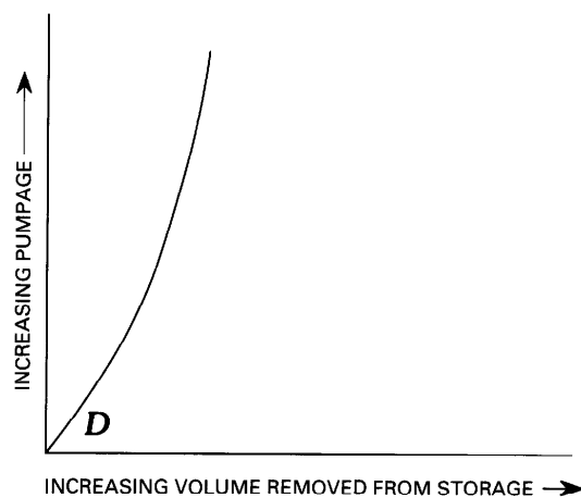
FIGURE 25.—Generalized geologic and hydrologic characteristics of the highland basins. A, Physical system. B, Water budget before development. C, Flow-component response to pumping. D, Change in storage in response to pumping.
