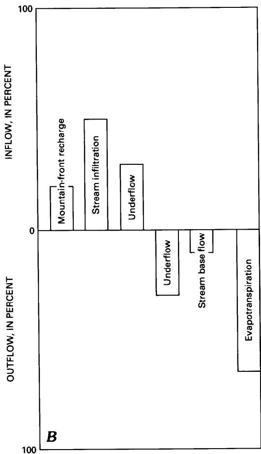
FIGURE 22.—Generalized geologic and hydrologic characteristics of the central basins. A , Physical system. B , Water budget before development. C , Flow-component response to pumping. D , Change in storage in response to pumping.
