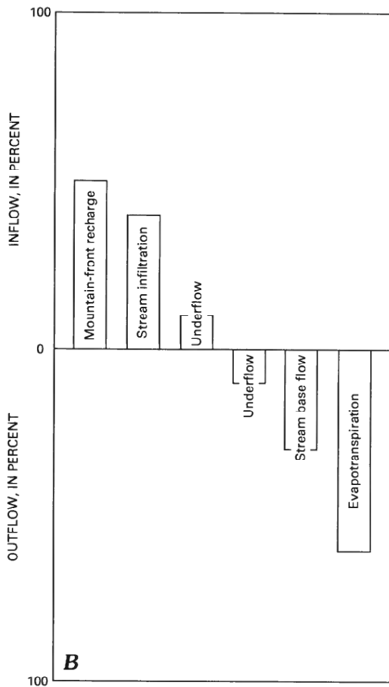
FIGURE 21.—Generalized geologic and hydrologic characteristics of the southeast basins. A, Physical system. B, Water budget before development. C, Flow-component response to pumping. D, Change in storage in response to pumping.
