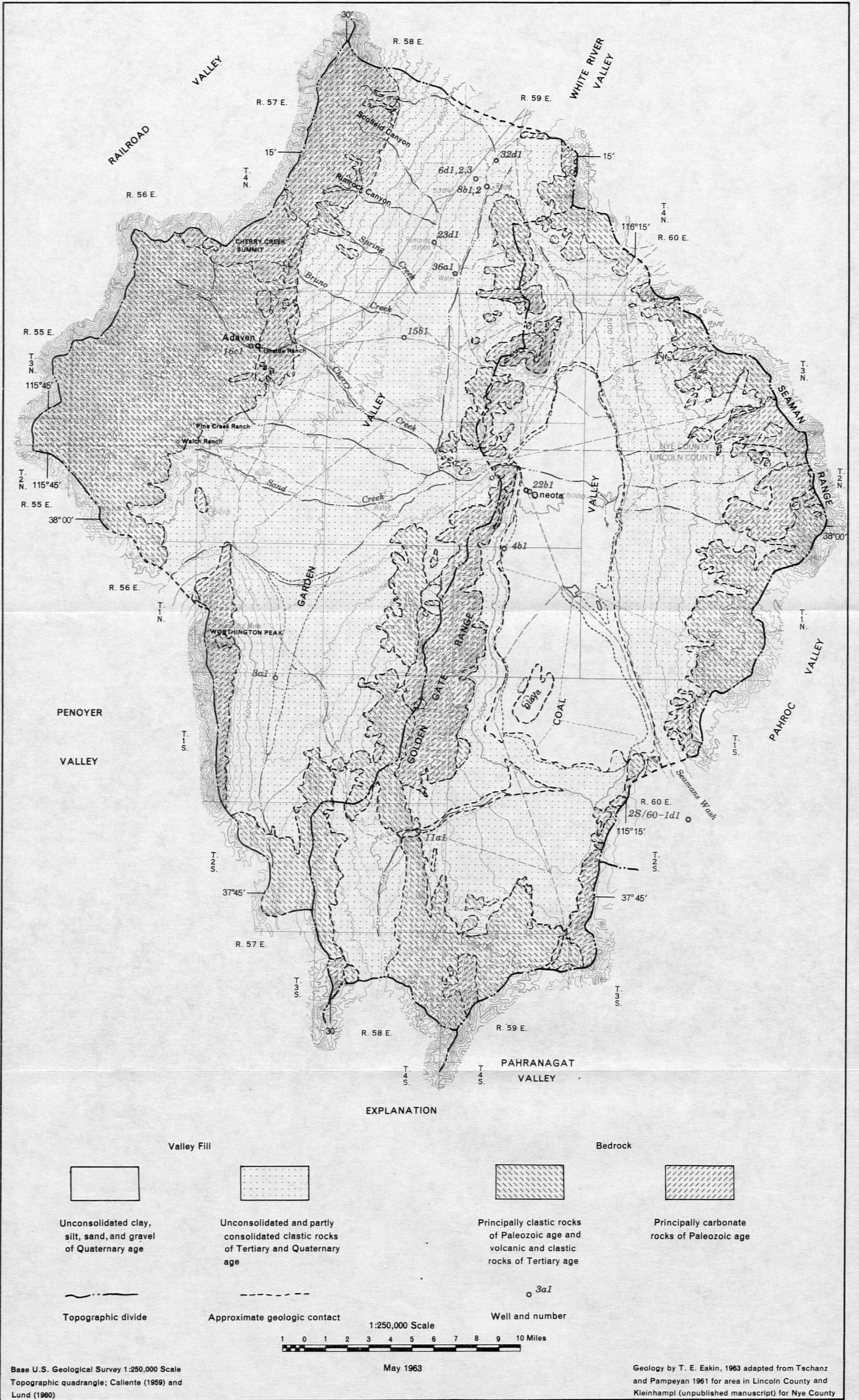
PLATE 1.—MAP OF THE GARDEN AND COAL VALLEYS, LINCOLN AND NYE COUNTIES, NEVADA SHOWING AREAS OF BEDROCK, VALLEY FILL, AND LOCATION OF WELLS
