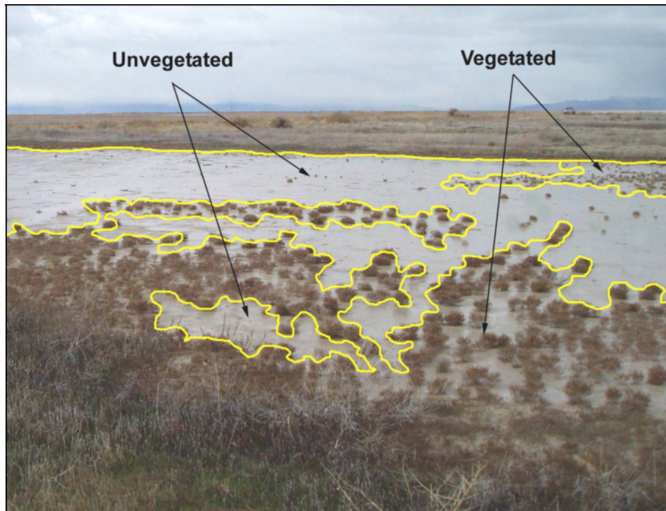
Figure 44. Example of sparse and patchy plant cover in a wetland. Areas labeled as vegetated have \geq 5 percent plant cover.
