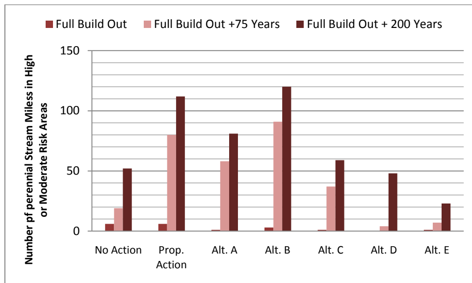
Figure 3.3.2-41 Miles of Perennial Streams Located within the Drawdown Area and Areas Where Impacts to Flow Could Occur (High or Moderate Risk Areas)
