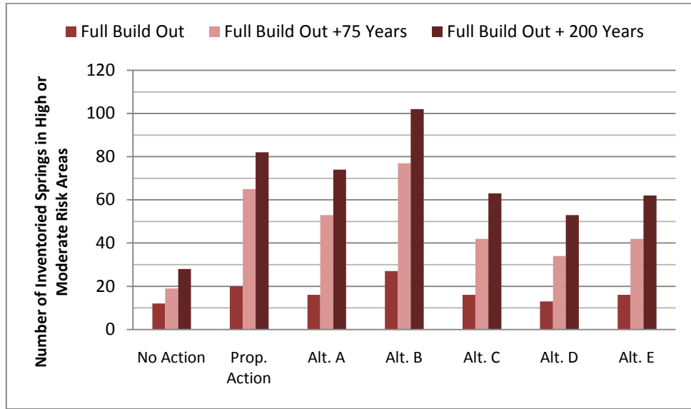
Figure 3.3.3-6 Number of Inventoried Springs Located within the Cumulative Drawdown Area and Areas Where Impacts to Flow Could Occur
