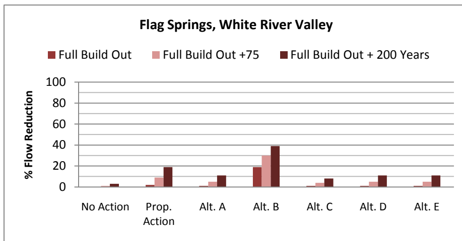
Figure 3.3.3-8 Model-simulated Cumulative Reduction in Flows at Preston Big Springs, Butterfield Springs, and Flag Springs 3, White River Valley
