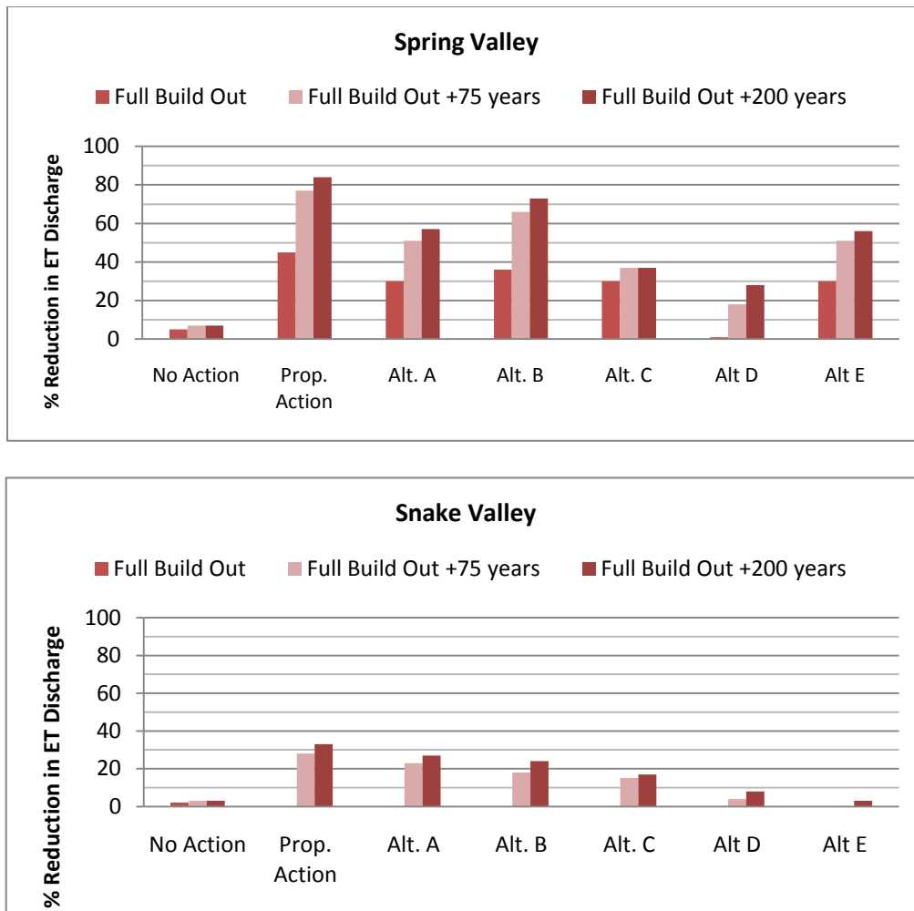
Figure 3.3.2-42 Model-simulated Reductions in Groundwater Discharge to Evapotranspiration Areas in Spring and Snake Valleys
