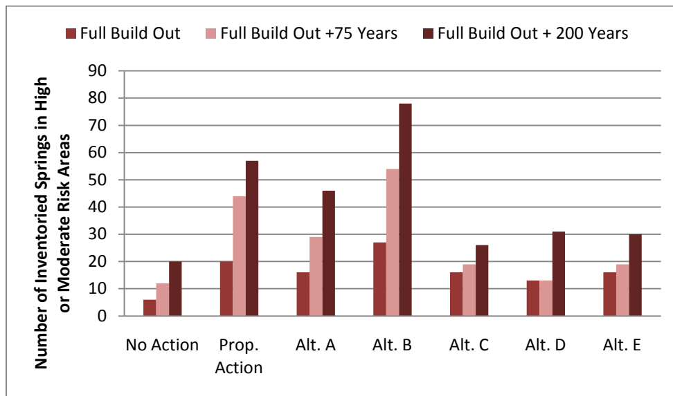
Figure 3.3.2-40 Number of Inventoried Springs Located within the Drawdown Area and Areas Where Impacts to Flow Could Occur (High or Moderate Risk Areas)
