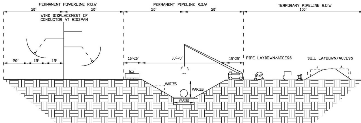
Figure ES-6 Preliminary Pipeline and Power Line ROW Cross Section
