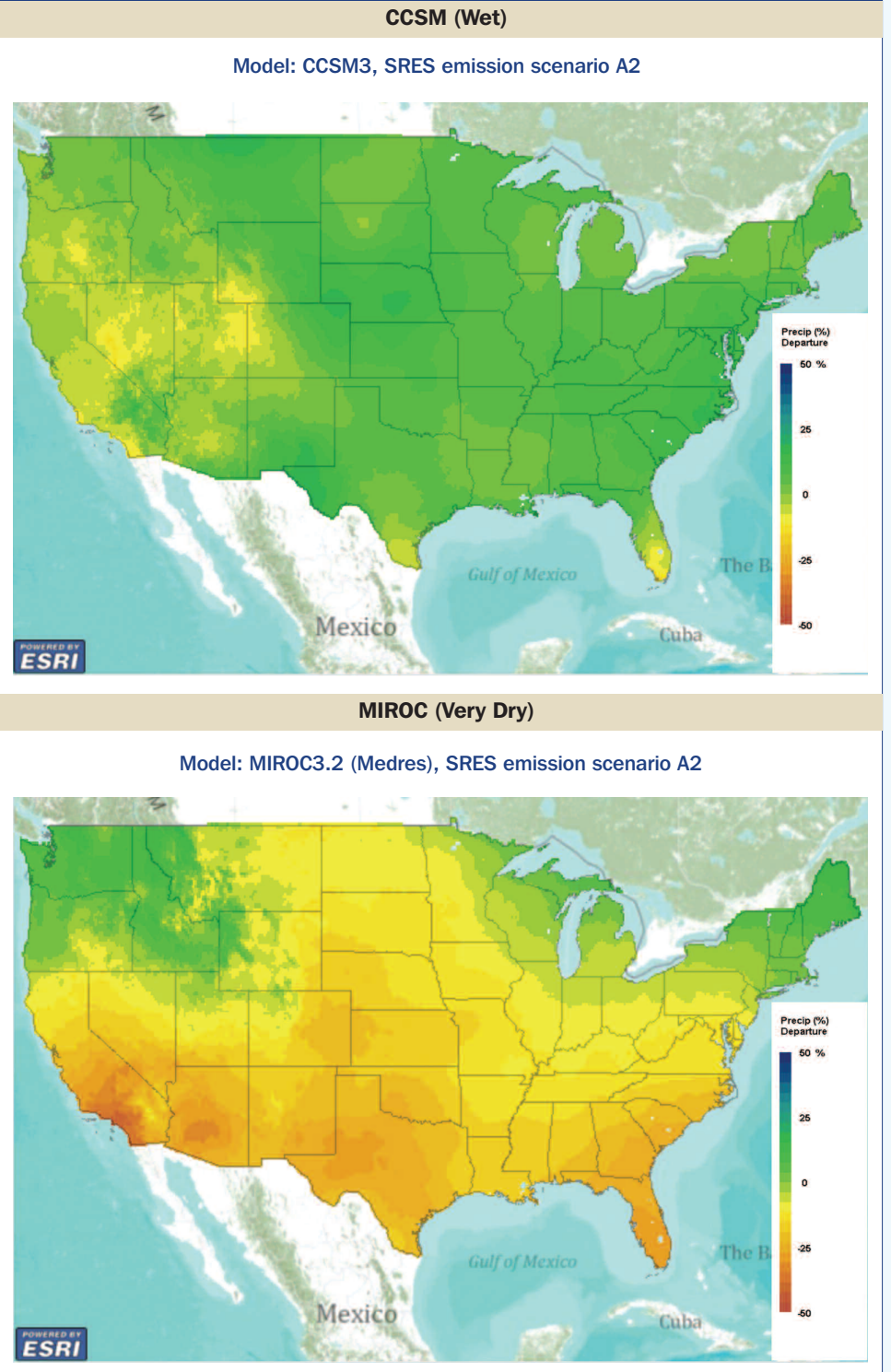
Exhibit 2: Change in Annual Precipitation by 2050 Under Two Climate Scenarios
