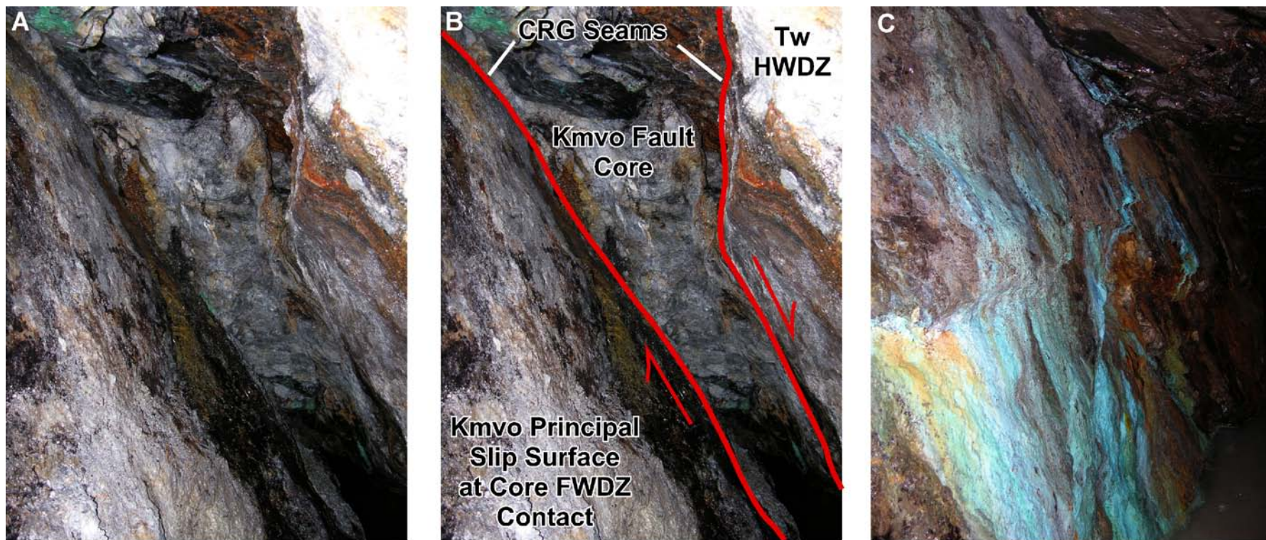
Figure 18. Photographs of the Standard fault vein from Levels 3 and 5 in the Standard Mine. (A) View of the Ohio Creek Member of Mesaverde Formation (Kmvo) footwall principal slip surface, Ohio Creek fault core, and Wasatch Formation (Tw) hanging wall in Level 3. The fault core is up to 60 cm wide here. (B) Annotated version of figure 18A. (C) Asymmetric groundwater flow and probable copper-rich precipitate on the Ohio Creek footwall principal slip surface of the Standard fault vein in Level 3.
