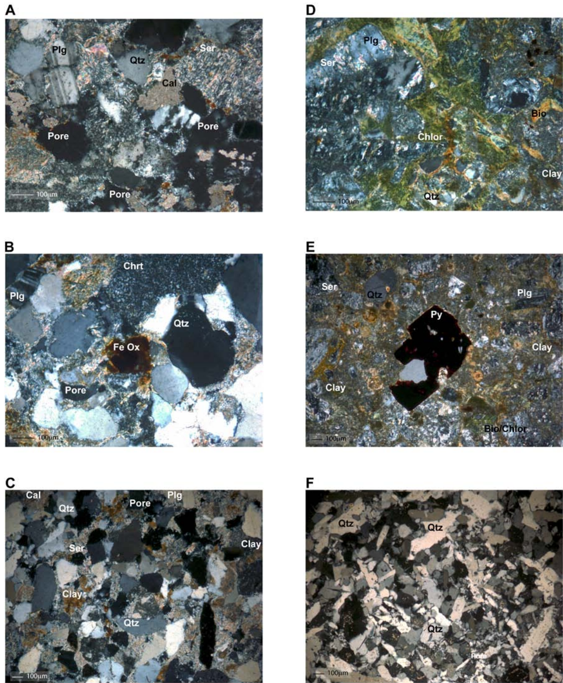
Figure 13. Thin section photomicrographs of representative outcrop samples from Elk Basin. (A) Ohio Creek Member of Mesaverde Formation footwall protolith sandstone, about 20 m northwest of the Standard fault vein near the Level 1 portal (sample 70909 7A). (B) Ohio Creek Member footwall protolith sandstone, about 100 m northwest of the Standard fault vein at the Level 3 portal (sample 70909 14A). (C) B8 drill core Ohio Creek footwall protolith sandstone, about 3 m northwest of the Standard fault vein below the Level 2 portal from 23 m below ground surface, 5x magnification (sample B8 75 Feet). (D) and (E) Wasatch Formation hanging wall protolith sandstone, about 80 m southeast of the Standard fault vein between the Level 4 and 5 portals, view (E) is 5x magnification (sample 72209 10A). (F) Wasatch Formation hanging wall damage and mineralized zone, about 1 meter southeast of the Standard fault vein at the Level 1 portal, 5x magnification (sample 72209 10A). Abbreviations include: Qtz = quartz, Plg = plagioclase feldspar, Cal = calcite, Pore = pore space, Chrt = chert, Clay = unidentified clay minerals, Fe Ox = iron oxidation, Py = pyrite, Chlor = chlorite. Scale bars are shown at the bottom of each image, all images use crossed polarized light and are 10x magnification unless noted.
