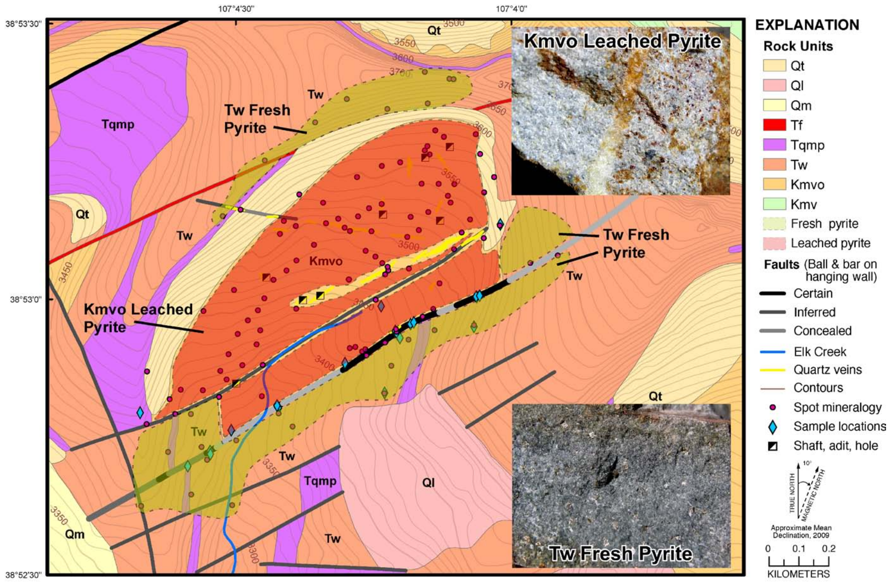
Figure 12. Reconnaissance geologic map of upper Elk Basin showing the spot mineralogy and extent of leached pyrite (orange overlay) versus fresh pyrite (light green overlay) from freshly broken hand samples from the ground surface. Photographs show examples of orange, iron oxide staining in cubic holes where pyrite likely originally resided in Ohio Creek Member (top, sample face is about 2 by 3 in) and fresh pyrite in Wasatch Formation (bottom, sample face is about 2 by 3 in). Modified from Gaskill and others, 1967. Qt, Quaternary talus deposits; Ql, Quaternary landslide deposits; Qm, Quaternary glacial deposits; Tf, Tertiary felsite; Tqmp, Tertiary quartz monzonite porphyry; Tw, Tertiary Wasatch Formation; Kmvo, Upper Cretaceous Ohio Creek Member of Mesaverde Formation; Kmv, Upper Cretaceous Mesaverde Formation.
