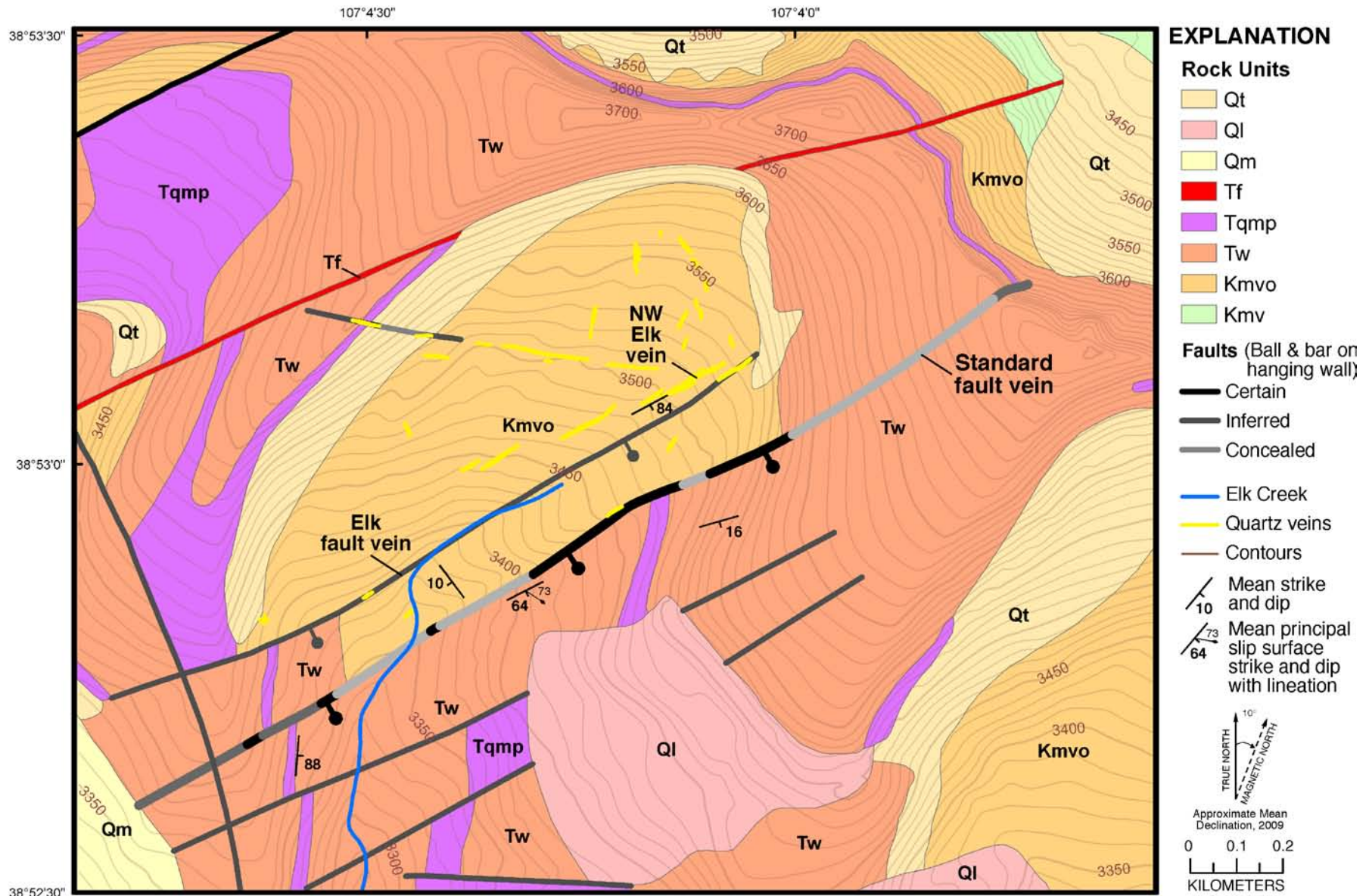
Figure 7. Reconnaissance geologic map of upper Elk Basin modified from Gaskill and others, 1967 revised by Jonathan Caine, 2009. Qt, Quaternary talus deposits; Ql, Quaternary landslide deposits; Qm, Quaternary glacial deposits; Tf, Tertiary felsite; Tqmp, Tertiary quartz monzonite porphyry; Tw, Tertiary Wasatch Formation; Kmvo, Upper Cretaceous Ohio Creek Member of Mesaverde Formation; Kmv, Upper Cretaceous Mesaverde Formation.
