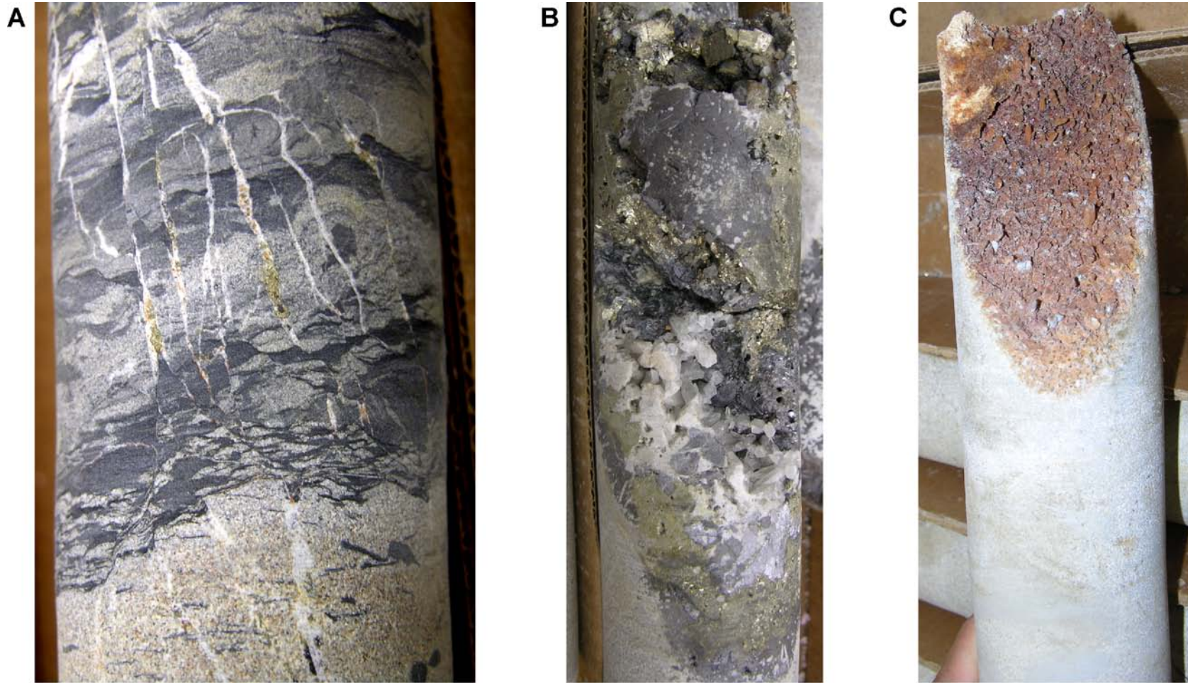
Figure 17. Photographs of drill core from borehole B8, just below Portal 2 of the Standard Mine, in the Ohio Creek Member of Mesaverde Formation footwall damage zone of the Standard fault vein. Each core is approximately 2 in. in diameter. (A) 76 ft, small quartz + pyrite fault veins; (B) 114 ft, vuggy quartz + pyrite + galena + sphalerite vein; (C) 170 ft, iron oxide stain on euhedral quartz vein.
