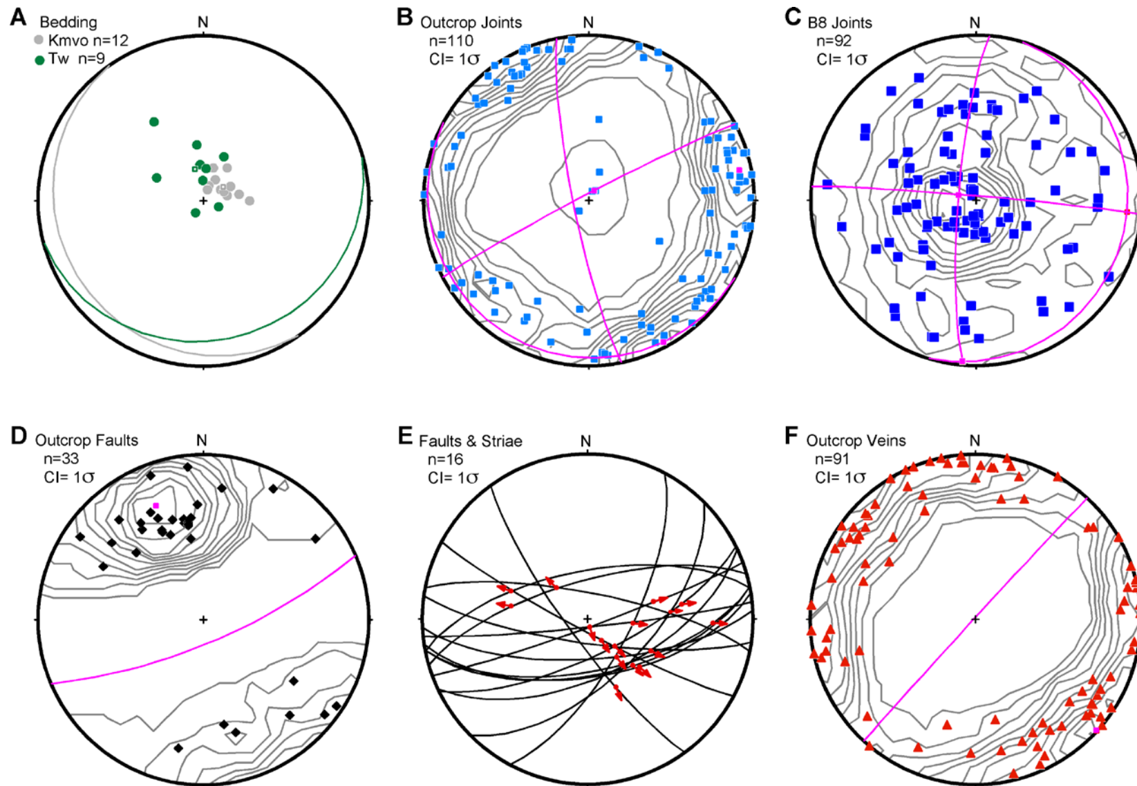
Figure 9. Lower-hemisphere, equal-area projections of structural orientation data collected in Elk Basin ( n = number, CI = contour interval, and \sigma = standard deviation). (A) Poles to bedding data collected in outcrop for the Upper Cretaceous Ohio Creek Member of Mesaverde Formation (gray circles) and Tertiary Wasatch Formation (green circles). The mean great circles for each formation are shown. (B) Kamb contoured (gray lines) poles (blue squares) to all joints collected from outcrop (Kamb, 1959). (C) Kamb contoured (gray lines) poles (blue squares) to all joints measured from in the B8 borehole image log. (D) Kamb contoured (gray lines) poles (black diamonds) to all faults collected from outcrop. (E) Slip-linear diagram for faults in outcrop that have slickenlines and shear sense indicators. Each black great circle is a single fault with its slip linear shown as a red dot. The red arrows for each dot show the direction of the hanging wall relative to the footwall of each fault. (F) Kamb contoured (gray lines) poles (red triangles) to all quartz or polymetallic veins collected from outcrop. The mean vectors and great circles for assumed cylindrical best fits to each data set are shown in pink (see Allmendinger, 2004).
