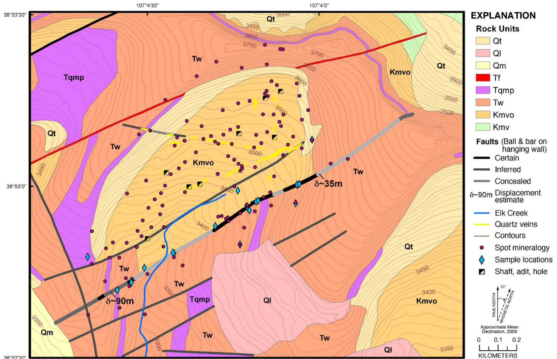
Figure 11. Reconnaissance geologic map of upper Elk Basin showing the locations of field-based spot mineralogy determinations, fault-vein rock samples, adits, shafts, dog holes, and estimates of net displacement ( \delta ). Modified from Gaskill and others, 1967. Qt, Quaternary talus deposits; Ql, Quaternary landslide deposits; Qm, Quaternary glacial deposits; Tf, Tertiary felsite; Tqmp, Tertiary quartz monzonite porphyry; Tw, Tertiary Wasatch Formation; Kmvo, Upper Cretaceous Ohio Creek Member of Mesaverde Formation; Kmv, Upper Cretaceous Mesaverde Formation
