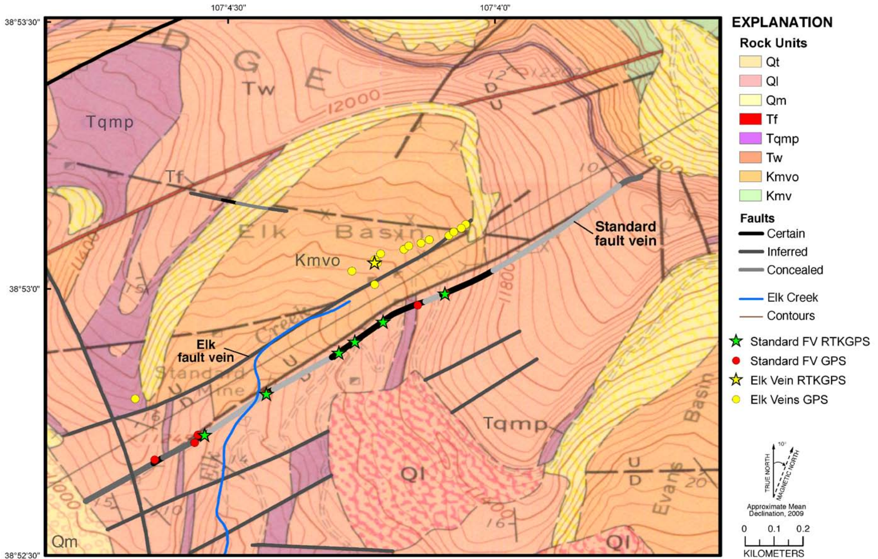
Figure 6. Gaskill and others (1967) geologic map (1:24,000) of upper Elk Basin overlain with the Real Time Kinematic and handheld GPS positions of the Standard and Elk fault veins. Qt, Quaternary talus deposits; Ql, Quaternary landslide deposits; Qm, Quaternary glacial deposits; Tf, Tertiary felsite; Tqmp, Tertiary quartz monzonite porphyry; Tw, Tertiary Wasatch Formation; Kmvo, Upper Cretaceous Ohio Creek Member of Mesaverde Formation; Kmv, Upper Cretaceous Mesaverde Formation; FV, fault vein; RTKGPS, real time kinematic global positioning system; GPS handheld global positioning system.
