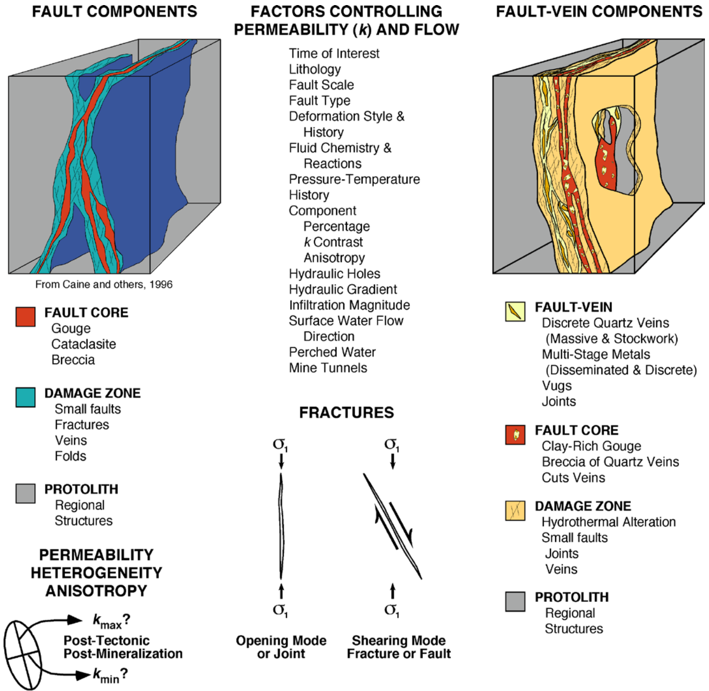
Figure 4. Fault zone, fracture, and fault vein conceptual models showing physical components and potential hydrological influences. The ellipse depicts the possible directions of maximum and minimum permeability for a fault or fault vein after they have formed causing them to be complex conduit-barrier systems. A sketch of the basic types of fractures found in nature with the ideal maximum principal stress ( \sigma_1 ) orientation that controls their formation is also shown.
