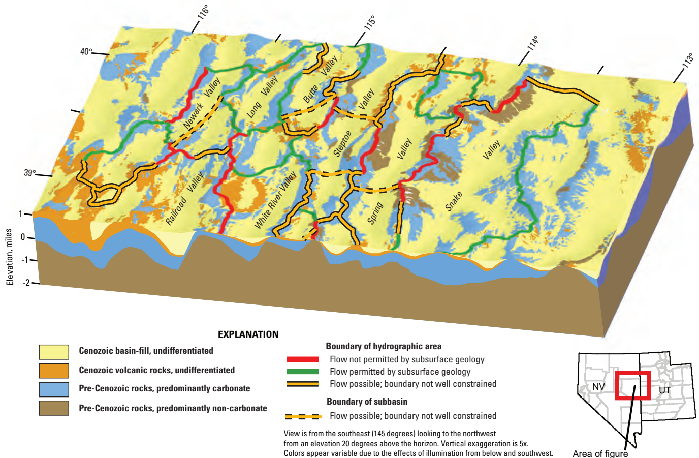
Perspective view of the primary aquifer systems.
