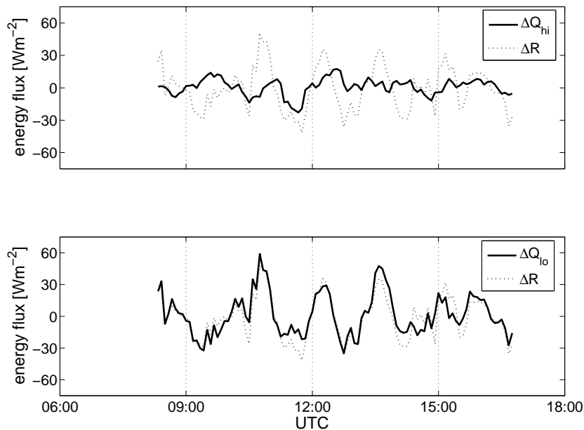
Fig. 1. Comparison of the change of the turbulent fluxes of sensible and latent heat in the high frequency range ( \Delta Q_{r\,m\,h\,i} ) and the low frequency range ( \Delta Q_{l\,o} ) and the change of the residual of the energy balance closure ( \Delta R ) for 30 min averages determined for time steps of 5 min. A moving average (daily cycle) was subtracted (8 June 2003).
