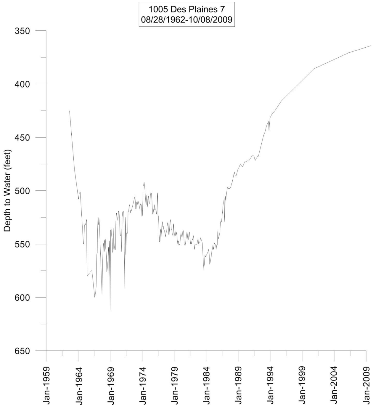
Figure 4 Depth to water in observation well 1005 (Des Plaines 7).
