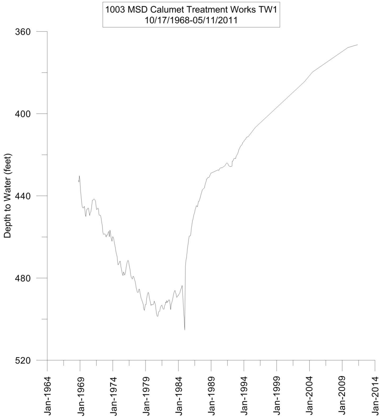
Figure 3. Depth to water in observation well 1003 (MSD Calumet Treatment Works TW1).
