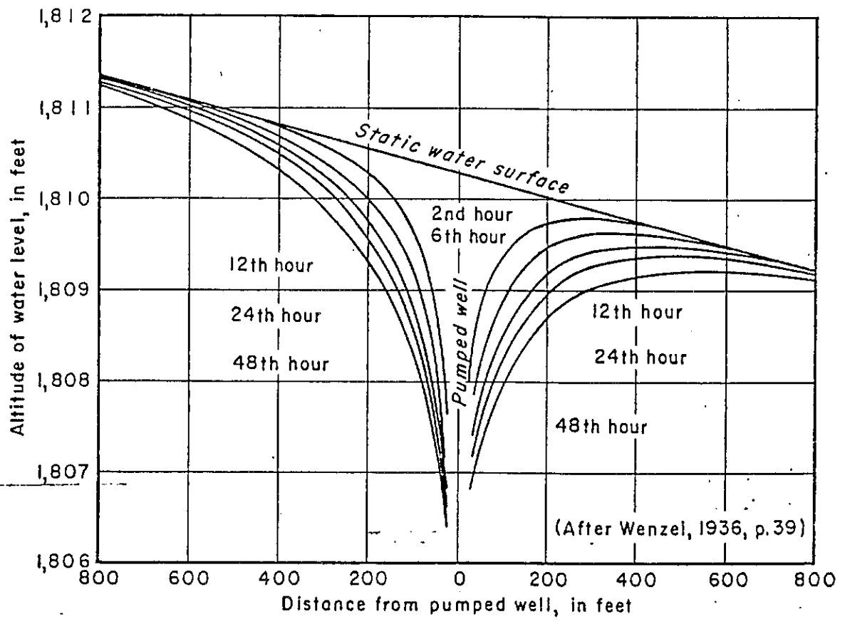
Figure 2-- Growth of cone of depression during pumping test in Platte Valley, Nebraska
