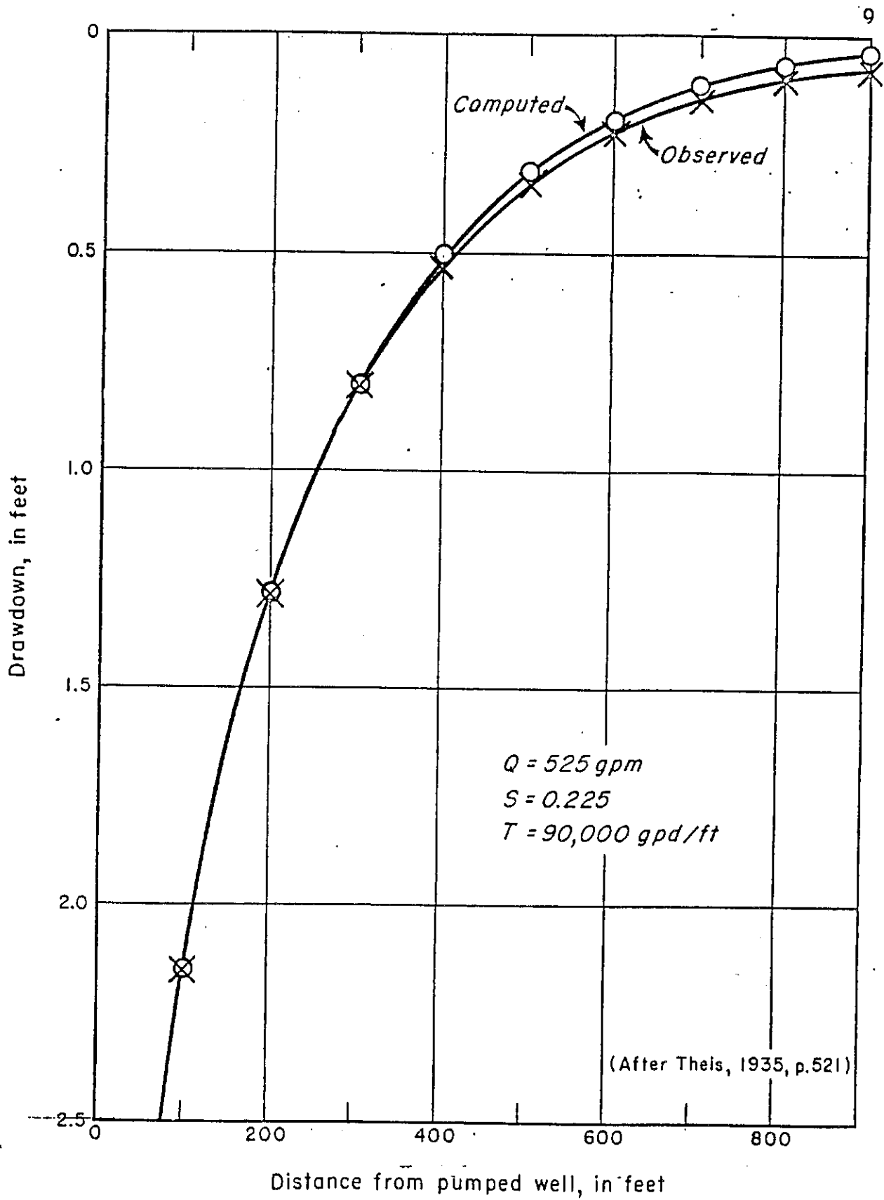
Figure 3-- Observed and computed drawdowns in the vicinity of a well after pumping 48 hours
