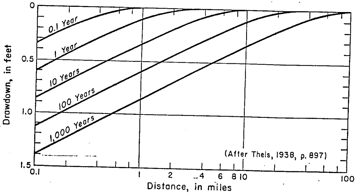
Figure 5 -- Drawdown for same conditions as those of Figure 4, plotted against distance from discharging well
