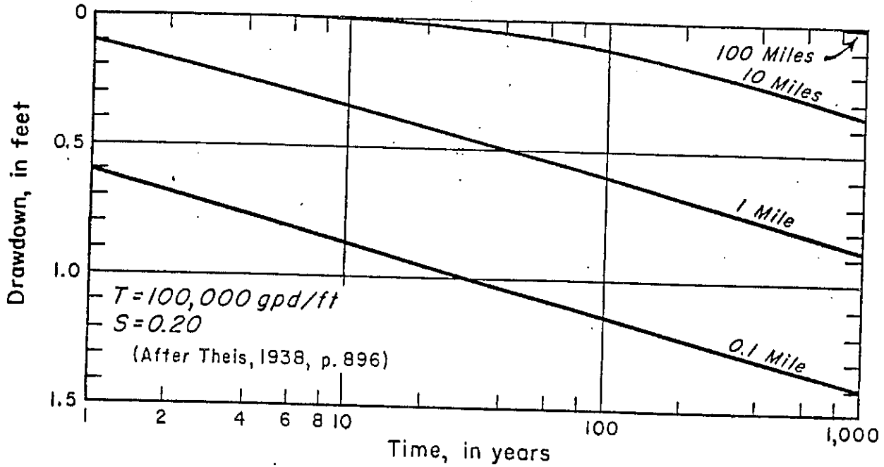
Figure 4 -- Drawdown in an ideal aquifer caused by continuous discharge of a well at the rate of 100 gallons per minute
