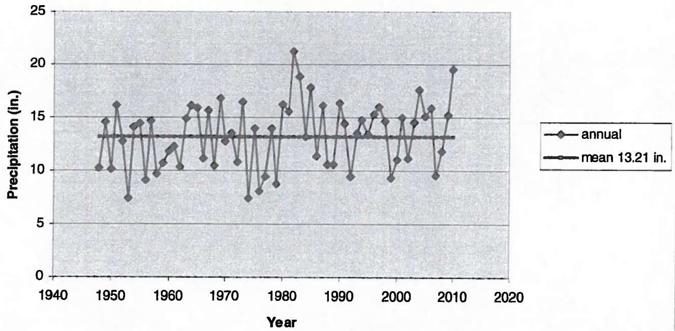
GBNP Mean Annual Precipitation
