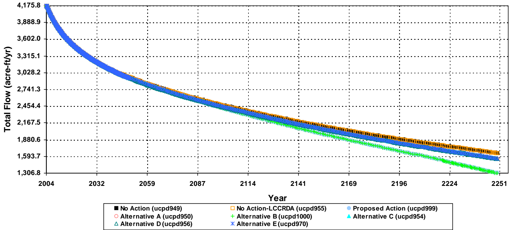
Simulated Stream / Spring Flow Changes at Muddy River at Overton G_OVERT
