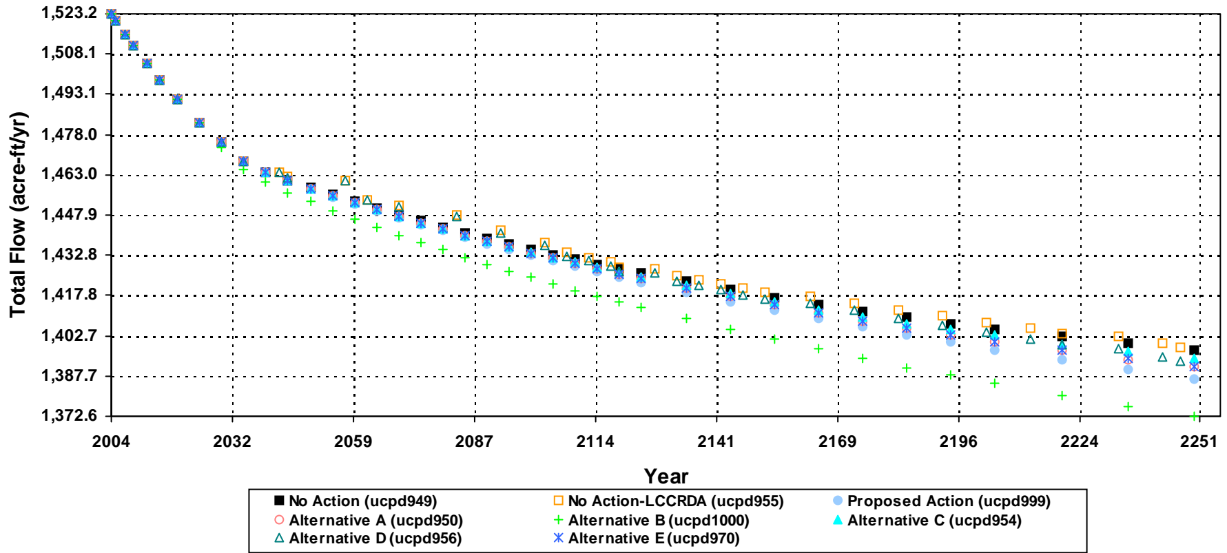
Simulated Stream / Spring Flow Changes at Arnoldson Spring SPiw07_2
