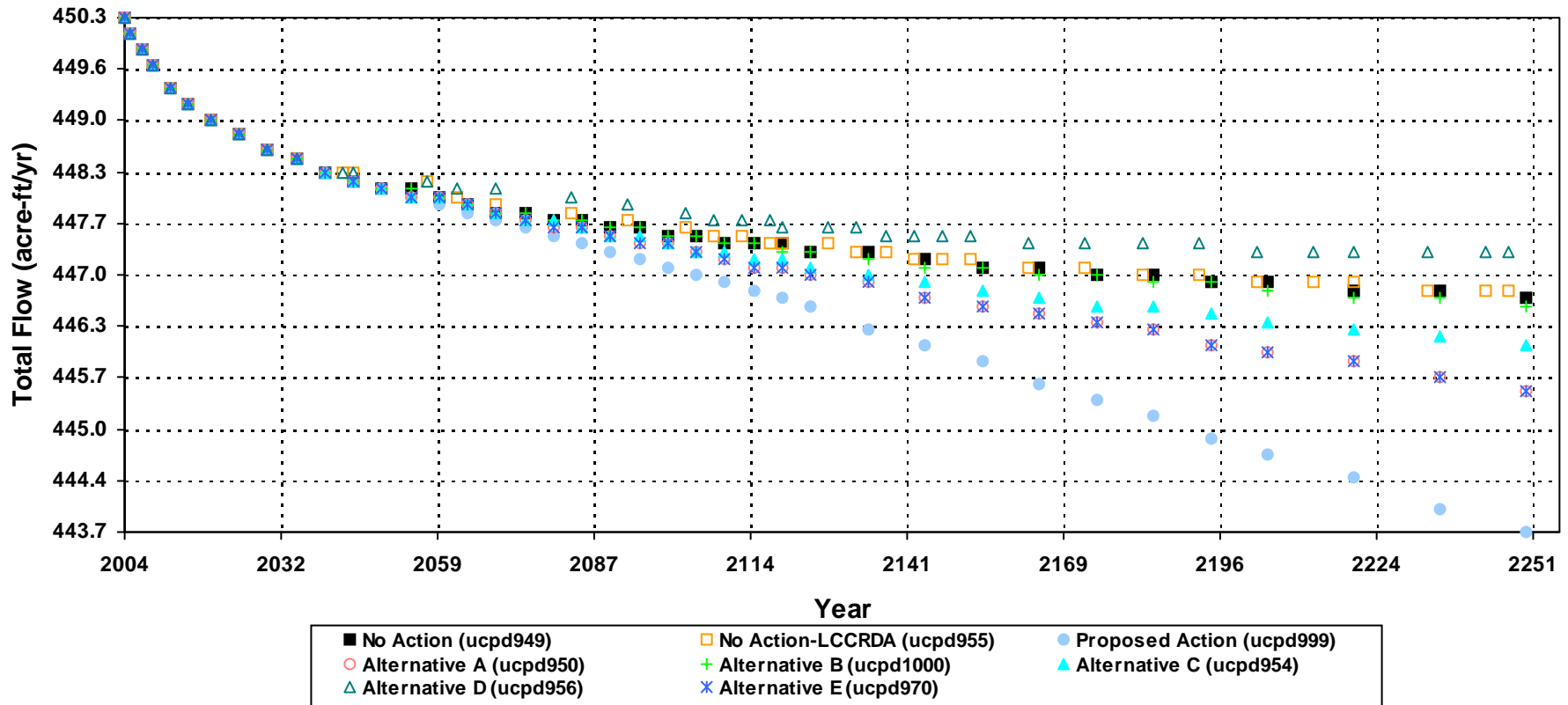
Simulated Stream / Spring Flow Changes at Monte Neva Hot Springs SPr79_3
