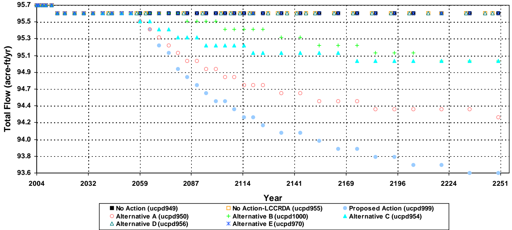
Simulated Stream / Spring Flow Changes at Kell Spring SPis95_13
