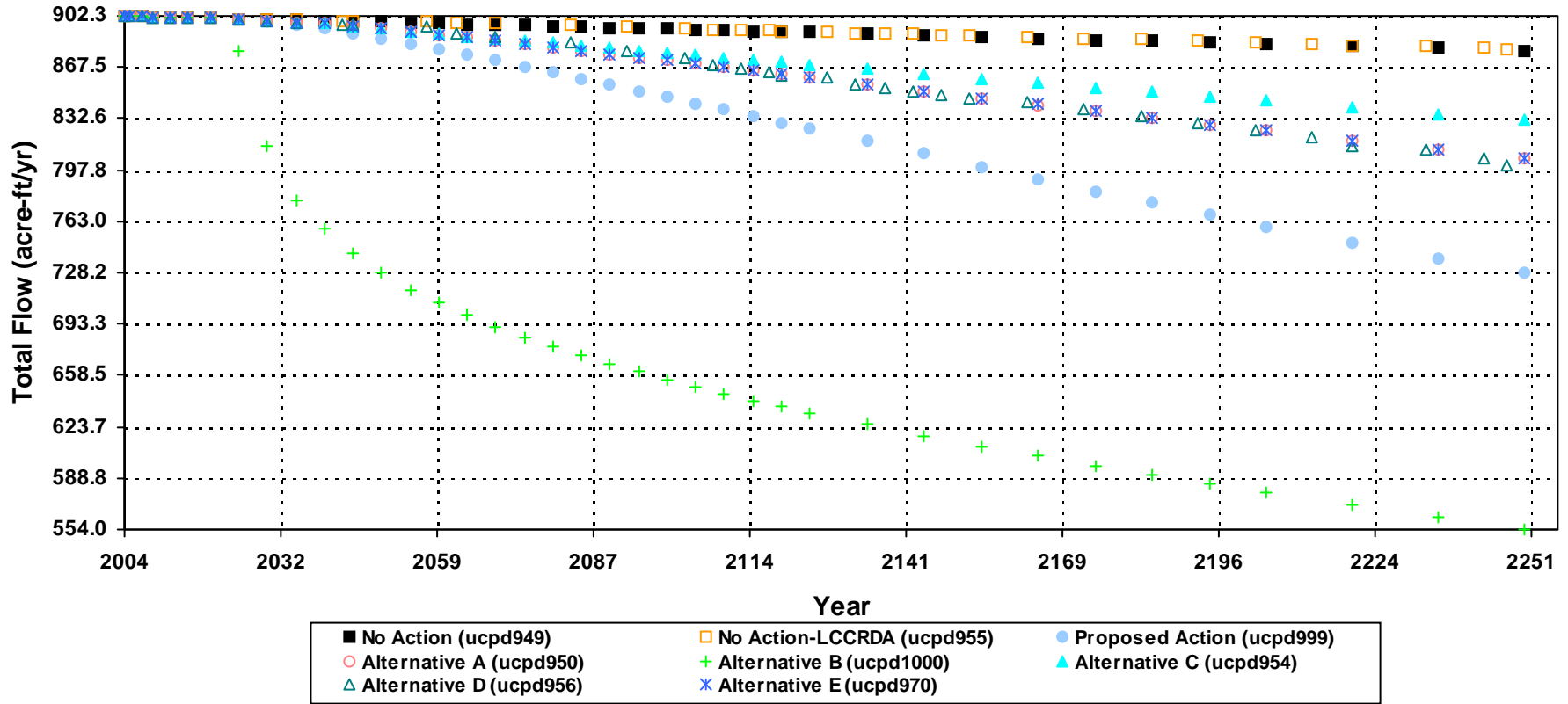
Simulated Stream / Spring Flow Changes at Flag Springs 3 SPiw07_7
