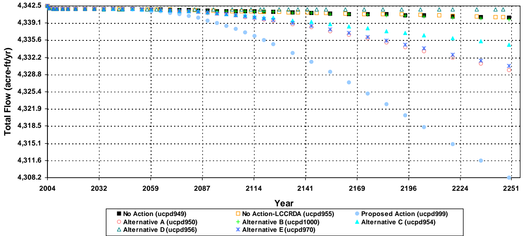
Simulated Stream / Spring Flow Changes at Warm Creek near Gandy, UT
