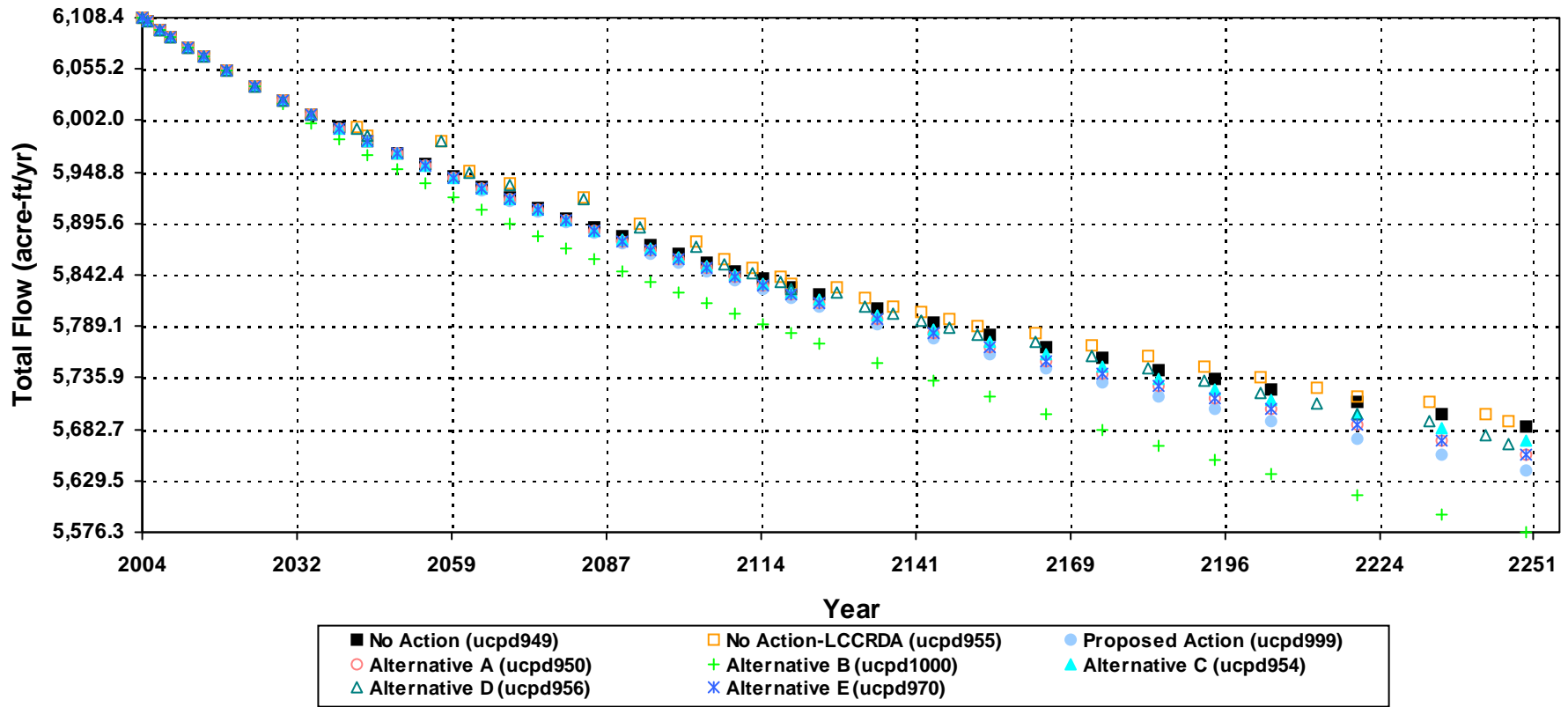
Simulated Stream / Spring Flow Changes at Preston Big Spring SPr07_4
