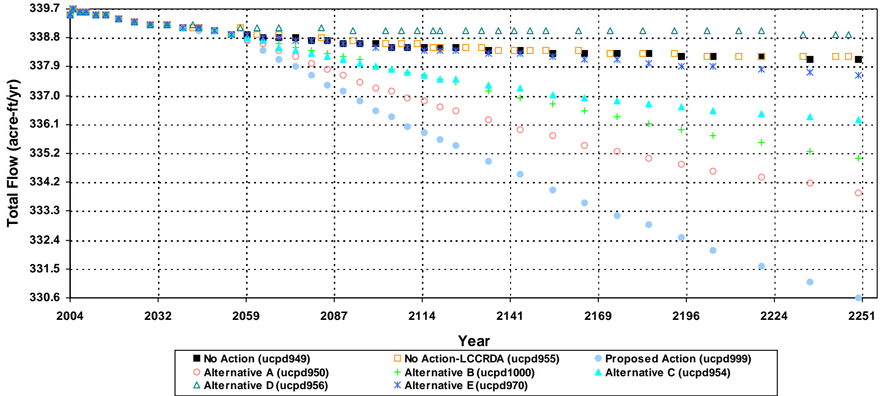
Simulated Stream / Spring Flow Changes at Foote Res. Spring SPib95_12
