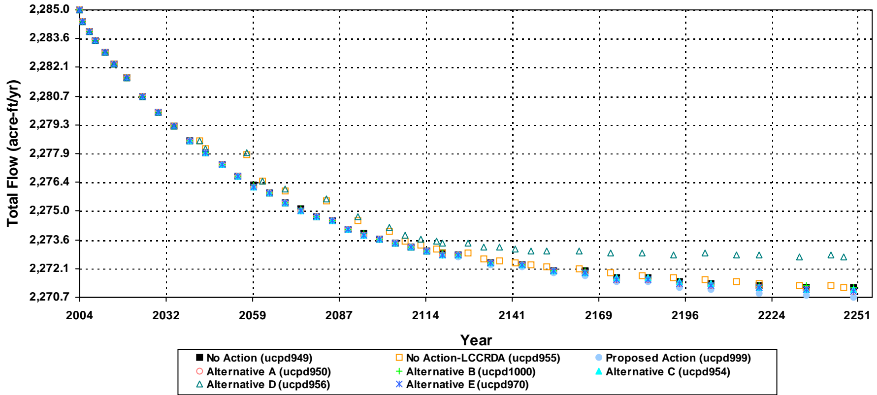
Simulated Stream / Spring Flow Changes at Currie Spring SPib79_6
