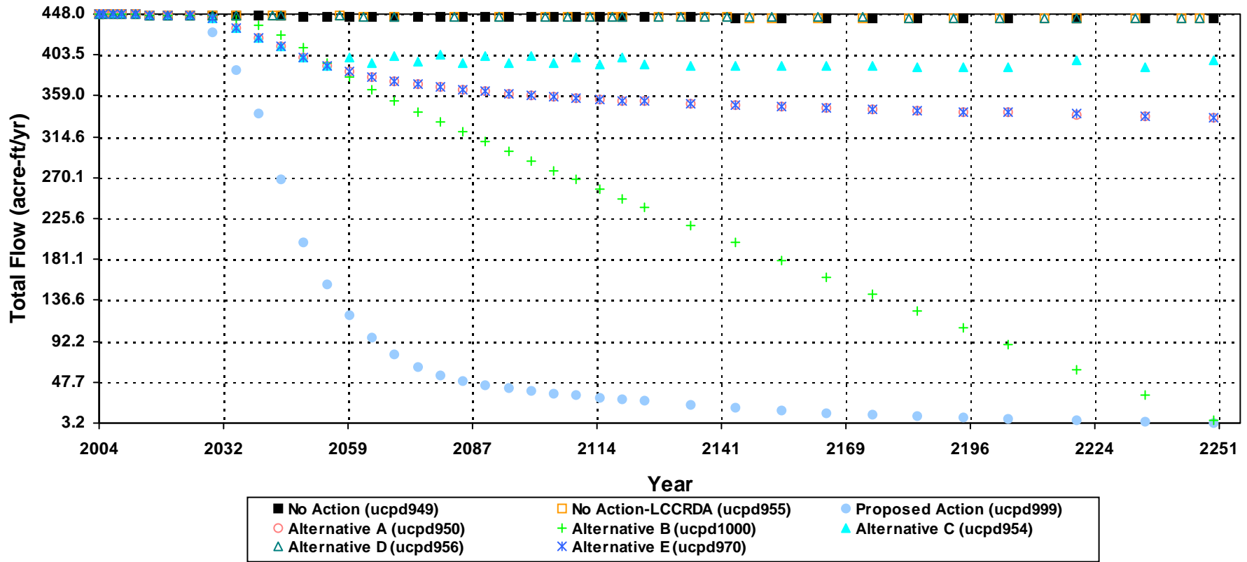
Simulated Stream / Spring Flow Changes at South Millick Spring SPib84_4
