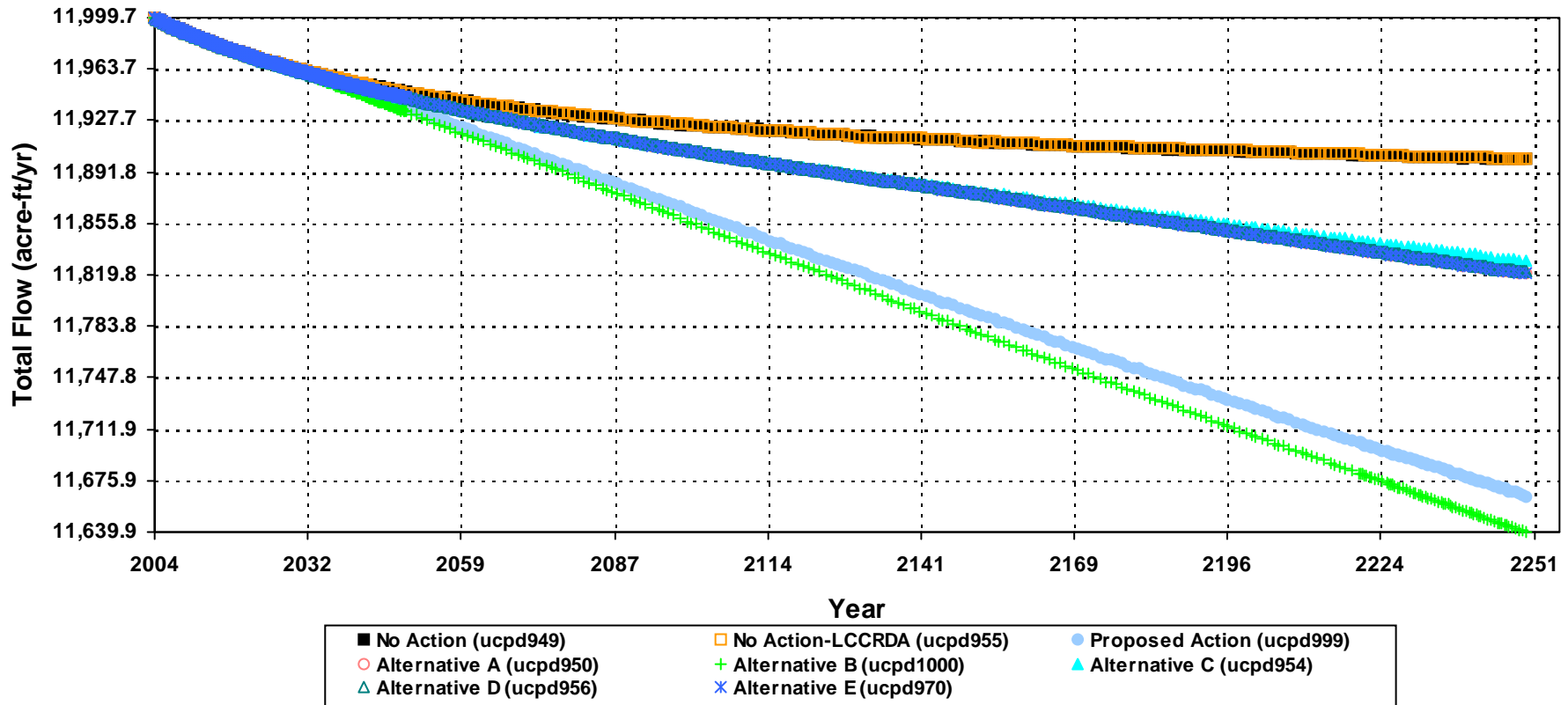
Simulated Stream / Spring Flow Changes at Ash Springs G_ASH
