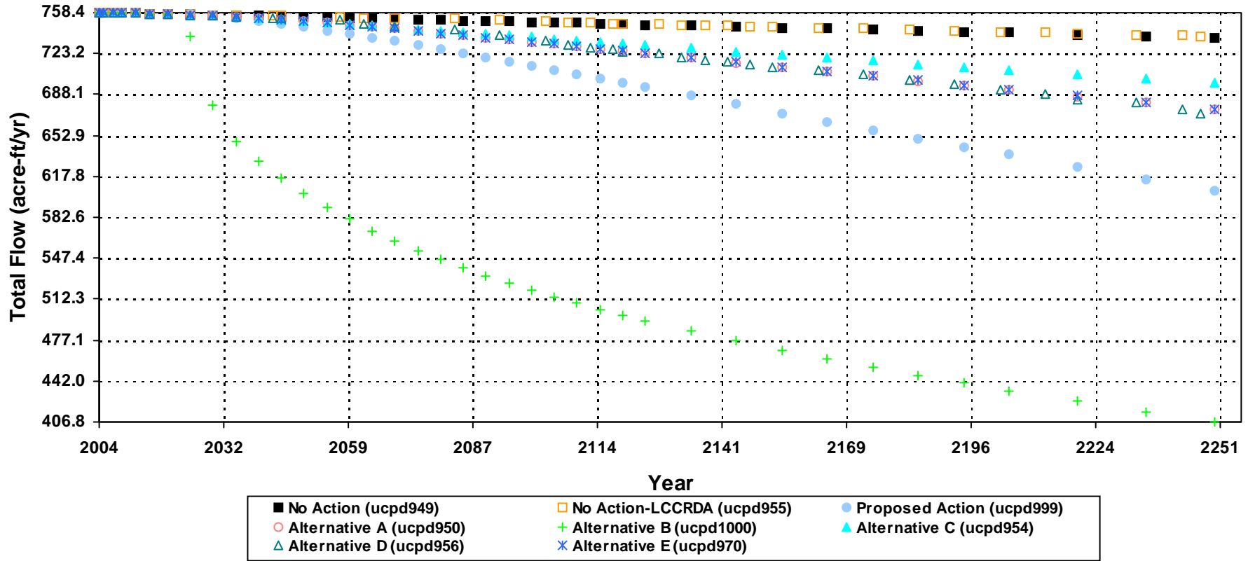
Simulated Stream / Spring Flow Changes at Butterfield Spring SPib07_10
