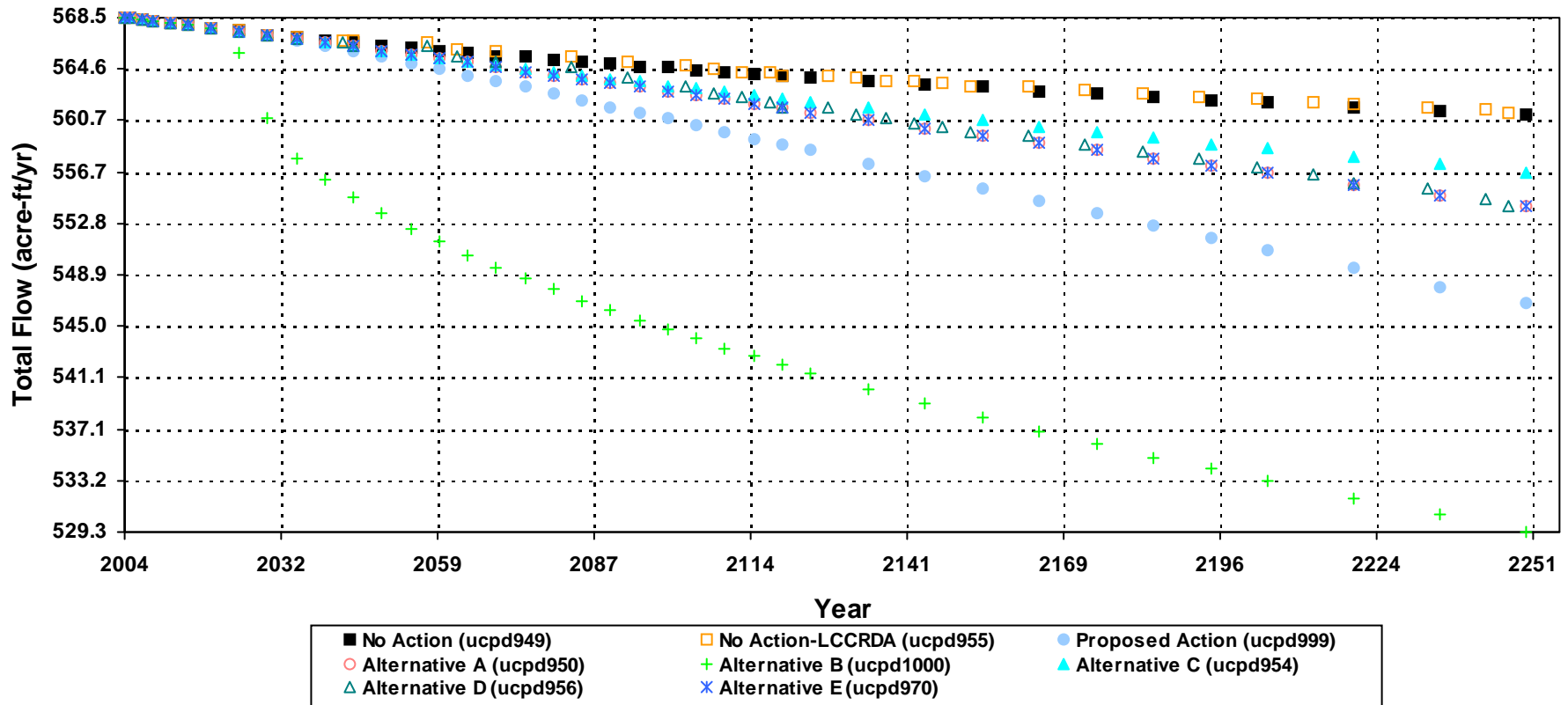
Simulated Stream / Spring Flow Changes at Moorman Spring
