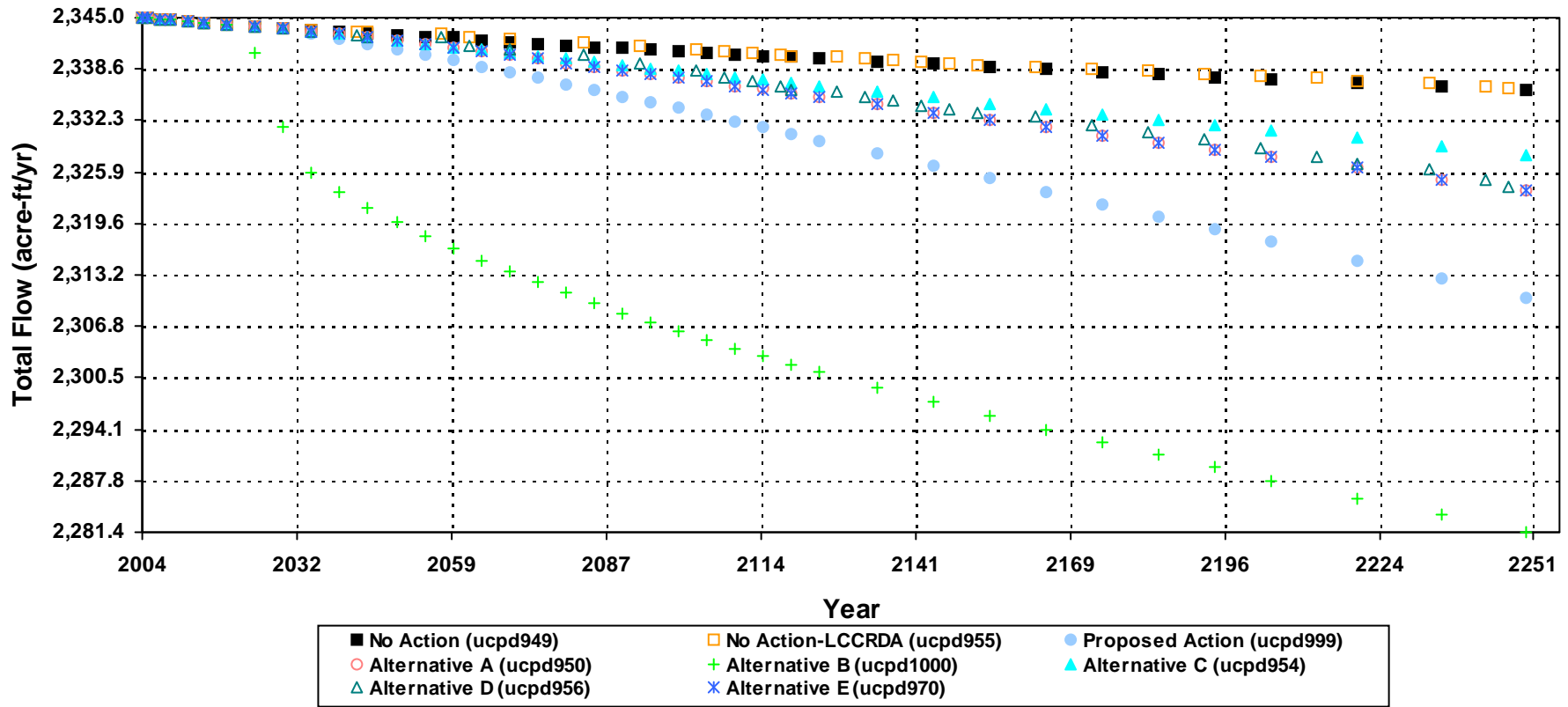
Simulated Stream / Spring Flow Changes at Moon River Spring
