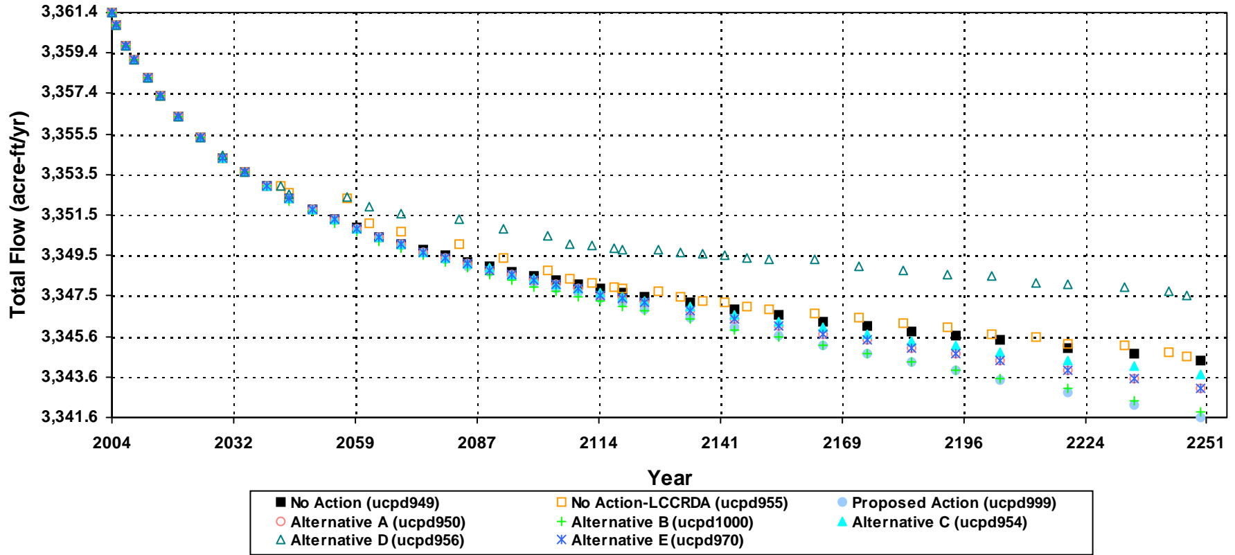
Simulated Stream / Spring Flow Changes at Campbel Ranch Springs
