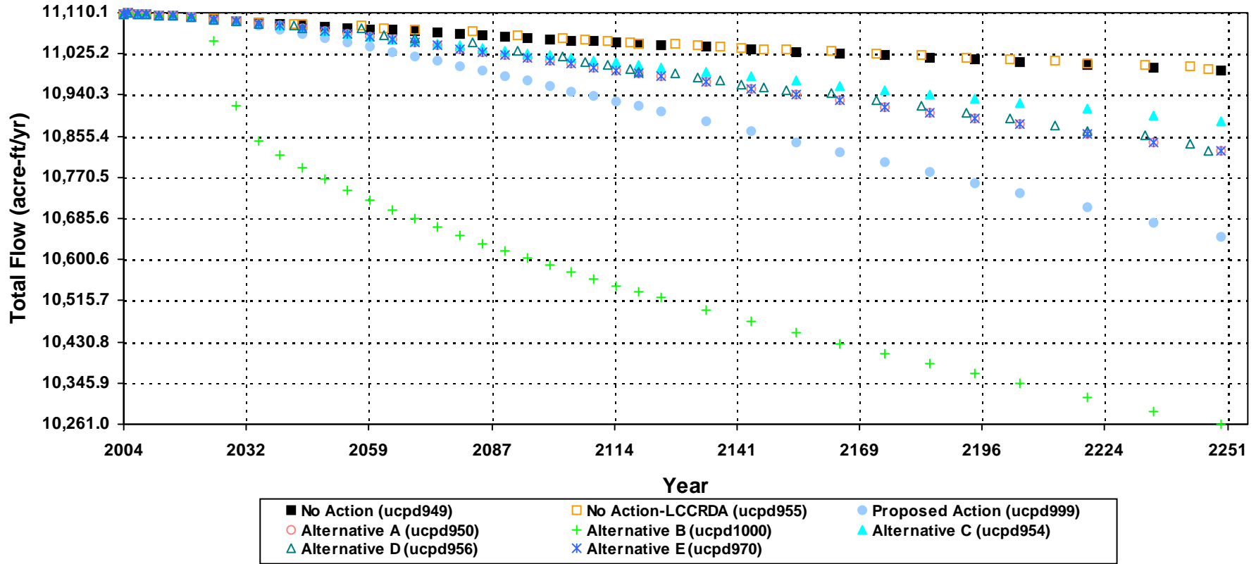
Simulated Stream / Spring Flow Changes at Hot Creek Spring SPr07_1
