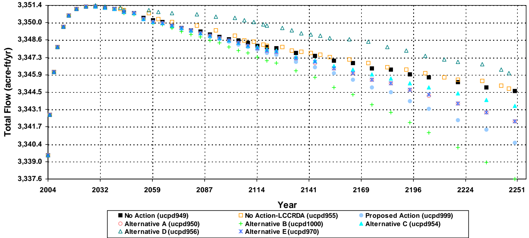
Simulated Stream / Spring Flow Changes at McGill Spring SPiw79_1
