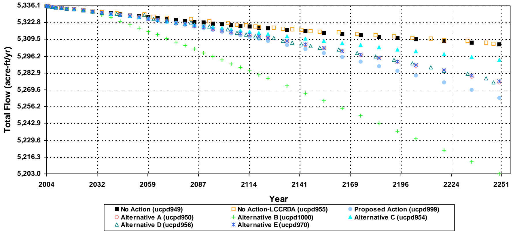
Simulated Stream / Spring Flow Changes at Lund Spring SPib07_5
