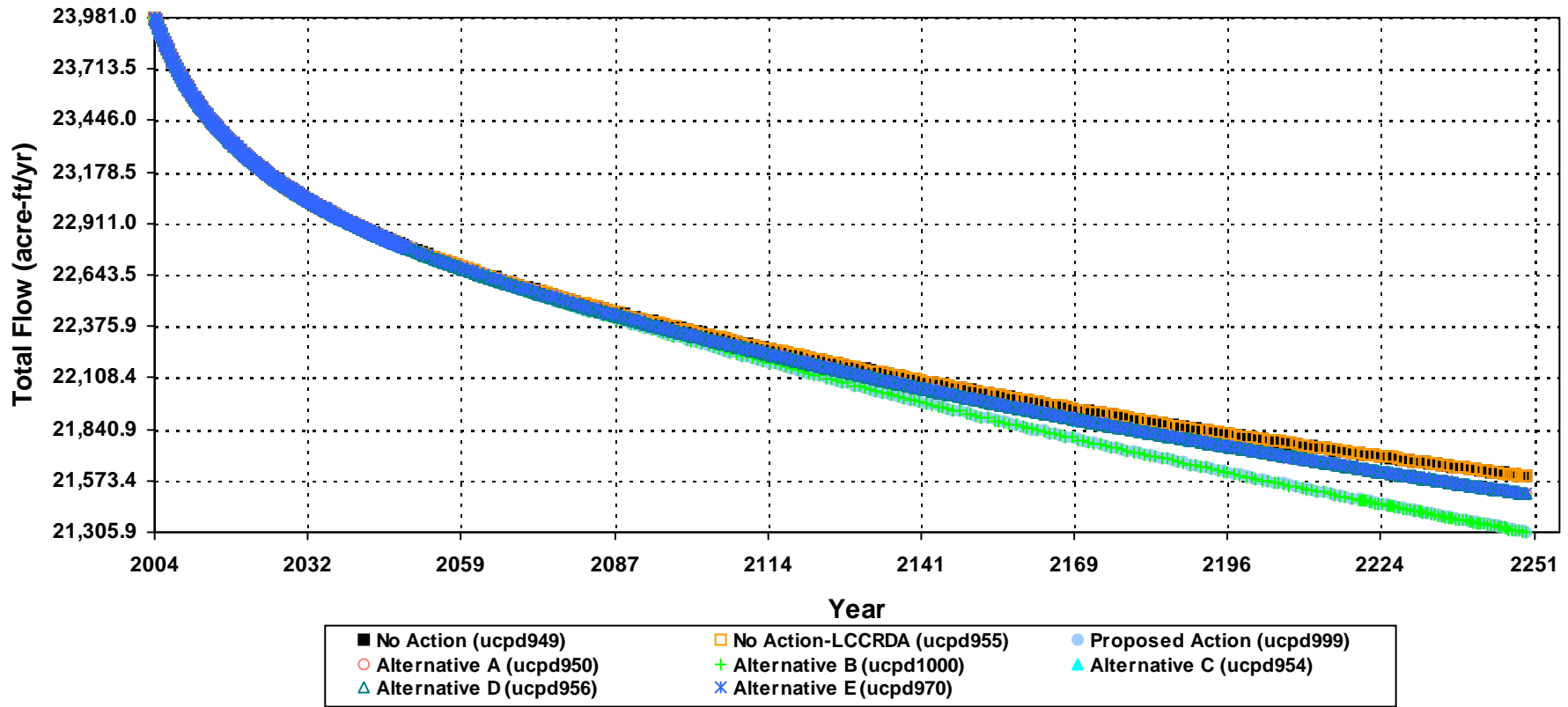
Simulated Stream / Spring Flow Changes at Muddy River near Glendale G_GLEND
