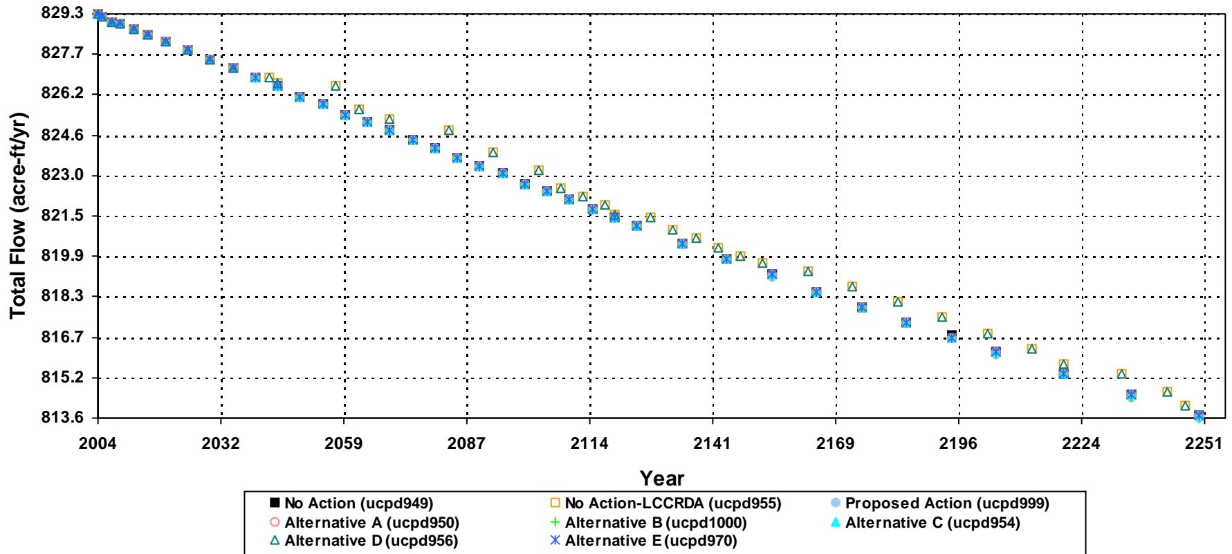
Simulated Stream / Spring Flow Changes at Rogers Spring SPiw15_1
