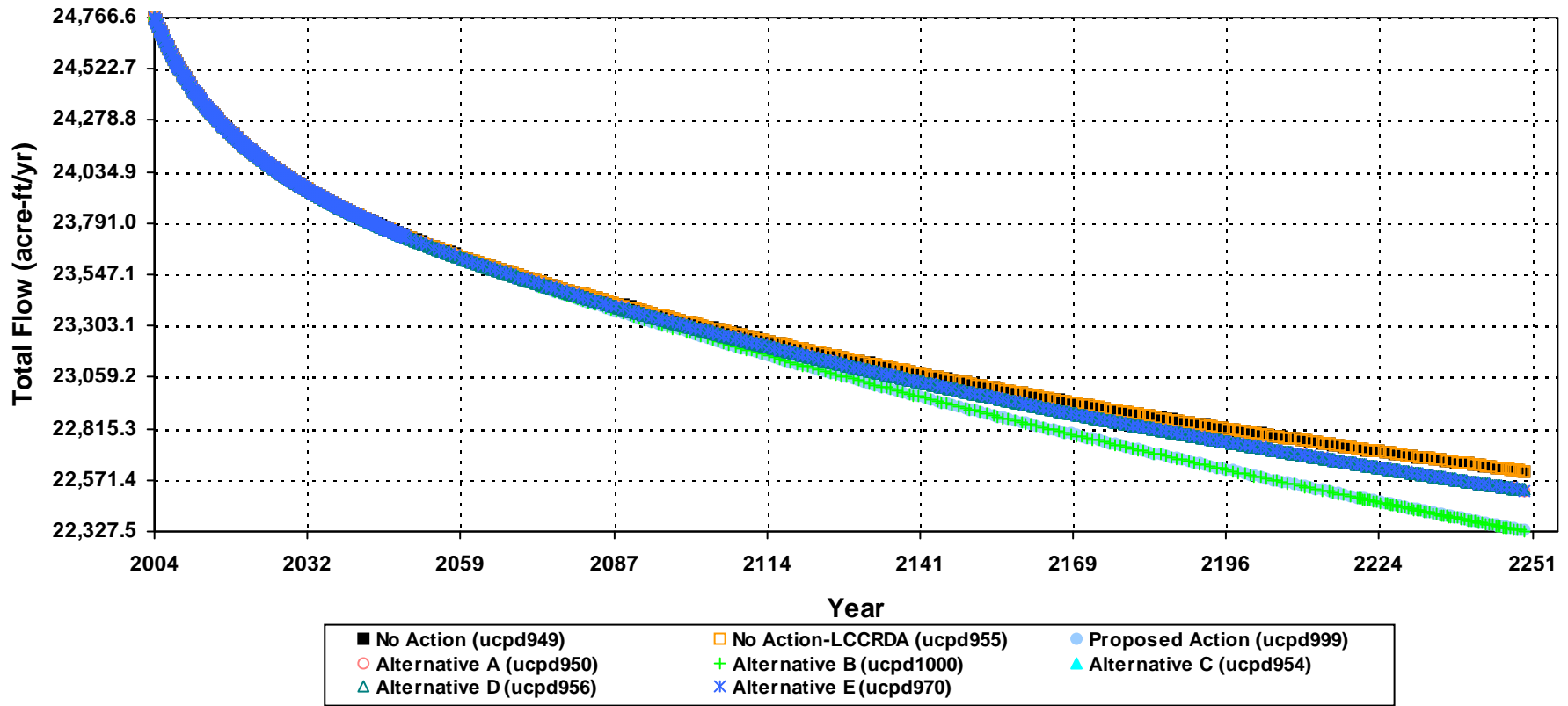
Simulated Stream / Spring Flow Changes at Muddy River near Moapa G_MOAPA
