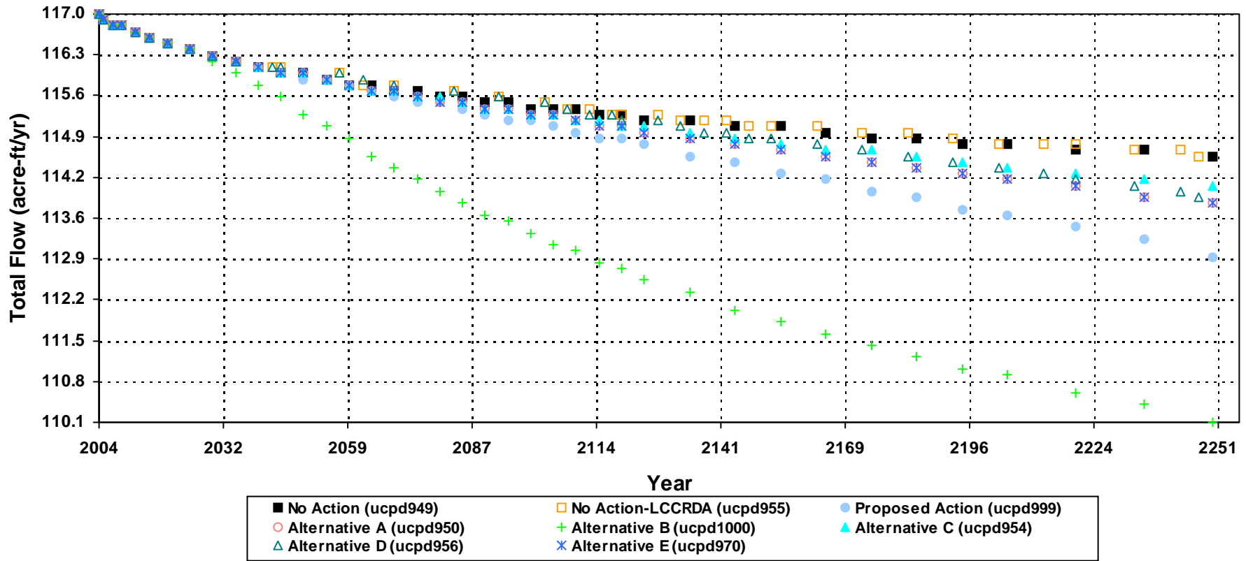
Simulated Stream / Spring Flow Changes at Hardy Springs
