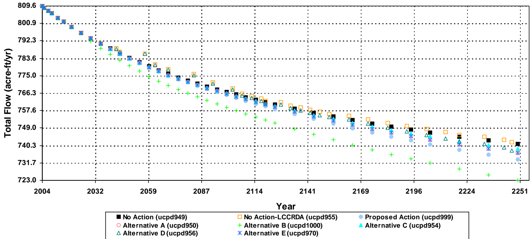
Simulated Stream / Spring Flow Changes at Cold Spring SPiw07_3
