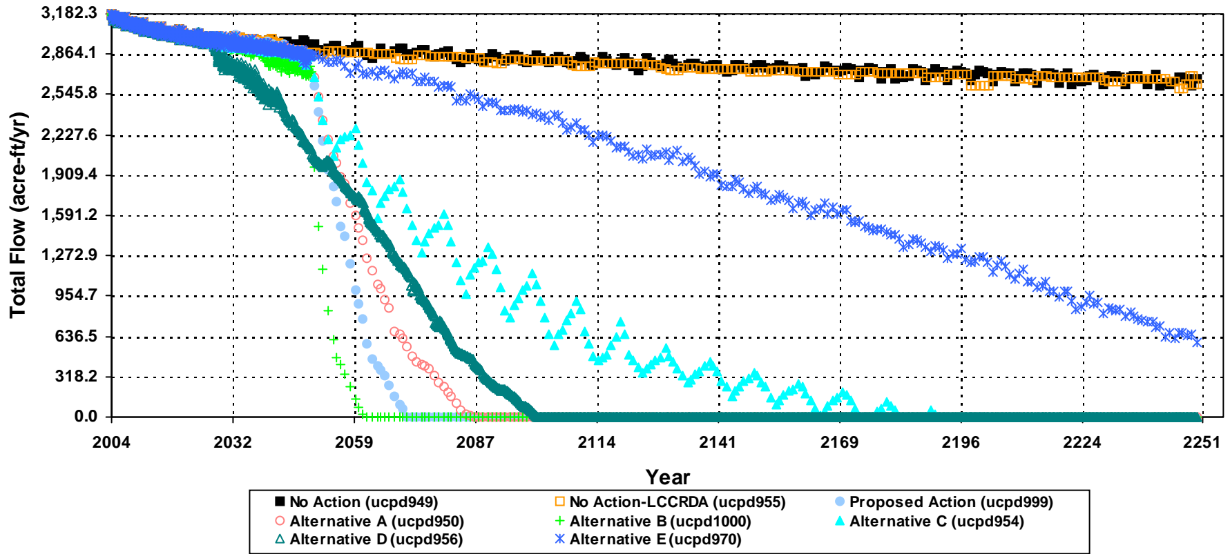
Simulated Stream / Spring Flow Changes at Big Springs G_BGSPR
