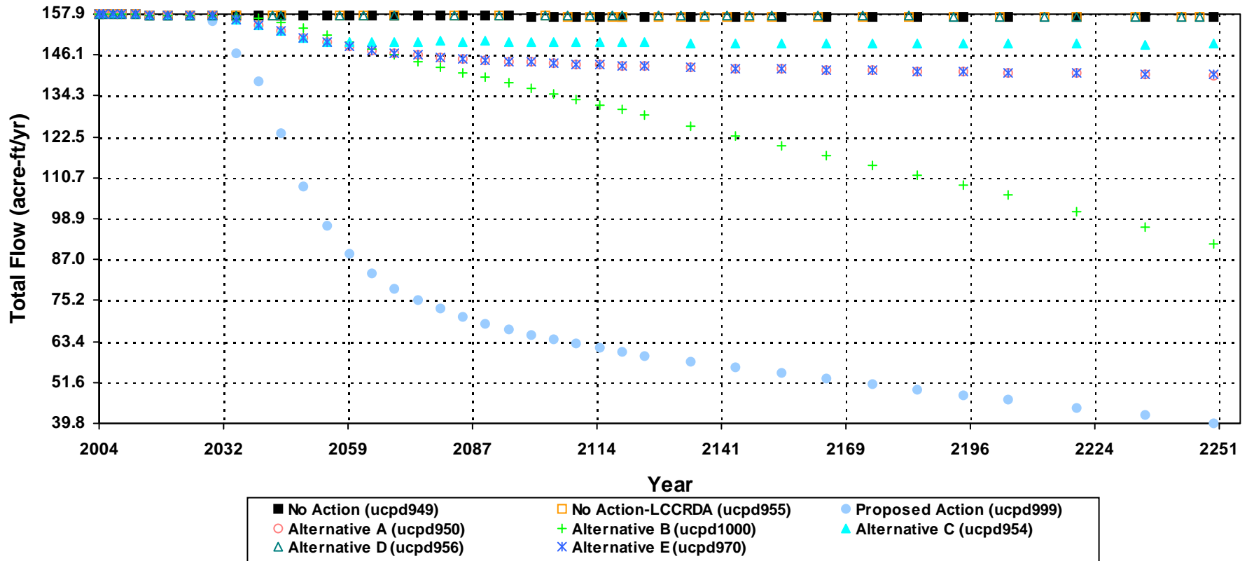
Simulated Stream / Spring Flow Changes at North Millick Spring
