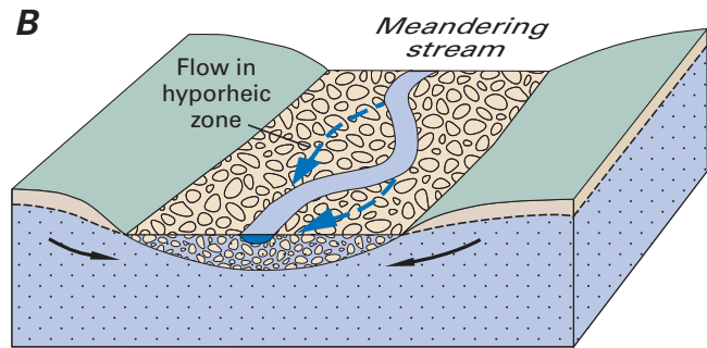
Figure 23. Surface-water exchange with ground water in the hyporheic zone is associated with abrupt changes in streambed slope (A) and with stream meanders (B).
