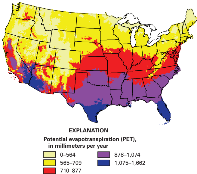
Figure 18. Annual potential evapotranspiration rates across the conterminous United States as calculated with the Hamon equation.
