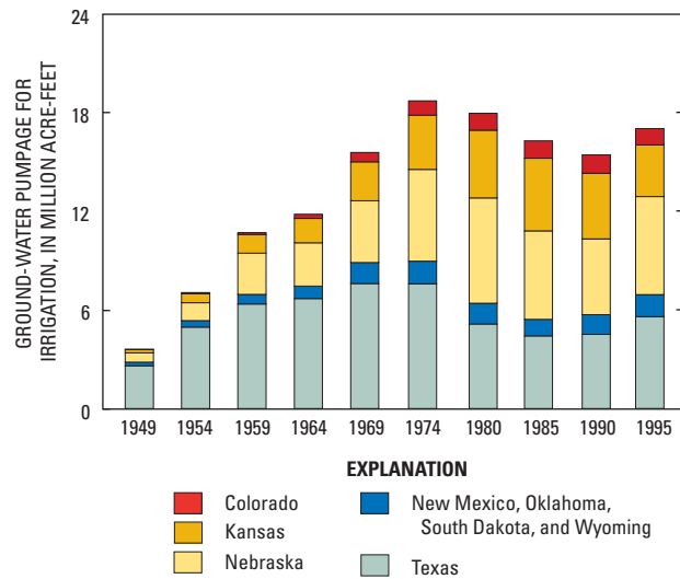
Figure 38. Ground-water pumpage from the High Plains aquifer for irrigation by State for selected years, 1949 to 1995 (McGuire and others, 2003).
