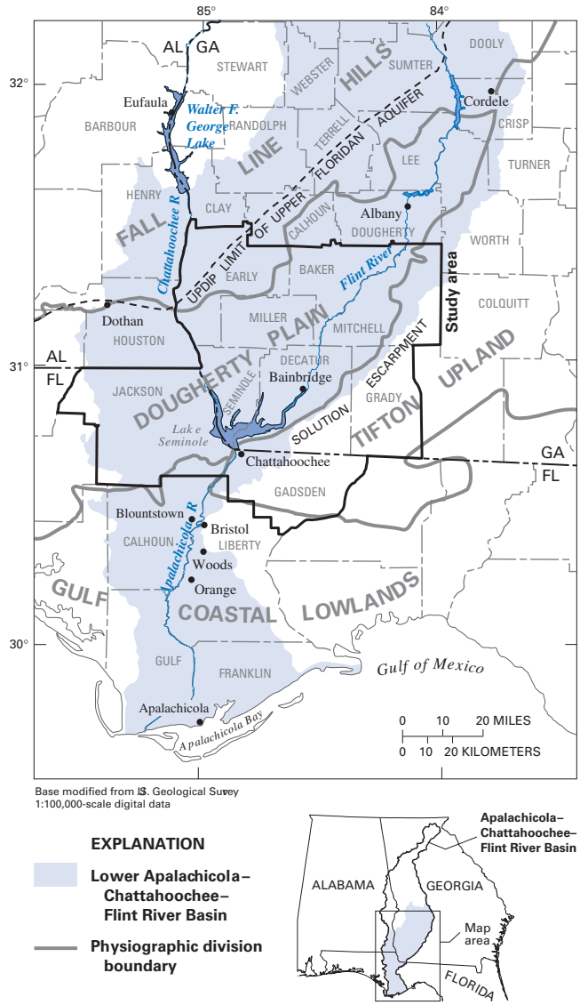
Figure 42. Location of Lake Seminole, boundaries of the lower Apalachicola-Chattahoochee-Flint River Basin, and physiographic divisions of the Coastal Plain Province in southeastern Alabama, northwestern Florida, and southwestern Georgia (Dalton and others, 2004).
