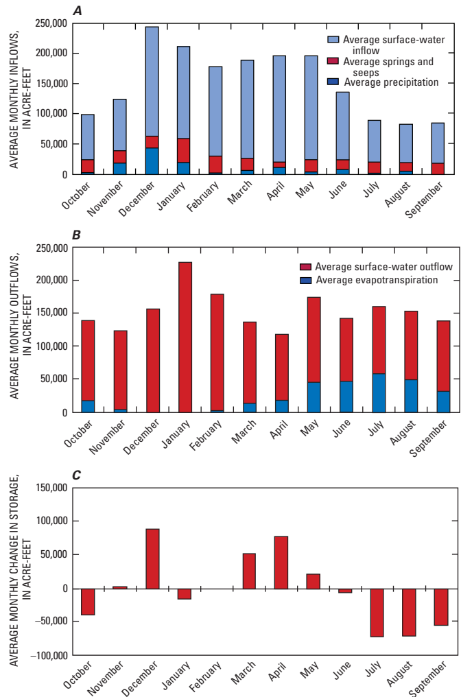
Figure 46. Average monthly water budget for Upper Klamath Lake for October 1964 through September 1967 (Hubbard, 1970): (A) Average monthly inflows, (B) average monthly outflows, and (C) average monthly change in storage.
