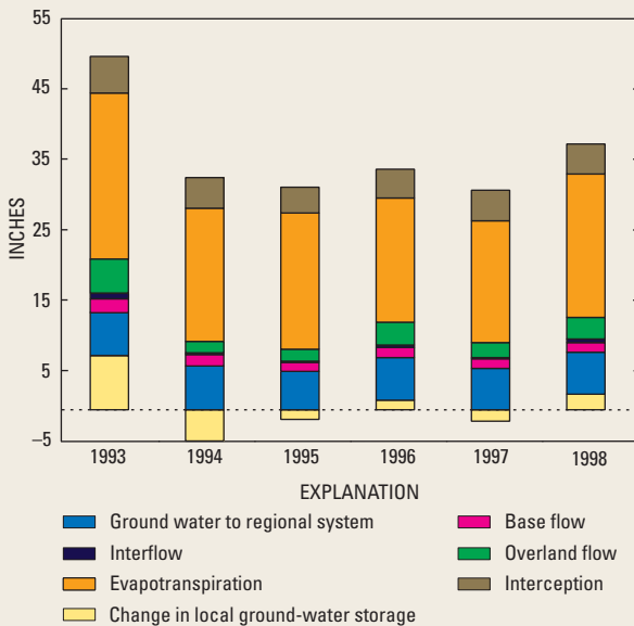
Figure D-2. Steuer and Hunt (2001) used a watershed model to simulate water fluxes in the Pheasant Branch Creek watershed near Middleton, Wisconsin, for the period 1993 to 1998. The model was subsequently used to predict the effects of urban development in the watershed.
