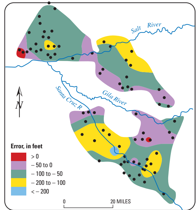
Figure 36. Map of central Arizona showing error in water levels predicted by a ground-water flow model (after Konikow, 1986). Errors are determined as predicted minus measured water levels. Location shown in figure 35.
