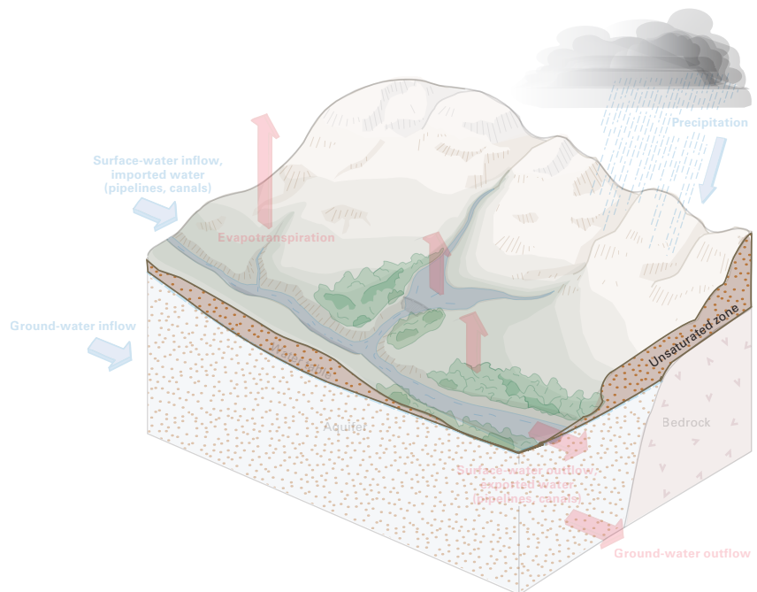
Figure 6. The unsaturated zone within the hydrologic cycle.
