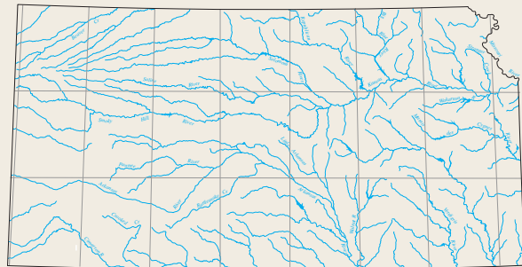
Figure J-2. Principal rivers, Kansas (Paulson and others, 1991).
