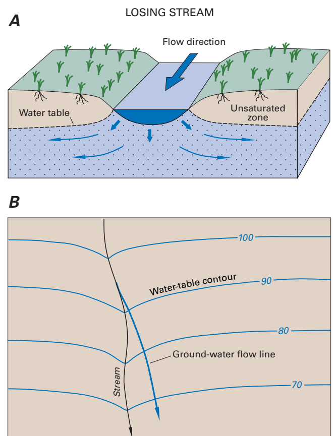
Figure 21. Losing streams lose water to the ground-water system (A). This can be determined from water-table contour maps because the contour lines point in the downstream direction where they cross the stream (B).
