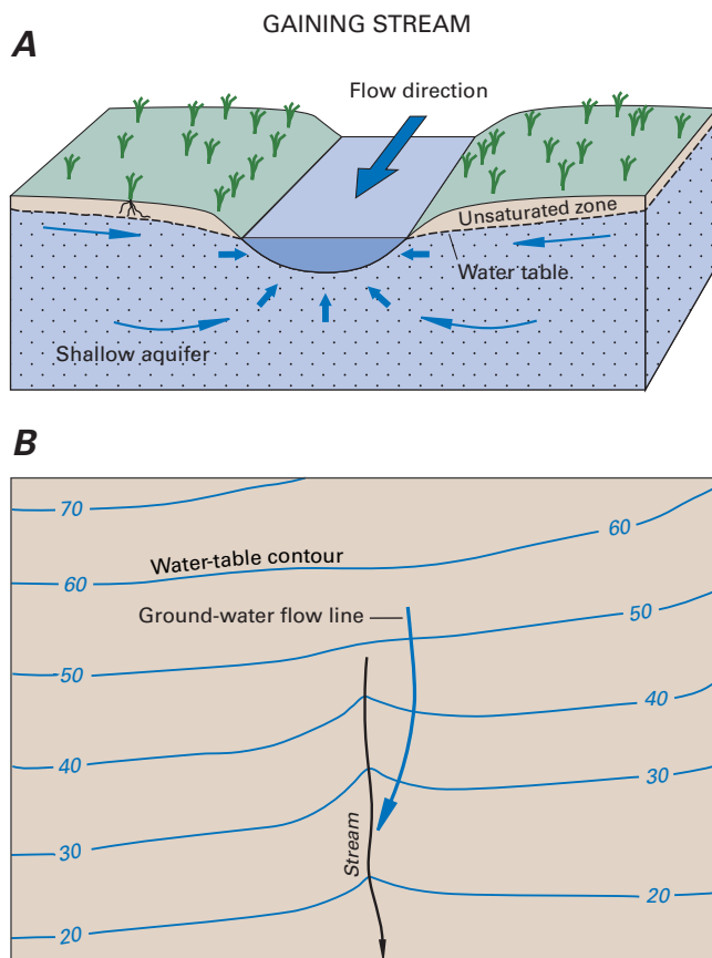
Figure 20. Gaining streams receive water from the ground-water system (A). This can be determined from water-table contour maps because the contour lines point in the upstream direction where they cross the stream (B).
