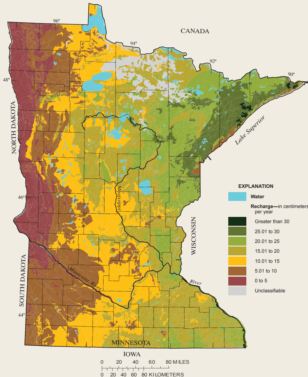
Figure F-1. Estimated annual rates of recharge in Minnesota (Lorenz and Delin, 2007).
