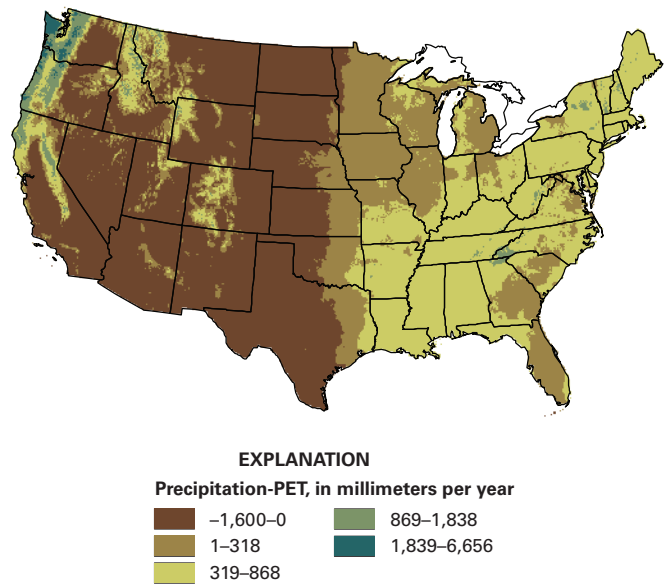
Figure 19. Difference between annual precipitation and potential evapotranspiration rates across the conterminous United States.
