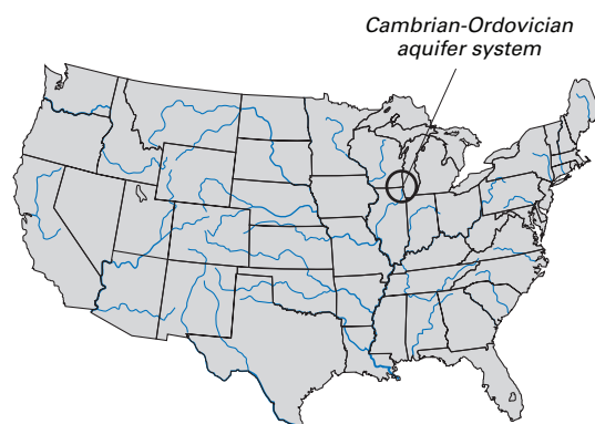
Figure 49. Approximate location map of Cambrian-Ordovician-age aquifer system in northern Illinois and southern Wisconsin.
