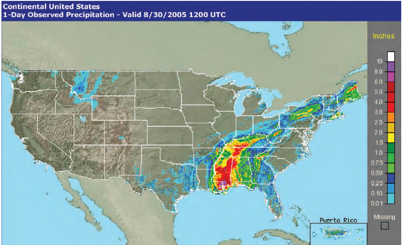
Figure 16. Daily rainfall for August 30, 2005 on a 4-kilometer spatial grid as determined by the National Weather Service MPE program. (National Weather Service, http://www.srh.noaa.gov/rfcshare/precip_analysis_new.php accessed on Feb. 13, 2007)
