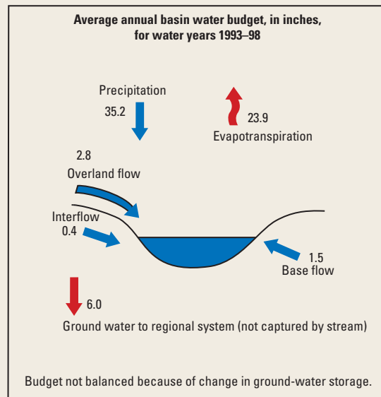
Figure D-2. Steuer and Hunt (2001) used a watershed model to simulate water fluxes in the Pheasant Branch Creek watershed near Middleton, Wisconsin, for the period 1993 to 1998. The model was subsequently used to predict the effects of urban development in the watershed.
