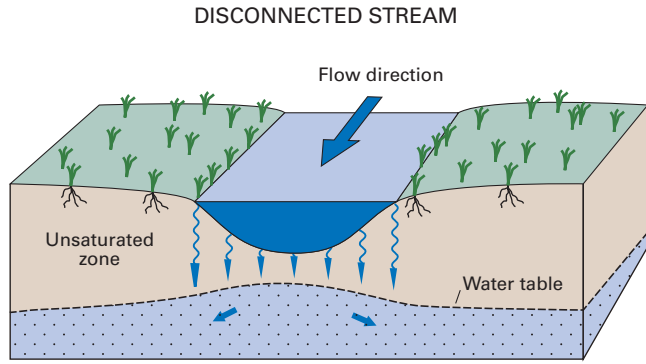
Figure 22. Disconnected streams are separated from the water table by an unsaturated zone.
