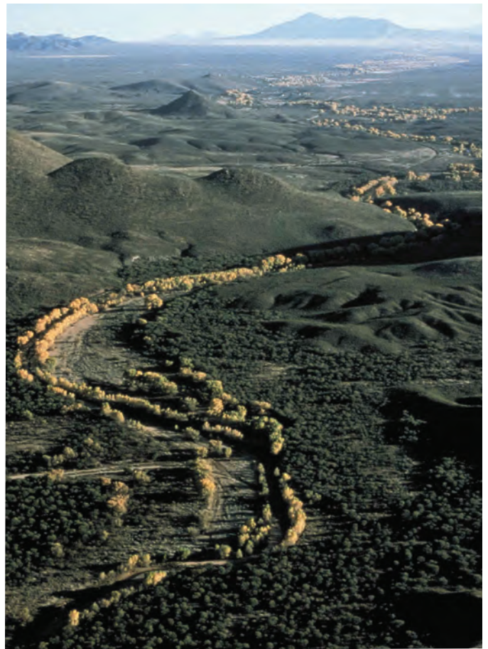
The San Pedro River flows northward from the Mexican State of Sonora into Arizona.
