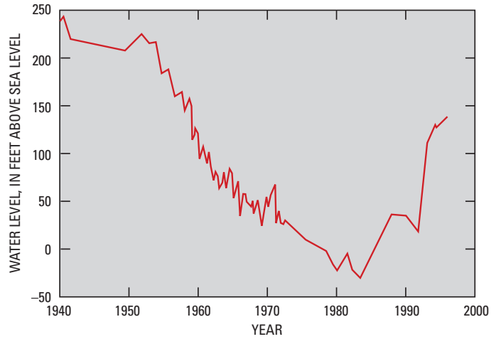
Figure 52. Trends in ground-water levels in the deep Cambrian-Ordovician aquifer system. Data are from a well in Cook County near Chicago (after Visocky, 1997).
