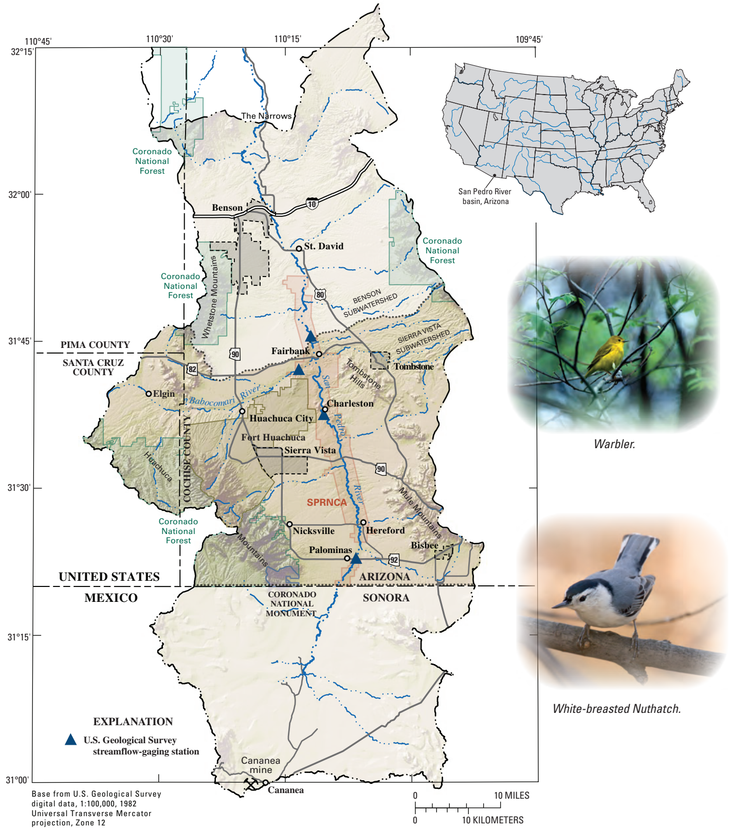
Figure 47. Location of the upper San Pedro River basin showing the San Pedro Riparian National Conservation Area (SPRNCA).
