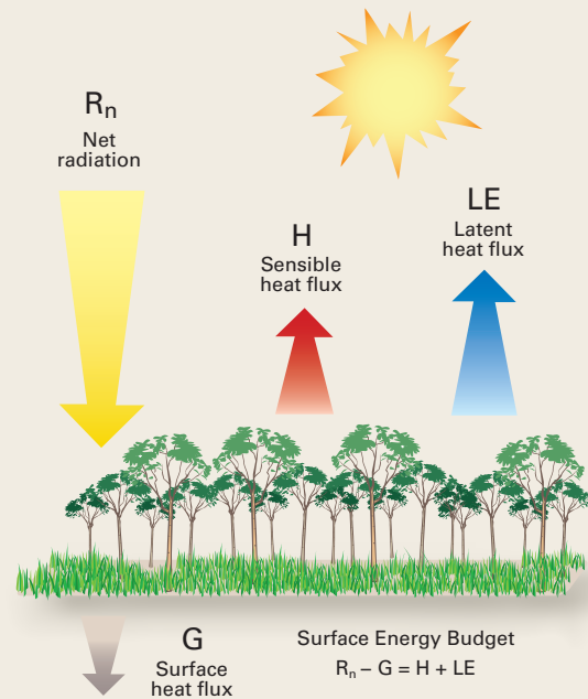
Figure B-1. Schematic of the energy budget at the Earth's surface.
