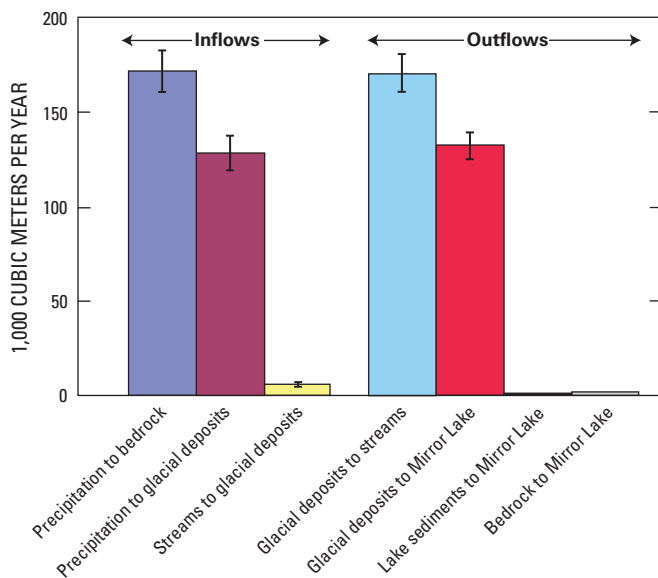
Figure 32. Model calculated water budget for the Mirror Lake ground-water basin from Tiedeman and others (1997). Error bars indicate approximate 95-percent confidence interval.
