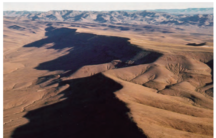
The unsaturated zone at Yucca Mountain, Nevada is as thick as 500 meters.
