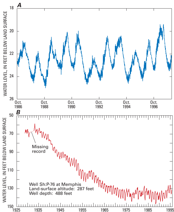
Figure 10. (A) Hydrograph of daily water-level measurements over a 10-year period for a well in Vanderburgh County, Indiana; and (B) water-level trends in a long-term observation well in Memphis, Tennessee (Taylor and Alley, 2001).
