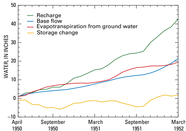
Figure 28. Ground-water budget for Beaverdam Creek Basin, April 1950 to March 1952.
