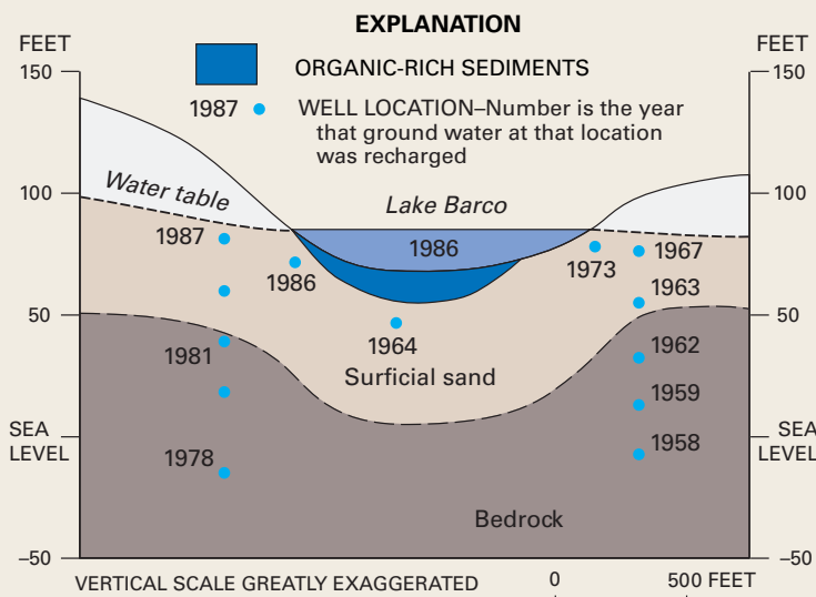
Figure C-2. Lake Barco, in northern Florida, is a flow-through lake with respect to ground water. The dates when water in different parts of the ground-water system was recharged indicate how long it takes water to move from the lake or the water table to a given depth (after Katz and others, 1995).
