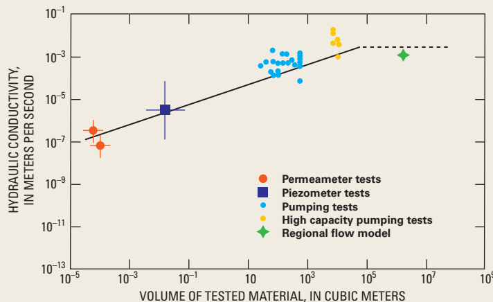
Figure G-2. Hydraulic conductivity as a function of sample size (after Schulze-Makuch and others, 1999).
