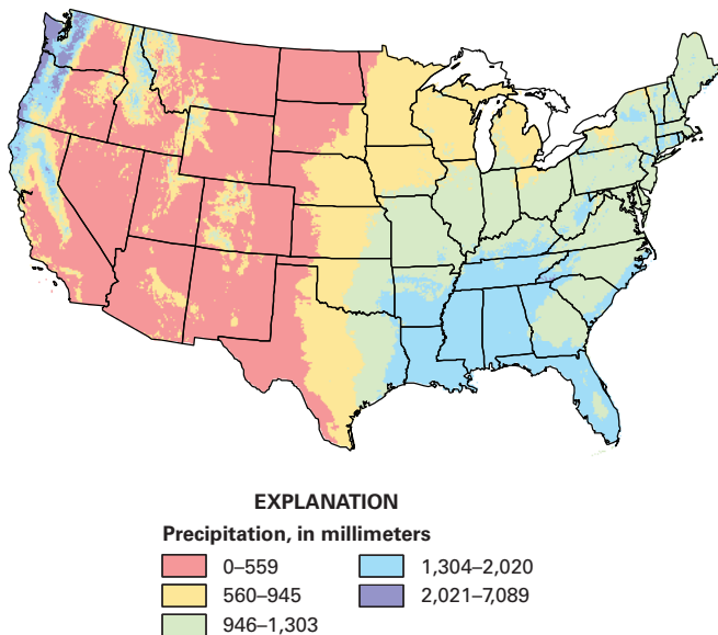
Figure 14. Average annual precipitation in the conterminous United States for the period 1980–1997 as determined by the DAYMET model ( http://www.daymet.org ).
