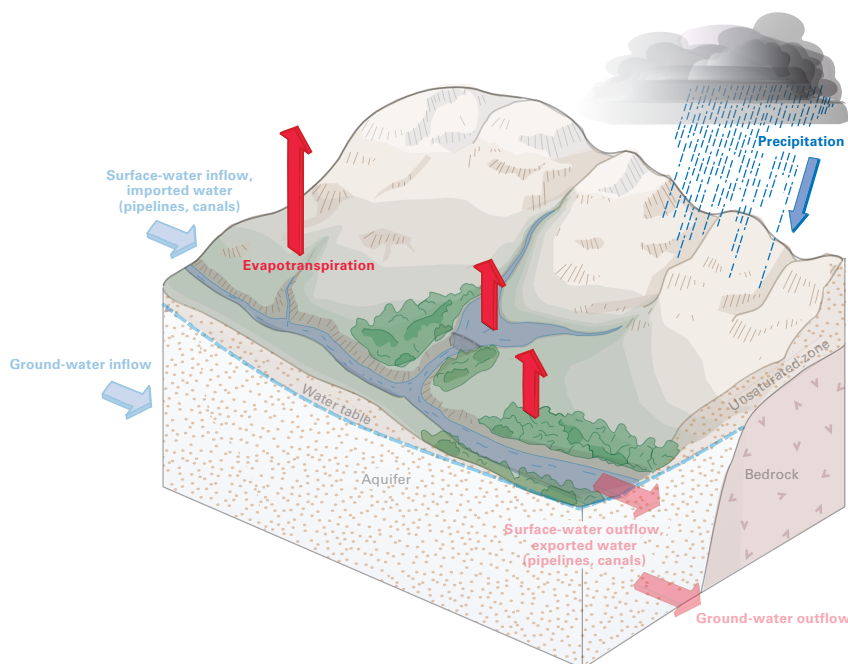
Figure 2. The atmosphere within the hydrologic cycle.
