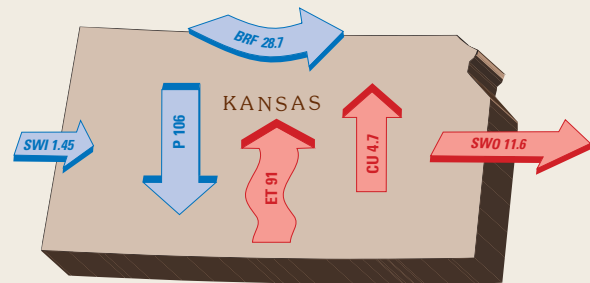
Figure J-1. Average-annual water budget for Kansas, in million gallons per day, 1970s and early 1980s. Abbreviations: BRF, boundary-river flow; CU, consumptive use (evapotranspiration related to human activities, mostly irrigation); ET, evapotranspiration from native plants and nonirrigated agricultural fields; P, precipitation; SWI, surface-water inflow; SWO, surface-water outflow (Carr and others, 1990).
