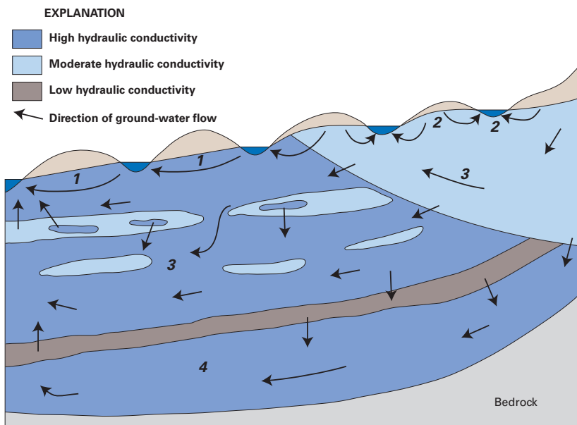
Figure 9. Ground-water flow systems in complex geological terrain. Ground water in the uppermost part of the ground-water system flows from surface-water body to surface-water body in the high hydraulic conductivity zone (characteristic of glacial outwash) because the water table slopes uniformly from one to the other (1). However, where the hydraulic conductivity of the deposits is lower (characteristic of glacial till), water-table mounds beneath the land-surface highs cause the local flow systems to discharge to contiguous surface-water bodies, such that there is no flow from one surface-water body to the next lower surface-water body (2). In both settings, intermediate-scale ground-water flow systems pass at depth beneath the local flow systems (3), and a regional ground-water flow system passes at depth beneath both local and intermediate flow systems (4).
