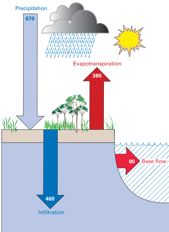
Figure 13. Average annual water exchange rates for North America (from Lvovitch, 1973) in millimeters of depth per unit area of land surface.
