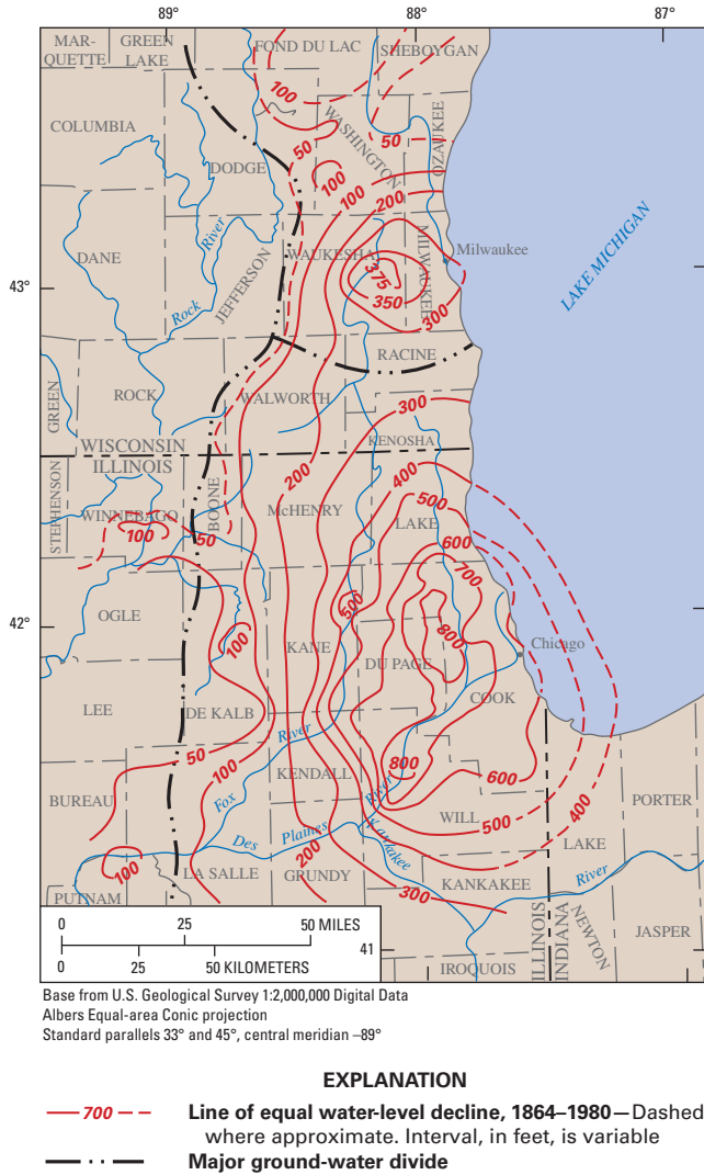
Figure 51. Ground-water level declines from 1864 to 1980 in the Cambrian-Ordovician aquifer system, Chicago and Milwaukee areas (Alley and others, 1999).
