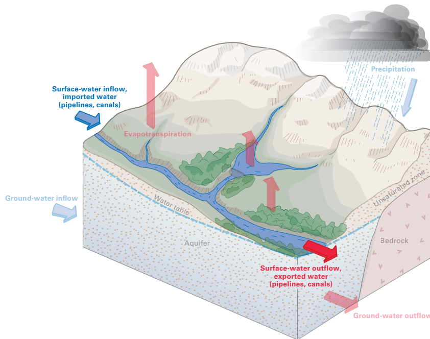
Figure 4. Lakes, wetlands, and streams within the hydrologic cycle.
