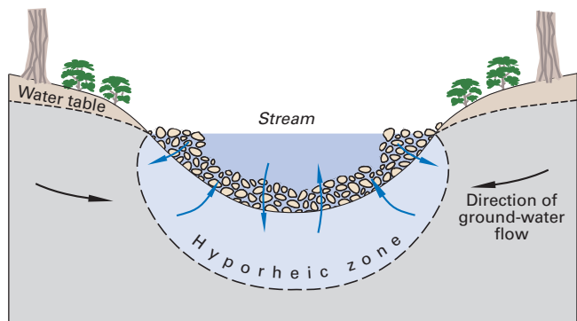
Figure 24. Streambeds and banks are unique environments because they are where ground water that drains much of the subsurface of landscapes interacts with surface water that drains much of the surface of landscapes.
