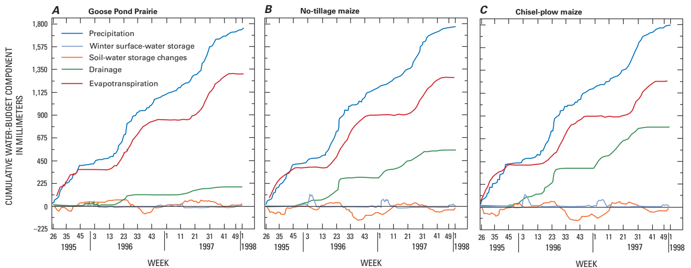
Figure 30. Water budget for (A) prairie site; (B) no-tillage maize site; and (C) chisel-plow maize site in central Wisconsin (Brye and others, 2000). Imbalance in the water budgets is attributed to runoff for the prairie and no-tillage site and to runoff from melting snow at the chisel-plow site.
