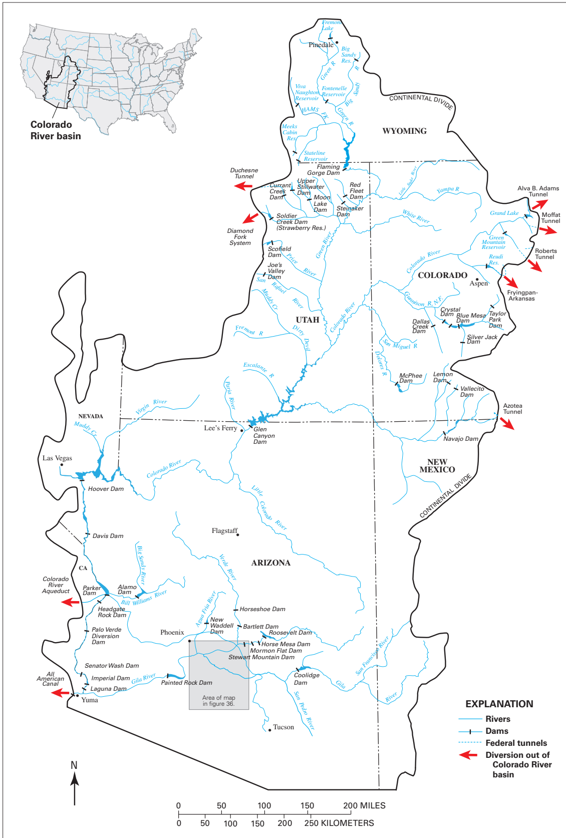
Figure 35. Map of the Colorado River basin showing locations of major surface-water reservoirs and diversions.
