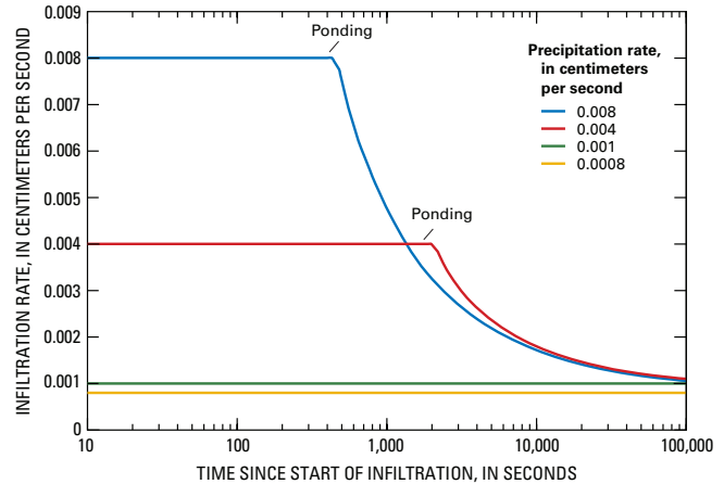
Figure 17. Infiltration rates generated for a one-dimensional uniform soil column with a variably saturated flow model as a function of time for four precipitation rates. The saturated hydraulic conductivity of the soil is 0.001 centimeter per second.
