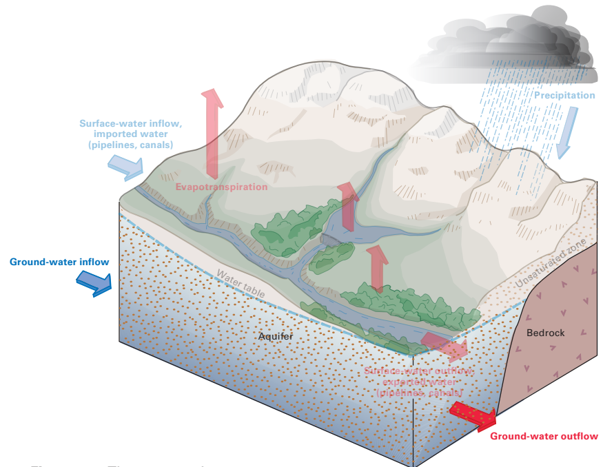
Figure 8. The saturated zone within the hydrologic cycle.
