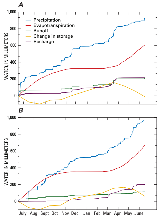
Figure 34. Water-budget components for (A) July 1982 through June 1983 and (B) July 1983 through June 1984 for a site in northwestern Illinois (Healy and others, 1989b).
