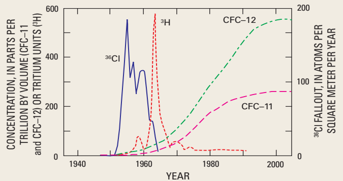
Figure C-1. Atmospheric concentrations for historical tracers, including ^3\text{H} , ^{36}\text{Cl} , CFC-11, and CFC-12 (after Scanlon and others, 2002).
