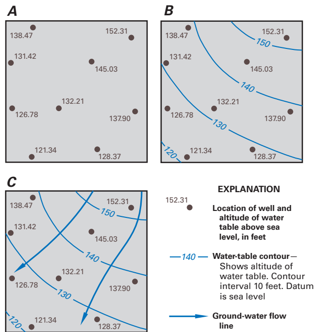
Figure 11. By using known altitudes of the water table at individual wells (A), contour maps of the water-table surface can be drawn (B), and directions of ground-water flow along the water table can be determined (C) because flow usually is approximately perpendicular to the contours (Winter and others, 1998).
