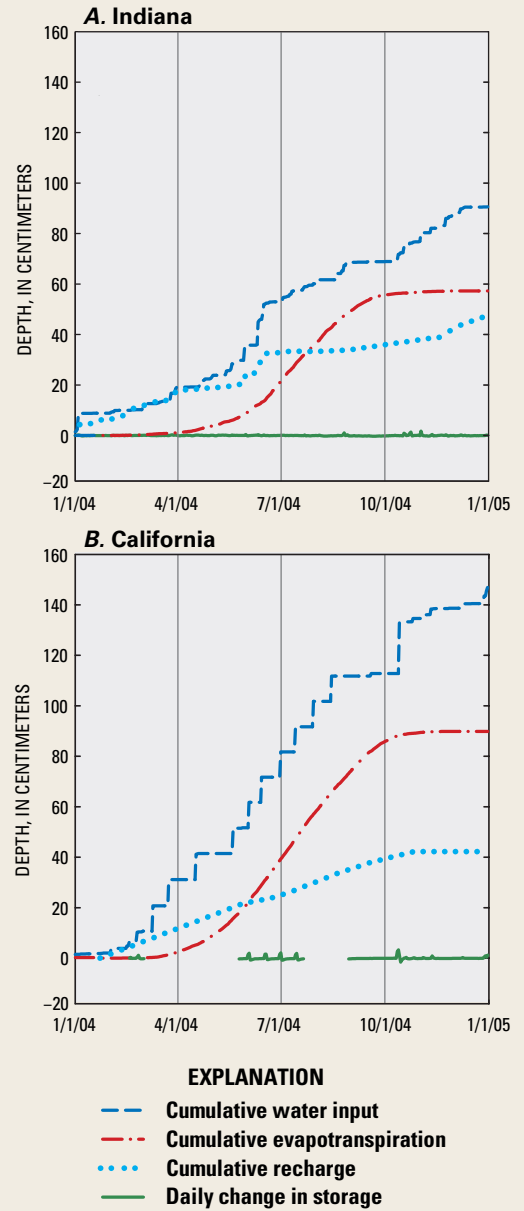
Figure F-2. Water budgets for (A) an unirrigated agricultural field in central Indiana, where most recharge occurs in winter and spring, and (B) an irrigated agricultural field in central California, where most recharge occurs during the growing season (after Fisher and Healy, 2007). Water input refers to the sum of precipitation and irrigation.
