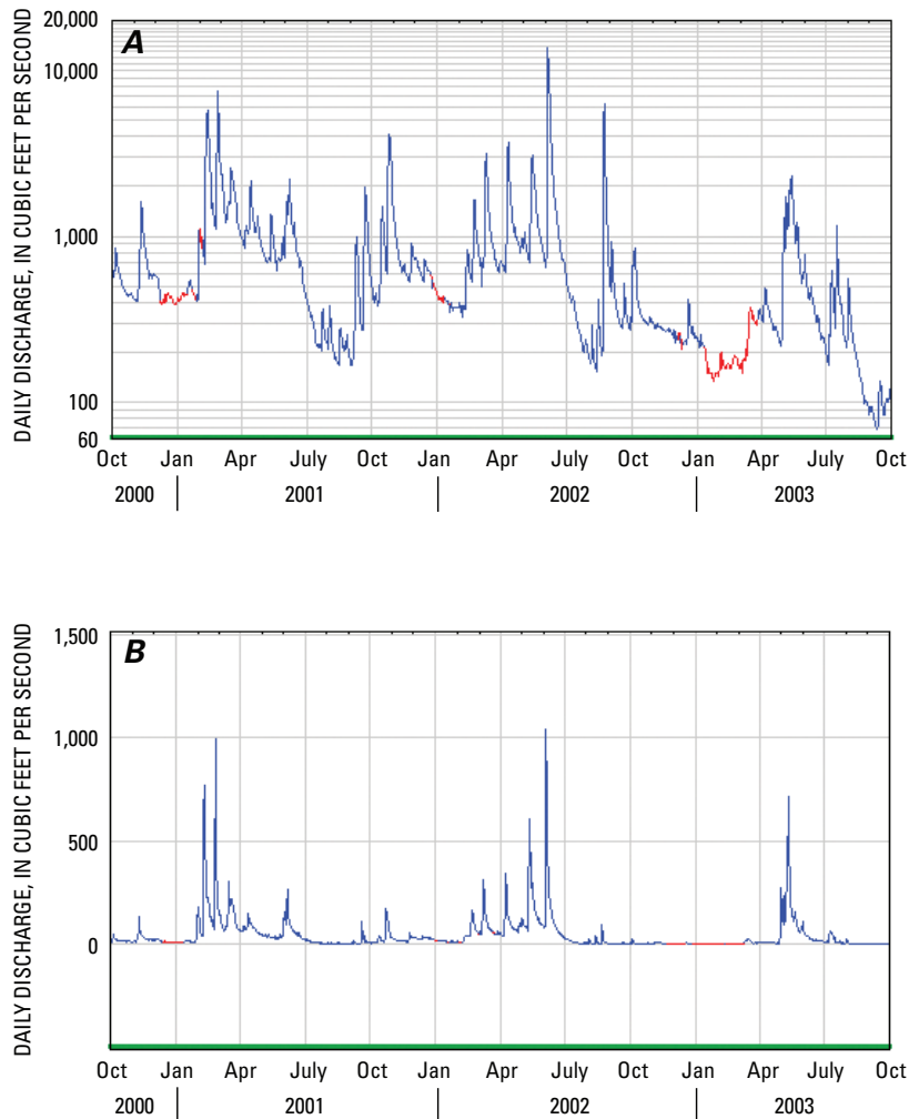
Figure 5. Streamflow hydrographs for two gaging sites: (A) Kishwaukee River near Perryville, Illinois (U.S. Geological Survey station number 05440000; drainage area 1,099 square miles) and (B) South Branch Kishwaukee River at DeKalb, Illinois (U.S. Geological Survey station number 05439000; drainage area 77.7 square miles). Red indicates estimated values.
