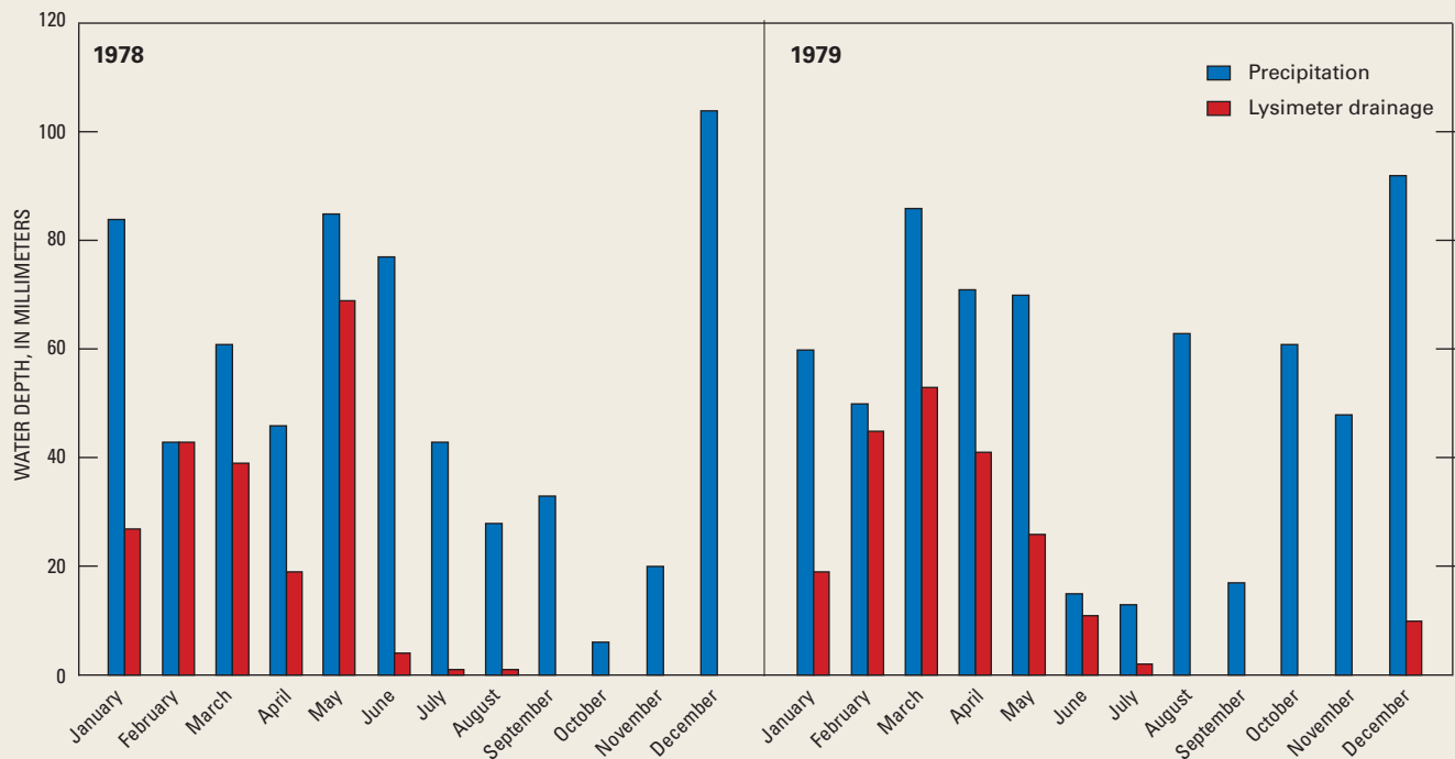
Figure E-1. Monthly rainfall and drainage from lysimeter at Fleam Dyke (Kitching and Shearer, 1982).
