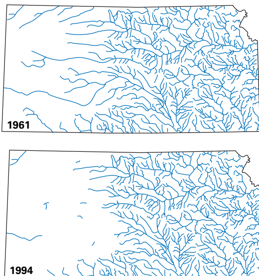
Figure 41. Major perennial streams in Kansas, 1961 and 1994. Parts of the High Plains aquifer occur in western Kansas where stream channels exhibiting perennial flow have been reduced in length (after Sophocleous, 2000).
