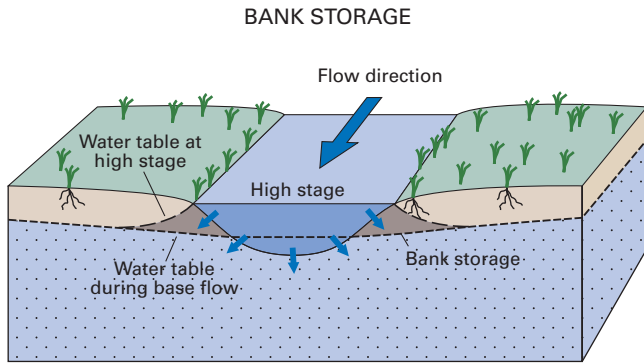
Figure 25. If stream levels rise higher than adjacent groundwater levels, stream water moves into the streambanks as bank storage.
