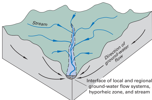
Figure 24. Streambeds and banks are unique environments because they are where ground water that drains much of the subsurface of landscapes interacts with surface water that drains much of the surface of landscapes.
