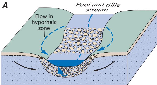
Figure 23. Surface-water exchange with ground water in the hyporheic zone is associated with abrupt changes in streambed slope (A) and with stream meanders (B).
