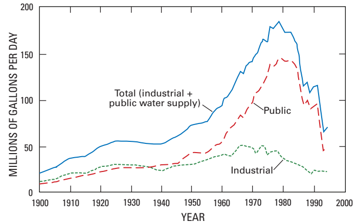
Figure 50. Ground-water withdrawals from the Cambrian-Ordovician aquifer system in the eight-county Chicago area, 1900–94 (Visocky, 1997).
