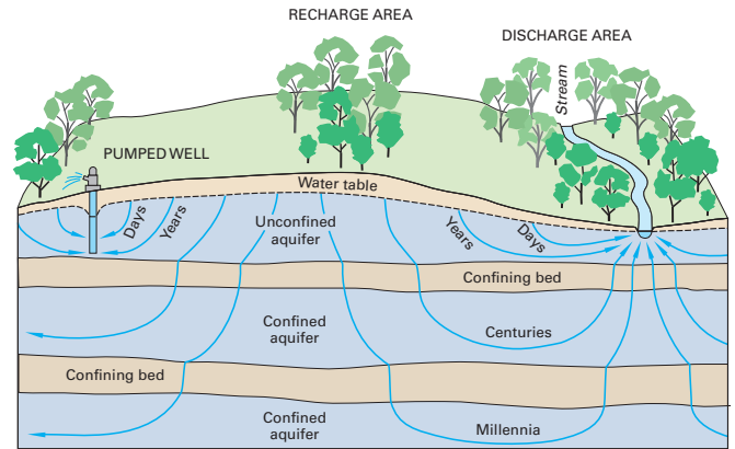
Figure 12. Ground-water flow paths vary greatly in length, depth, and traveltime from points of recharge to points of discharge in the ground-water system.
