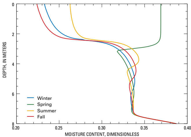
Figure 7. Hypothetical moisture-content profiles at four different times of the year. As depth increases, the variation in moisture content decreases.
