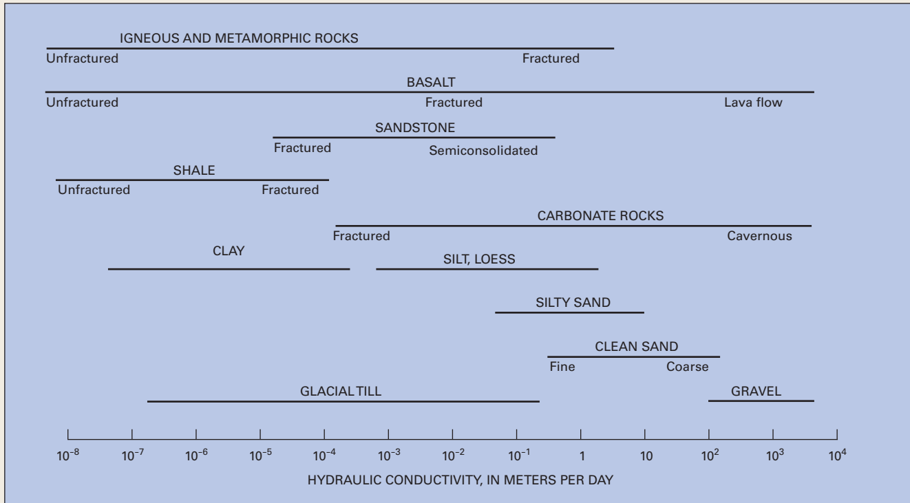
Figure G-1. Approximate ranges in hydraulic conductivity for selected earth materials. A total range of 13 orders of magnitude is shown, which is indicative of the range for more common earth materials. In general, the average hydraulic conductivity of earth material in the same hydrogeologic terrain can vary by orders of magnitude (after Heath, 1983).
