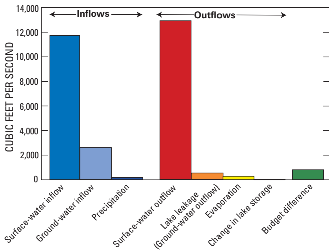
Figure 44. Average monthly water budget for Lake Seminole for the period April 2000 through September 2001 (Dalton and others, 2004).
