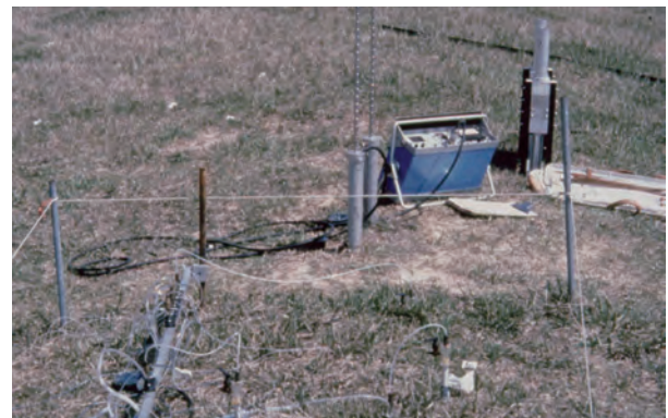
Soil moisture content and pressure head were measured.
