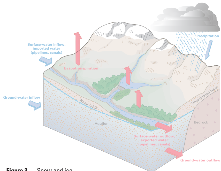
Figure 3. Snow and ice within the hydrologic cycle.
