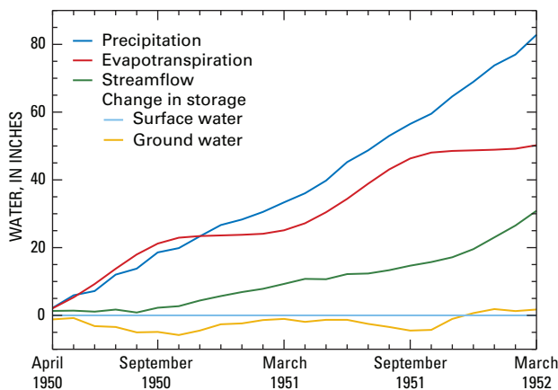
Figure 27. Water budget for Beaverdam Creek Basin, April 1950 to March 1952.
