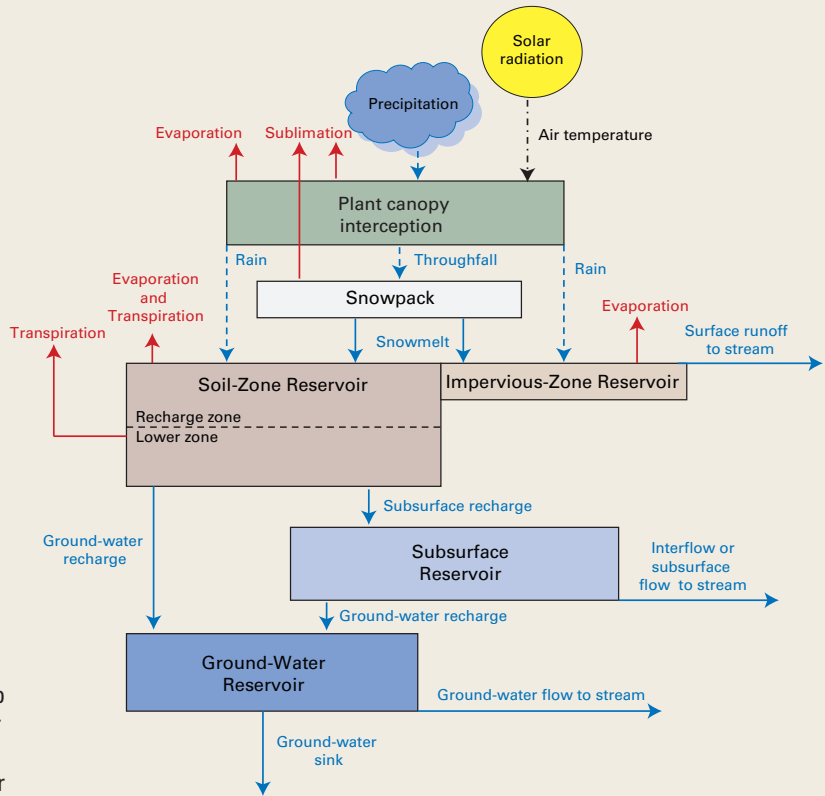
Figure D-1. Schematic diagram showing various reservoirs and processes that are considered in a watershed model (R.S. Regan, written commun., 2007).
