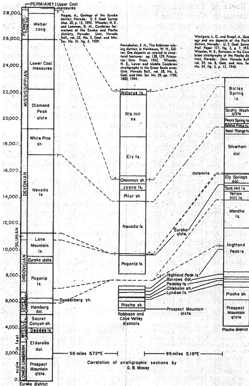
FIGURE 3—Diagrammatic correlation of Paleozoic stratigraphic columns in the Eureka, Pioche, and Robinson mining districts, and Cave Valley, Nevada.
