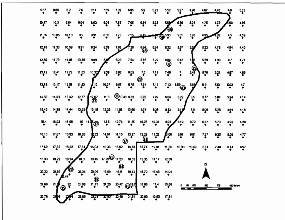
Figure 12. Map of the parcel IND 111 showing percent total perennial cover (circles) and estimated DTW (in feet) in 2001.
