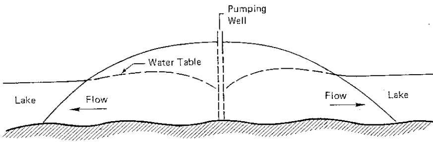
FIGURE 4.4 Cross section of the island aquifer system when the influence of pumping has reached the shoreline.
