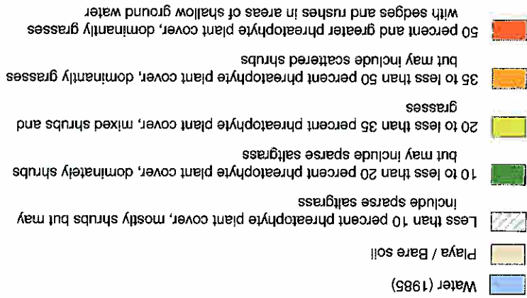
Figure B3. Estimated phreatophyte plant cover in Upper Fish Lake area, Little Fish Lake Valley, Nevada, 1985.
