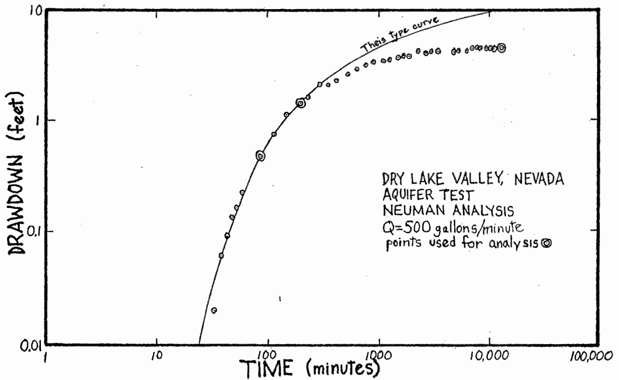
Figure 6. Log-log graph of drawdown vs. time for deep piezometer.
