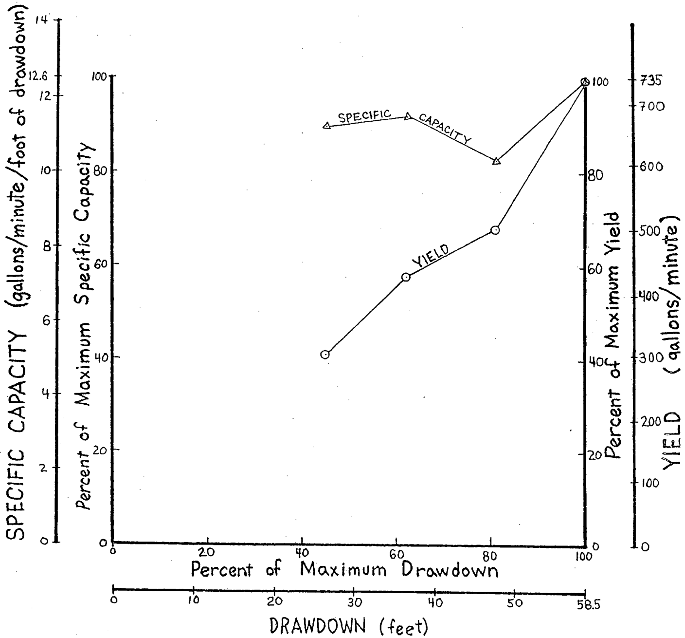
Figure 2. Specific capacity and yield during step-drawdown test.
