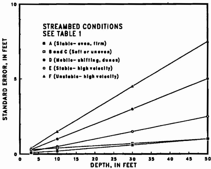
Figure 2.--Relation between depth and standard error for individual depth measurements made using a cable suspension system.
