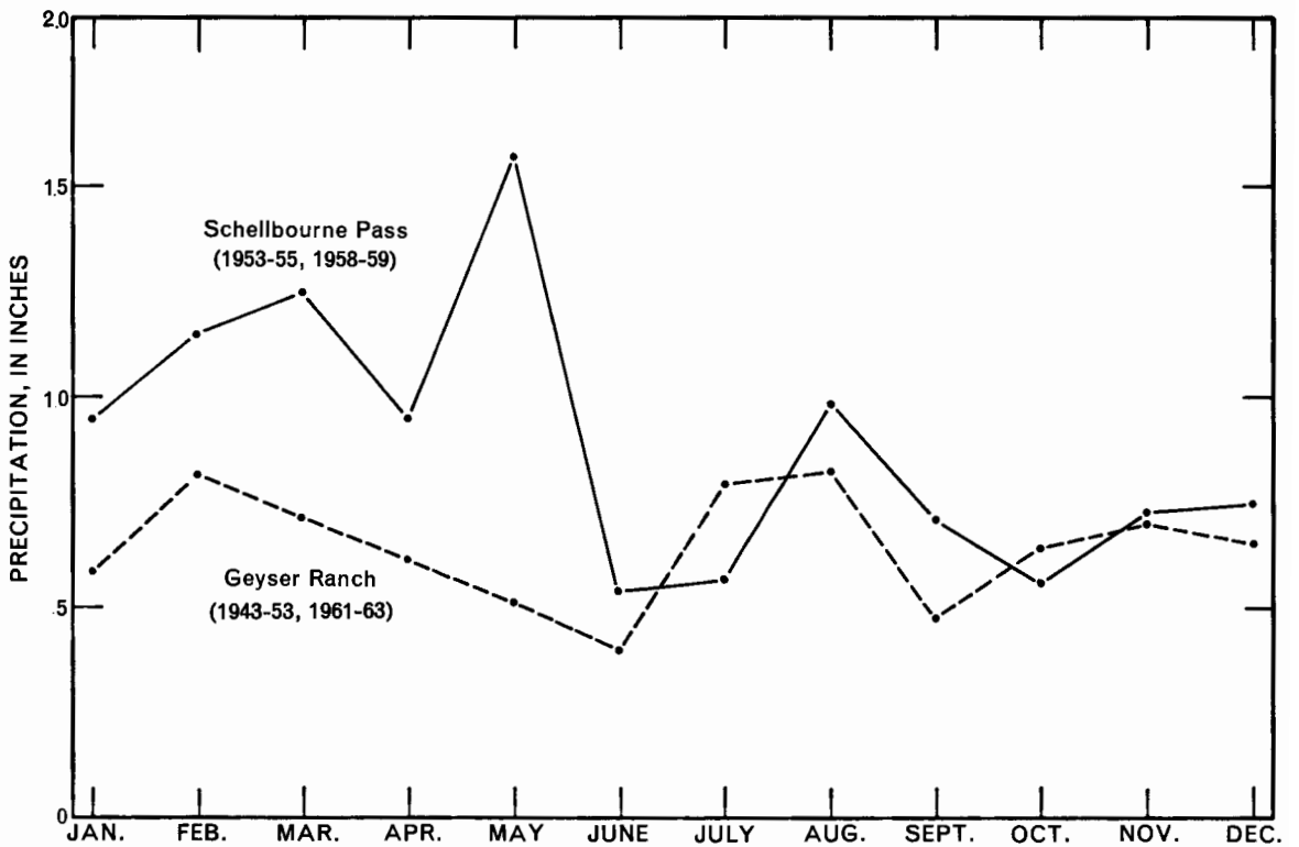
Figure 4.— Graph of average monthly precipitation at Shellbourne Pass and Geyser Ranch
