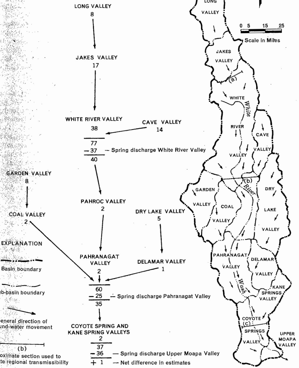
Fig. 6. Generalized flow pattern and estimated average annual recharge to and discharge from the regional groundwater system.
