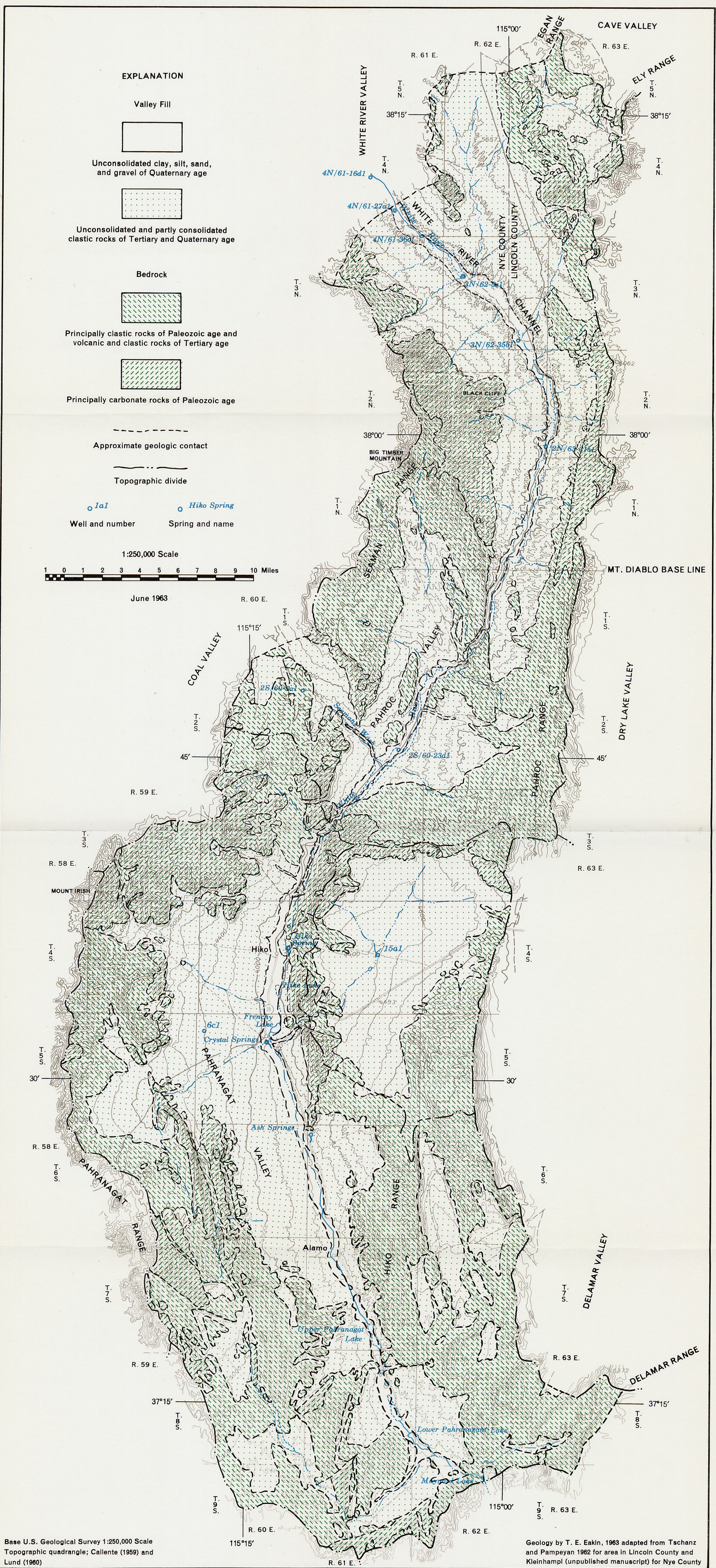
PLATE 1.—MAP OF THE PAHRANAGAT AND PAHROC VALLEYS, LINCOLN AND NYE COUNTIES, NEVADA SHOWING AREAS OF BEDROCK, VALLEY FILL, AND LOCATION OF SELECTED WELLS
