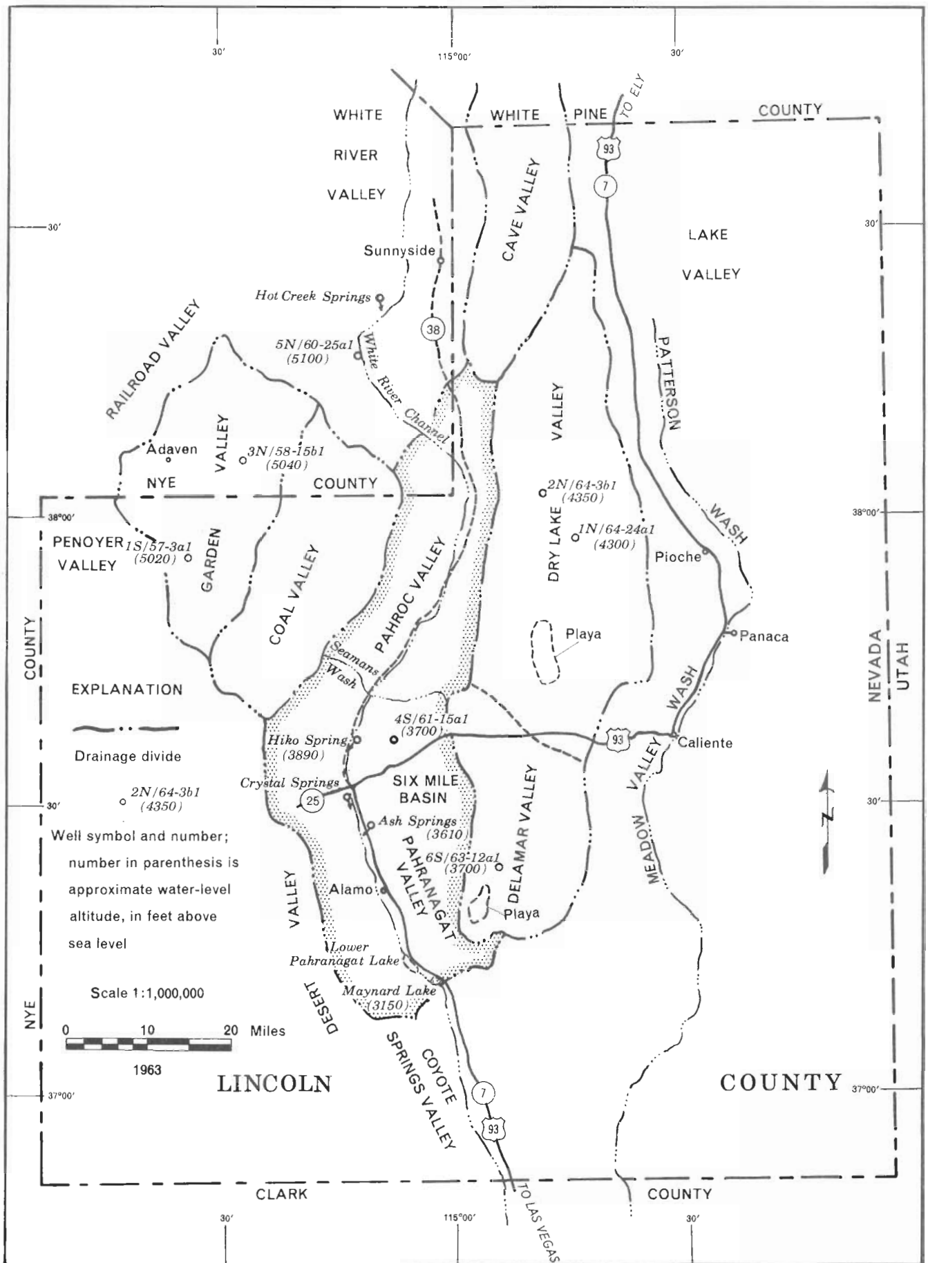
FIGURE 4. Sketch map showing relation of Pahrancagat and Pahrroc Valleys to adjacent areas
