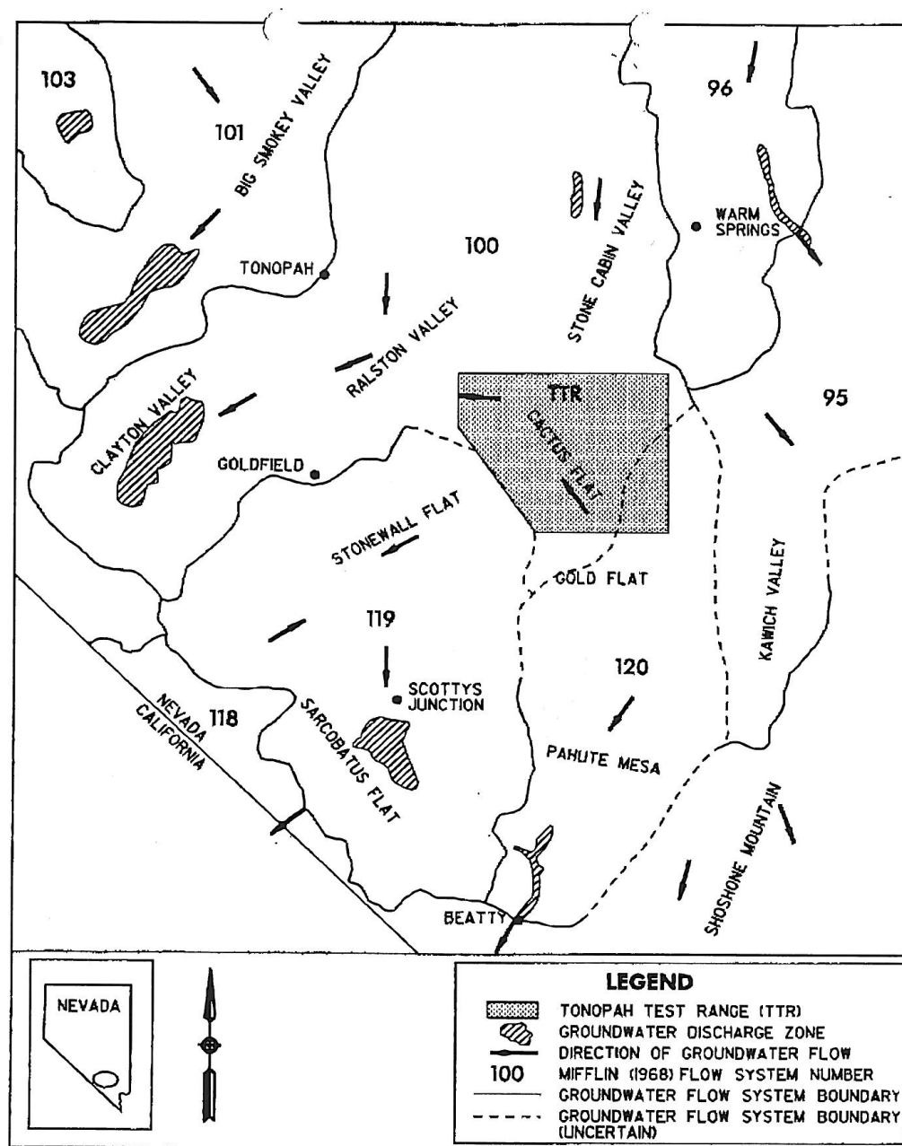
Figure 2. Groundwater Flow Systems near TTR
